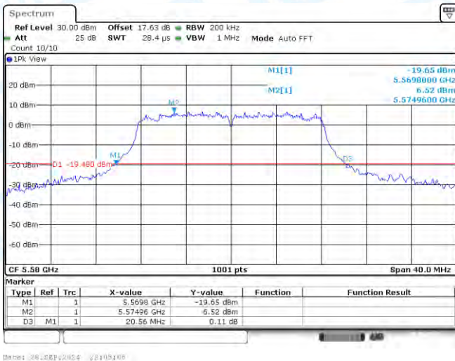
11A-Ant2-5580
