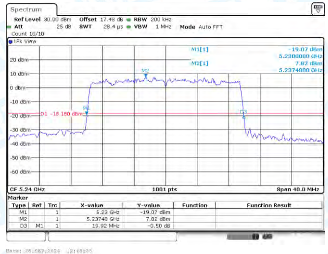
11AX20-CDD-Ant1-5240
