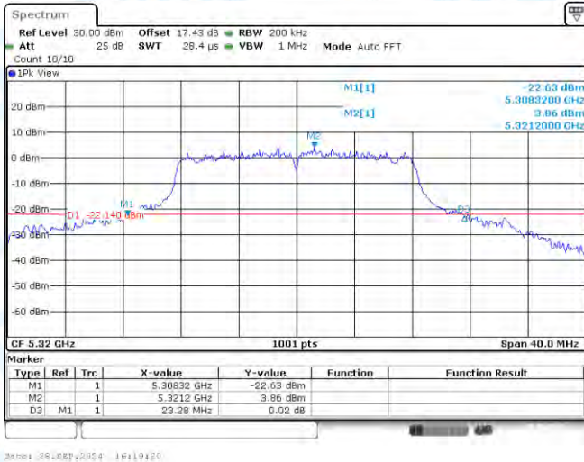
11A-CDD-Ant1-5320
