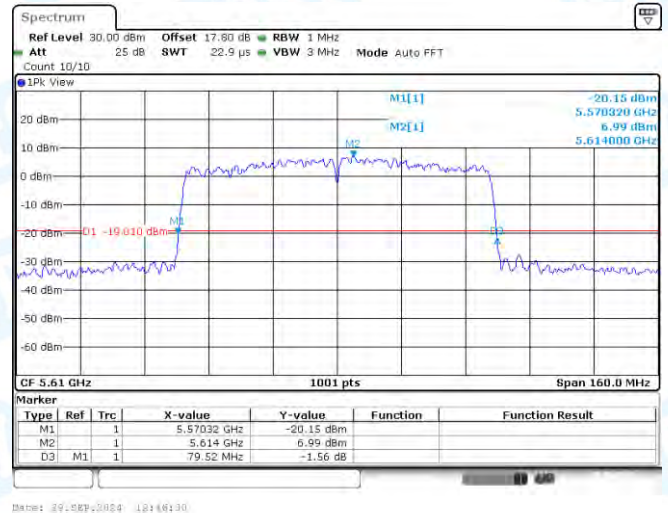
11AC80-CDD-Ant3-5610
