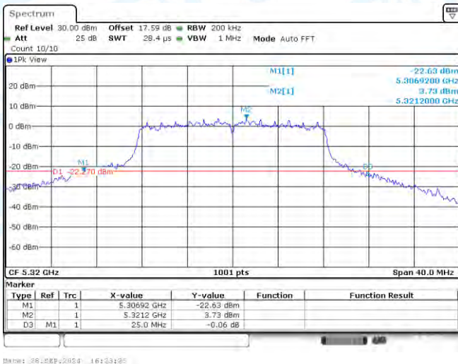
11A-CDD-Ant3-5320
