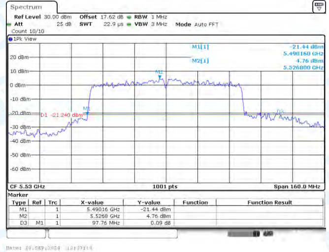
11AC80-CDD-Ant2-5530
