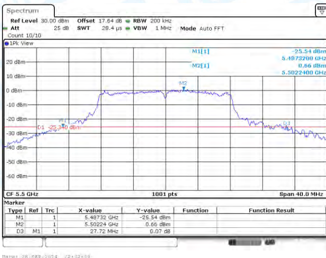
11A-CDD-Ant2-5500
