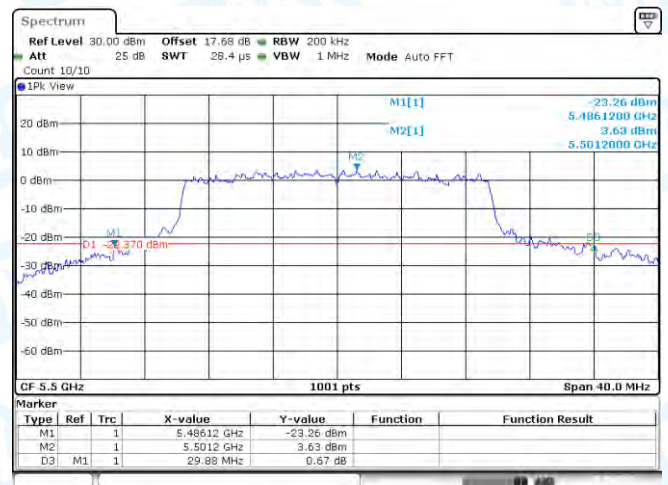
11AX20-CDD-Ant1-5500
