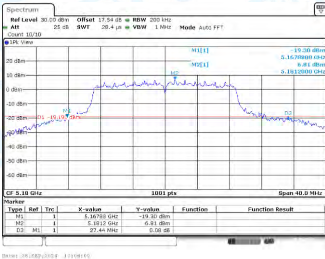
11AC20-CDD-Ant3-5180
