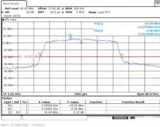
11N40-CDD-Ant1-5550
