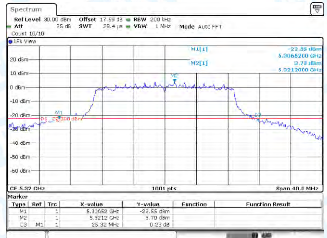
11AC20-CDD-Ant1-5320
