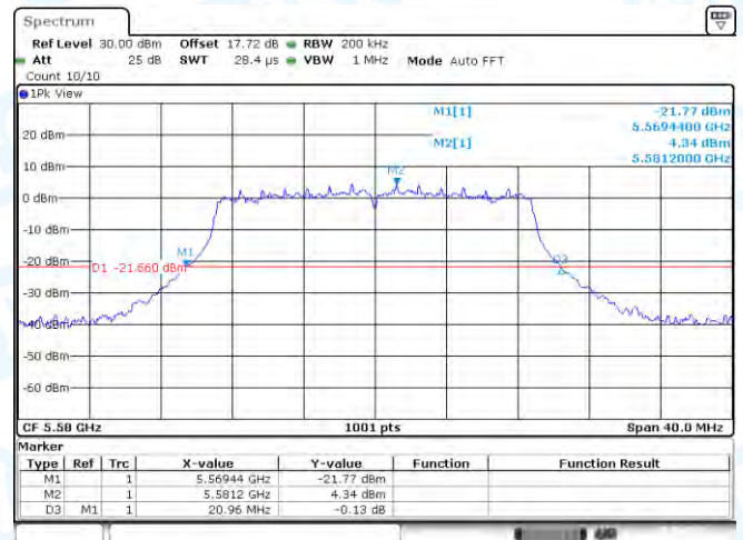
11AC20-CDD-Ant1-5580
