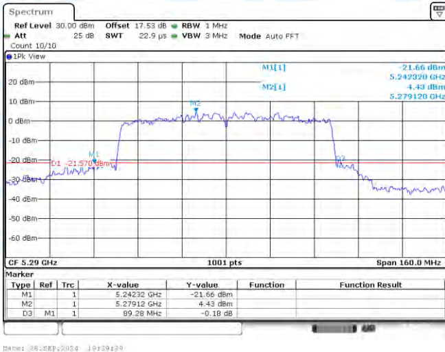
11AC80-CDD-Ant2-5290
