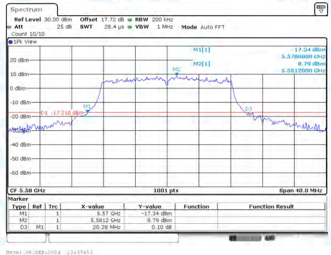
11A-Ant3-5580
