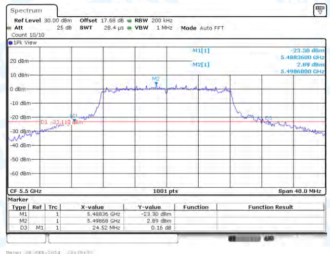
11A-CDD-Ant3-5500
