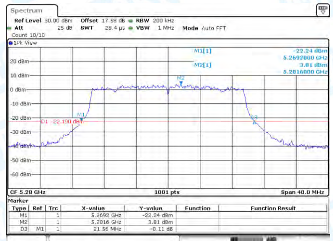
11AX20-CDD-Ant1-5280
