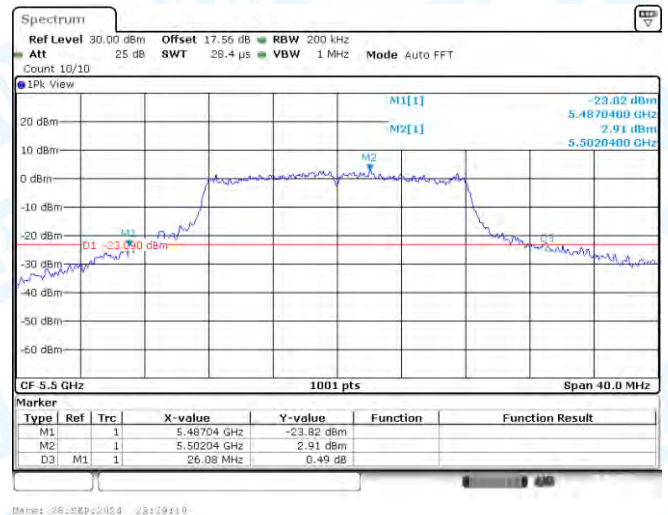
11A-CDD-Ant1-5500
