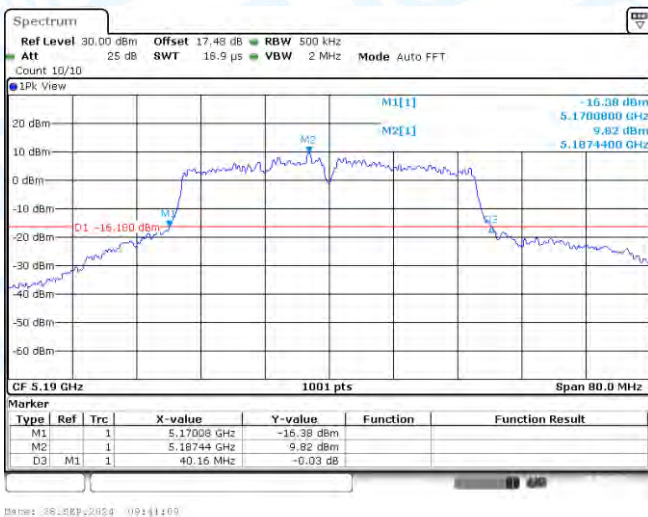
11N40-CDD-Ant2-5190
