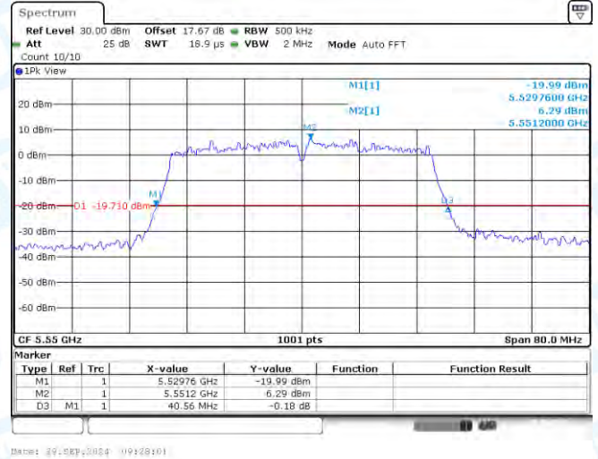
11N40-CDD-Ant2-5550
