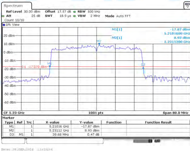
11AX40-CDD-Ant2-5230
