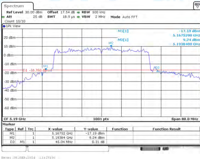
11AX40-CDD-Ant3-5190
