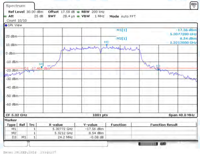
11A-Ant3-5320
