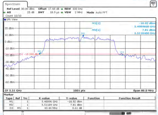
11N40-CDD-Ant1-5510
