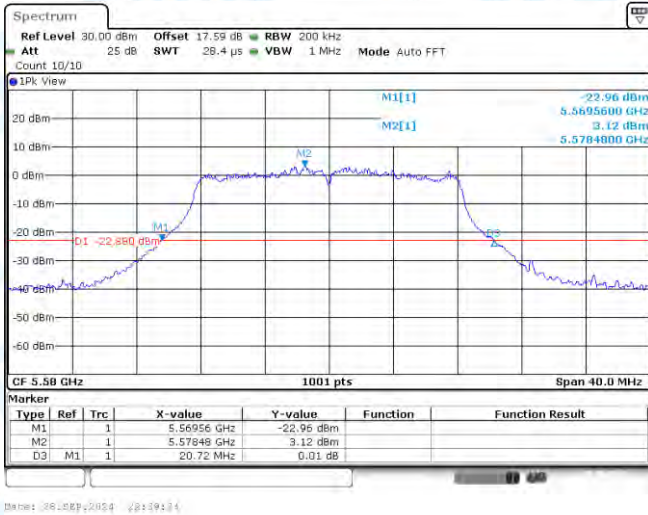
11A-CDD-Ant1-5580
