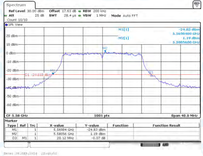
11A-CDD-Ant2-5580
