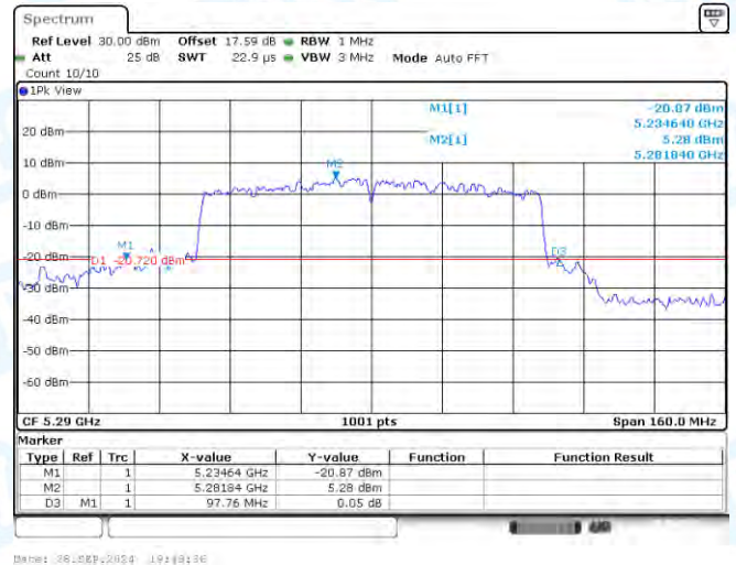
11AC80-CDD-Ant3-5290
