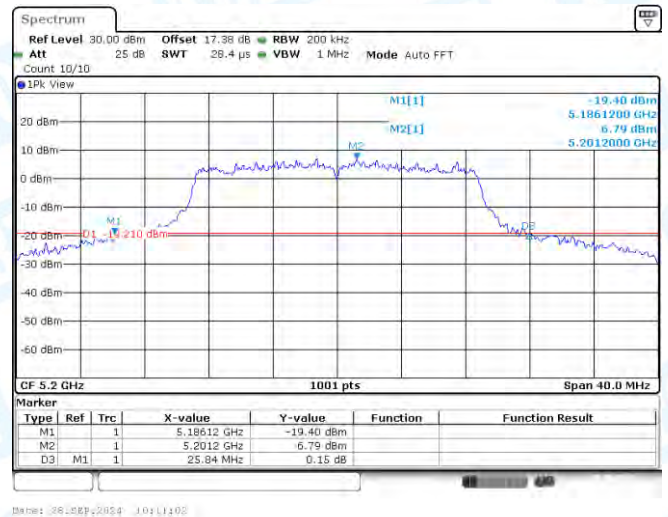
11AC20-CDD-Ant1-5200
