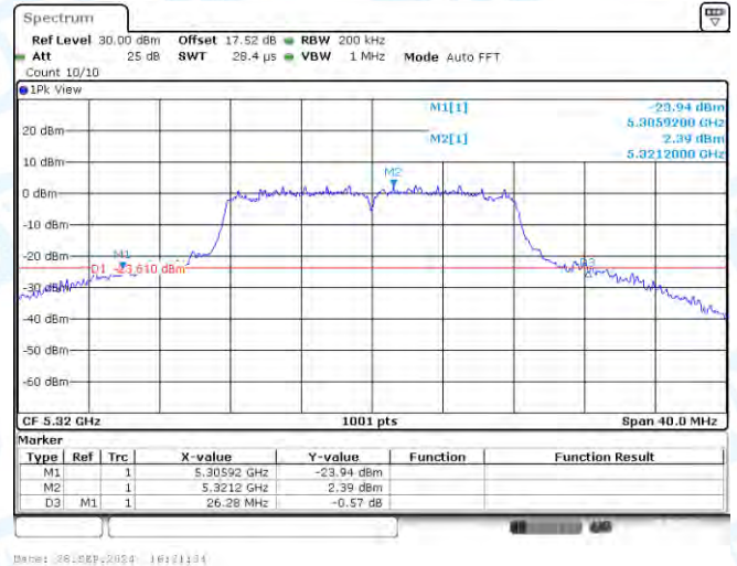
11A-CDD-Ant2-5320
