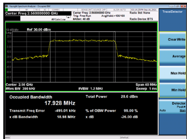
NR n7 64QAM 100%RB CH-High
