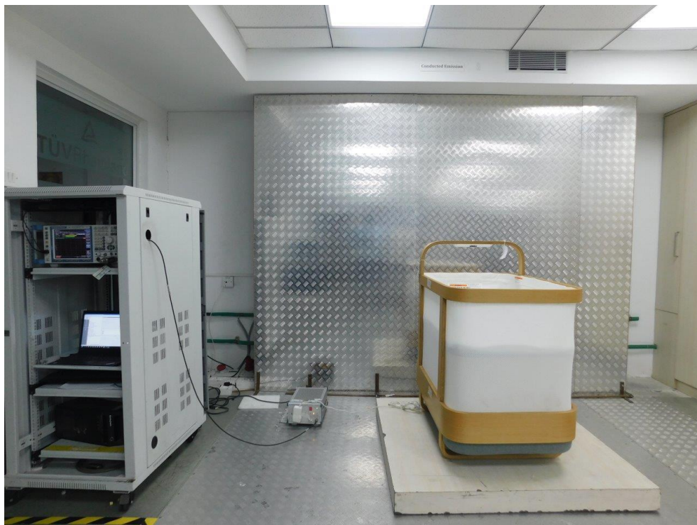
Conducted AC Powerline Test Setup
