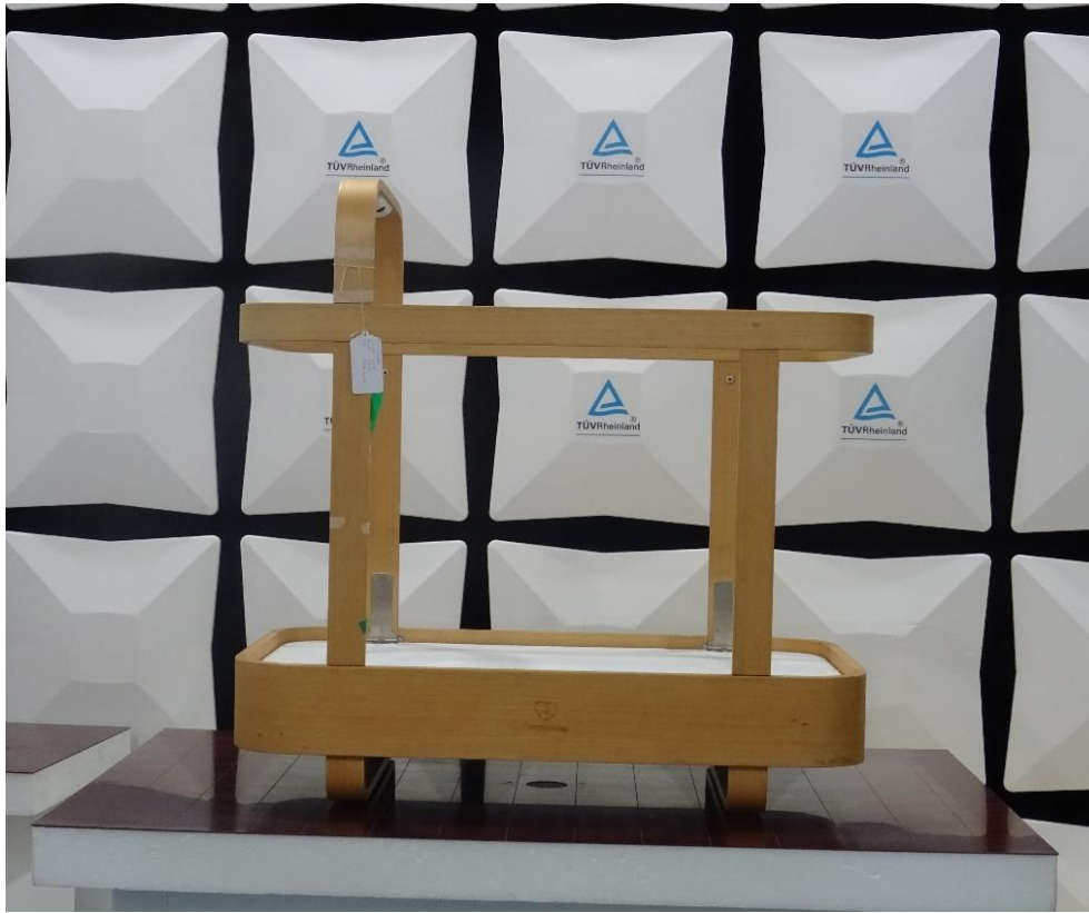
Closeup view of EUT
