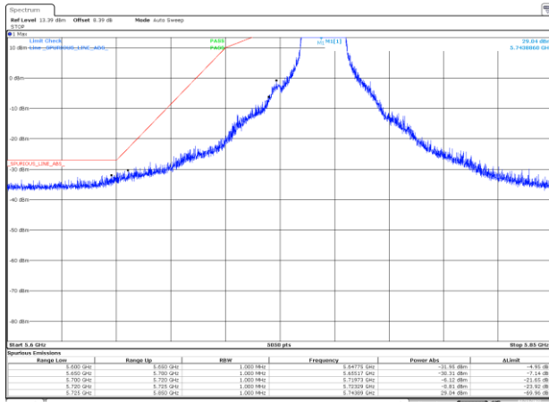
BE-NR-LOW, MIMO-B, 802.11ax20-HE0, Ch149
