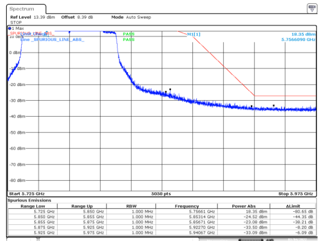
BE-NR-HIGH, MIMO-B, 802.11n40-HT0, Ch151
