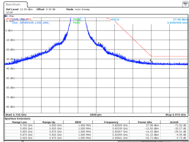
BE-NR-HIGH, MIMO-B, 802.11n20-HT0, Ch165
