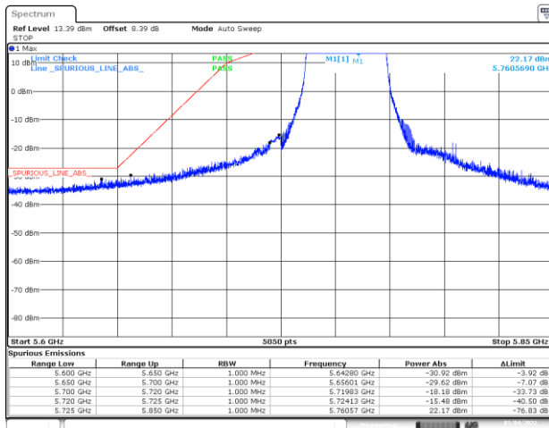
BE-NR-LOW, MIMO-B, 802.11n40-HT0, Ch151
