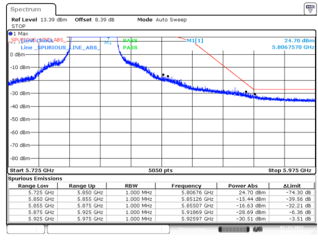
BE-NR-HIGH, MIMO-B, 802.11n40-HT0, Ch159
