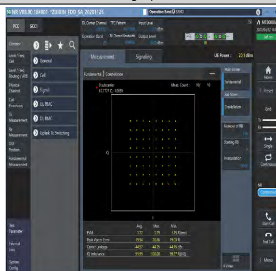
1-N25--15-40-M-4-DFT-64QAM-Outter_Full-216@0-A Ant1-see graph-PASS
