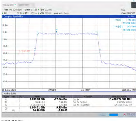
1-N25--15-15-H-5-DFT-256QAM-Outer_Full-75@0-A nt1-13.429-14.460-≤15-PASS
