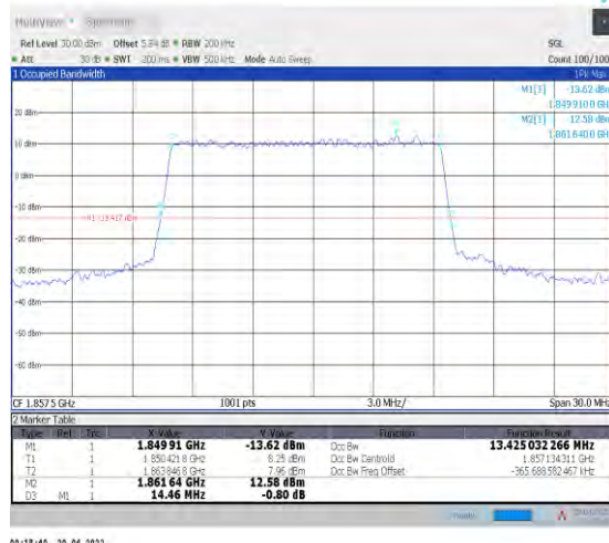
1-N25--15-15-L-4-DFT-64QAM-Outer_Full-75@0-Ant 1-13.425-14.460-≤15-PASS
