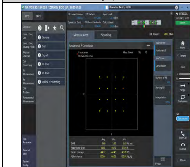
1-N25--15-40-M-3-DFT-16QAM-Outter_Full-216@0-A nt1-see graph-PASS
