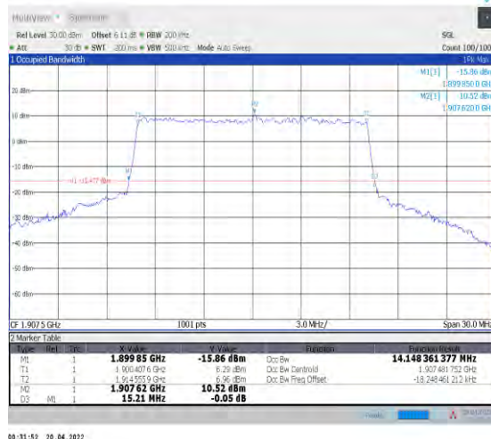
1-N25--15-15-H-8-CP-64QAM-Outer_Full-79@0-Ant 1-14.148-15.210-≤15-PASS
