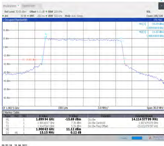
1-N25--15-15-H-7-CP-16QAM-Outer_Full-79@0-Ant 1-14.115-15.150-≤15-PASS
