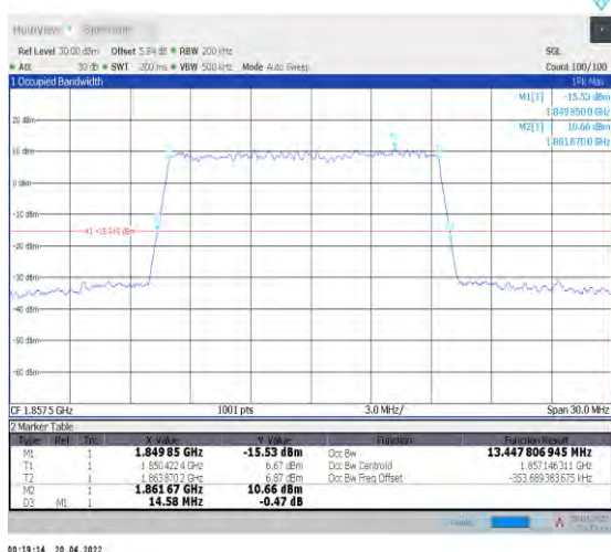
1-N25--15-15-L-5-DFT-256QAM-Outer_Full-75@0-A nt1-13.448-14.580-≤15-PASS
