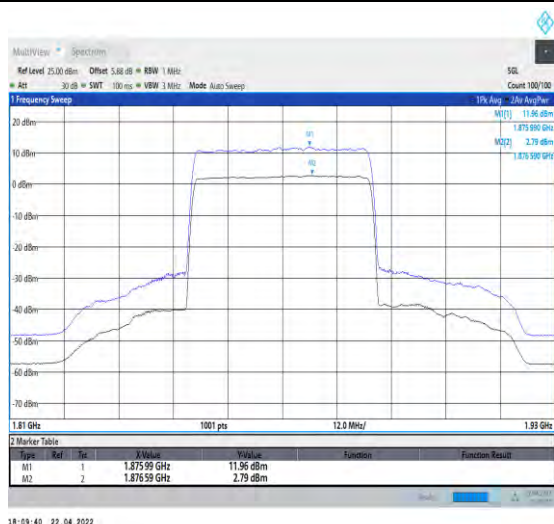
1-N25--15-40-L-1-DFT-256QAM-Outer_Full-216@0-Ant1-9.17-100%-0.00-9.17-PASS-≤13
