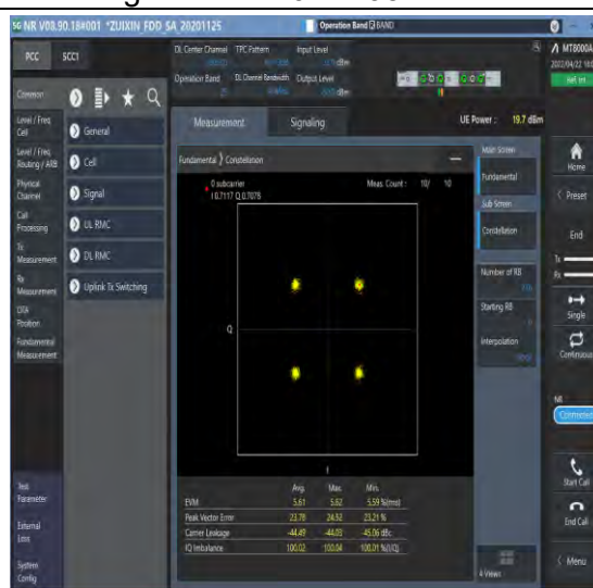
1-N25--15-40-M-6-CP-QPSK-Outer_Full-216@0-Ant1-see graph-PASS
