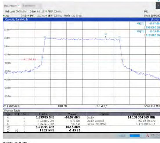
1-N25--15-15-H-6-CP-QPSK-Outer_Full-79@0-Ant1 14.131-15.270-≤15-PASS
