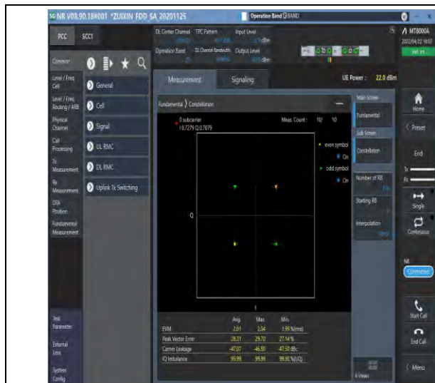
1-N25--15-40-M-1-DFT-PI2BPSK-Outter_Full-216@0-A Ant1-see graph-PASS
