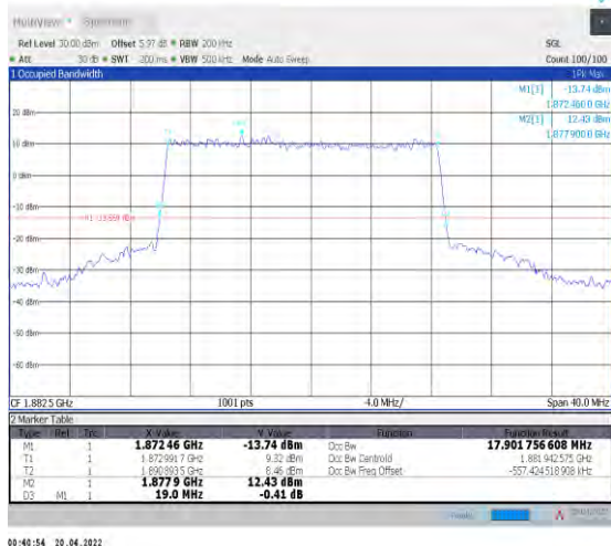
1-N25--15-20-M-3-DFT-16QAM-Outer_Full-100@0-A nt1-17.902-19.000-≤20-PASS
