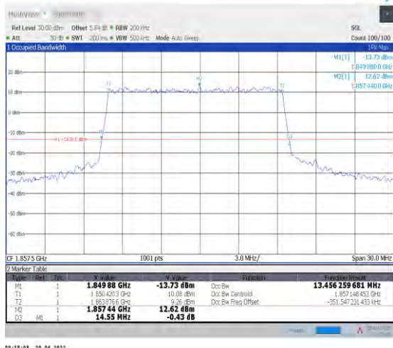
1-N25--15-15-L-3-DFT-16QAM-Outer_Full-75@0-Ant 1-13.456-14.550-≤15-PASS
