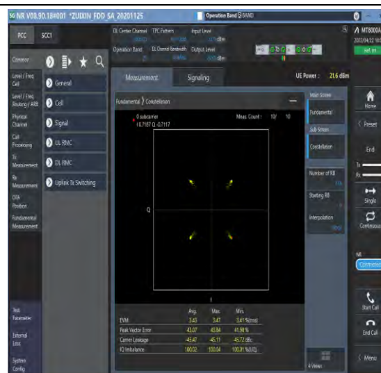
1-N25--15-40-M-2-DFT-QPSK-Outter_Full-216@0-A nt1-see graph-PASS
