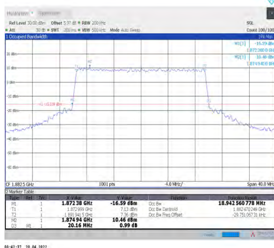
1-N25--15-20-M-6-CP-QPSK-Outer_Full-106@0-Ant 1-18.943-20.160-≤20-PASS
