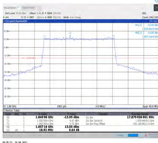
1-N25--15-20-L-3-DFT-16QAM-Outer_Full-100@0-A nt1-17.879-18.920-≤20-PASS
