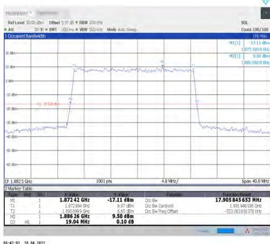
1-N25--15-20-M-5-DFT-256QAM-Outer_Full-100@0-A Ant1-17.906-19.040-≤20-PASS
