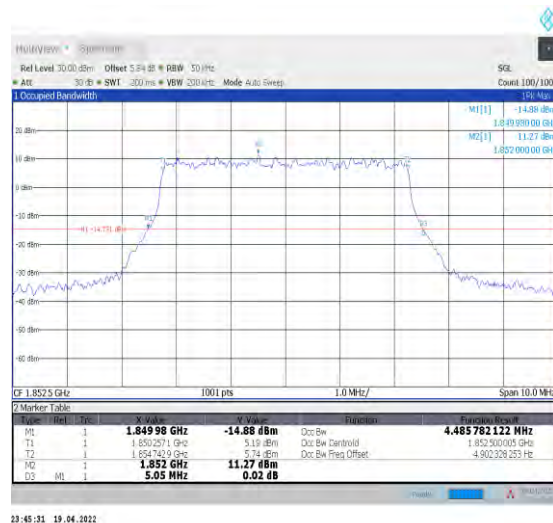
1-N25--15-5-L-4-DFT-64QAM-Outer_Full-25@0-Ant1-4.486-5.050-≤5-PASS
