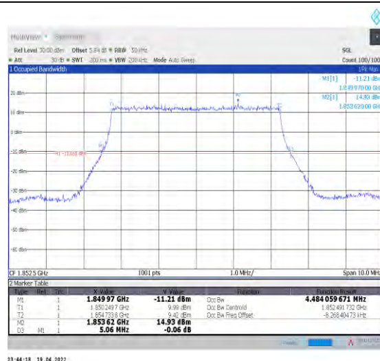
1-N25--15-5-L-2-DFT-PI2BPSK-Outer_Full-25@0-An t1-4.484-5.060-≤5-PASS
