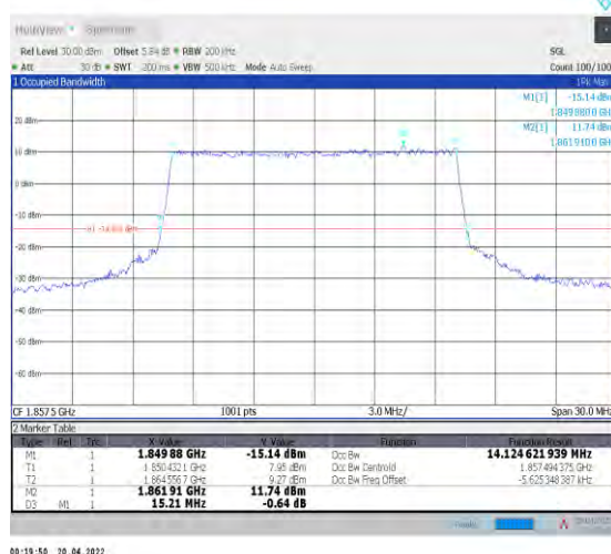
1-N25--15-15-L-6-CP-QPSK-Outer_Full-79@0-Ant1 14.125-15.210-≤15-PASS
