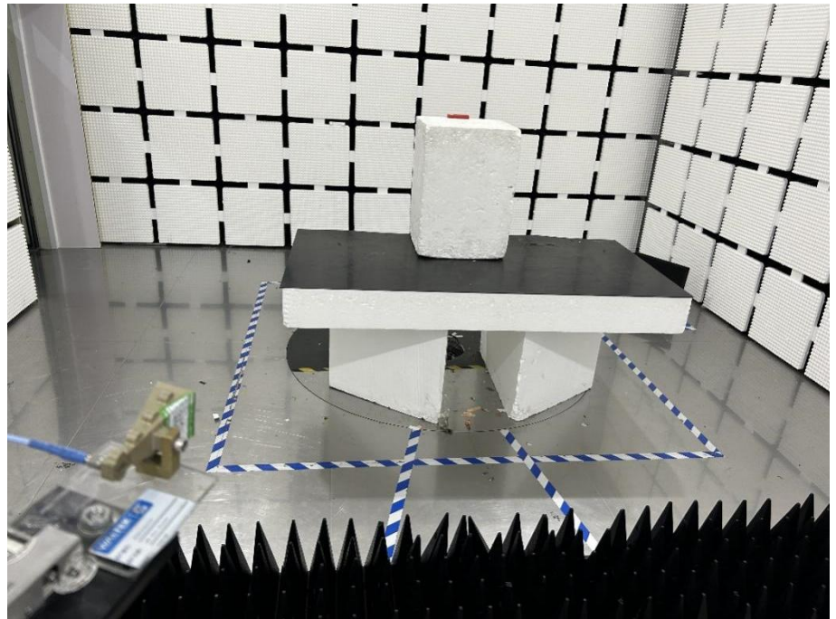
Radiation Emission Test Setup (Above 18GHz)
