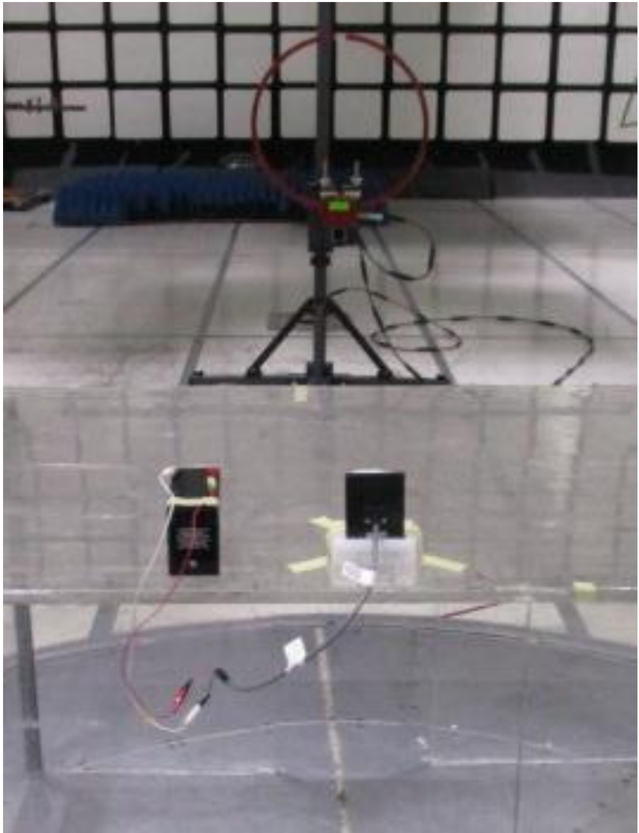
Radiated Emissions Below 30MHz
