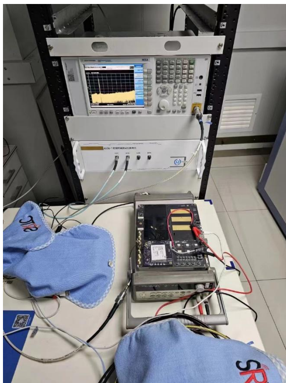
RF Conducted Test setup (BT/WIFI)
