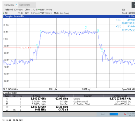
1-N78-3450-3550--30-10-H-4-DFT-64QAM-Outer_Fu ll-24@0-Ant0-8.57-9.680-≤10-PASS
