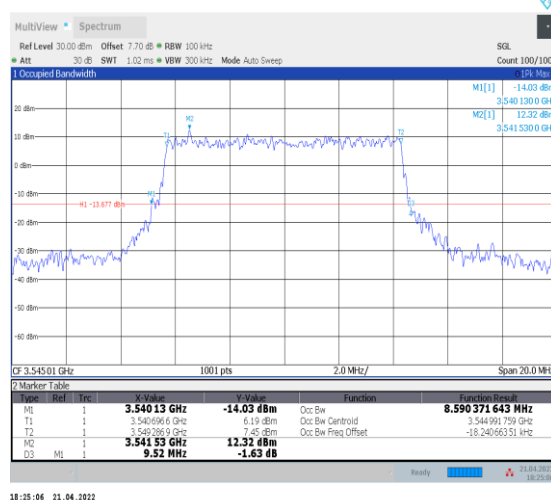
1-N78-3450-3550--30-10-H-6-CP-QPSK-Outer_Full- 24@0-Ant0-8.59-9.520-≤10-PASS
