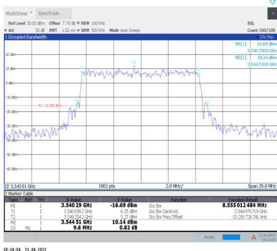
1-N78-3450-3550--30-10-H-5-DFT-256QAM-Outer_F ull-24@0-Ant0-8.555-9.600-≤10-PASS
