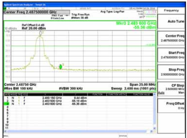
Band Edge_8DPSK_3M_DH5_2480MHz
