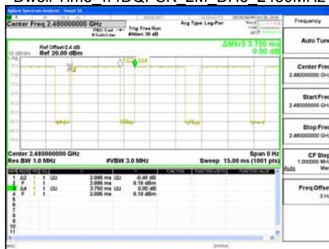
Dwell Time \pi 4DQPSK 2M DH5 2480MHz
