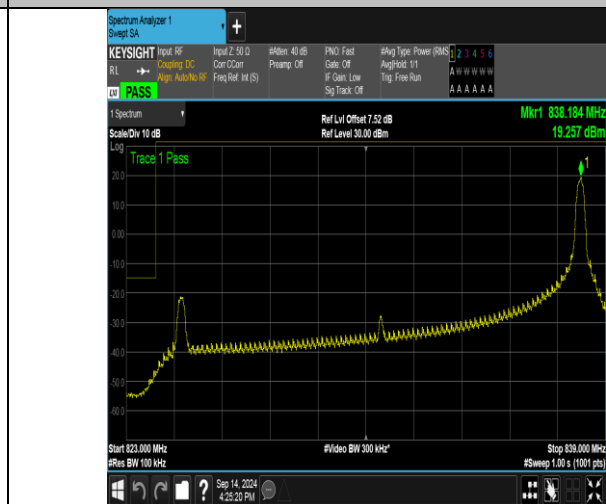
Band26_15MHz_16QAM_26865_1RB#74
