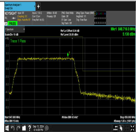
Band26_1.4MHz_16QAM_27033_6RB#0
