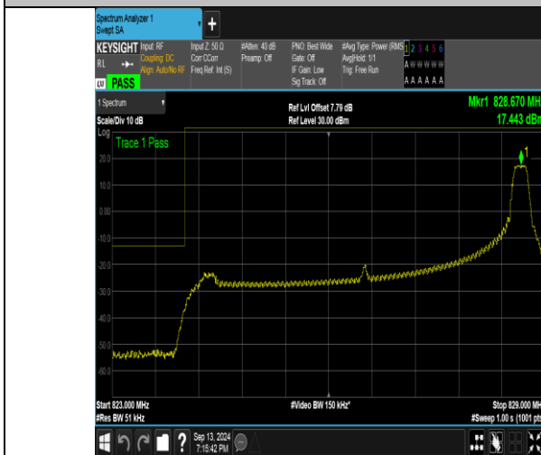
Band26_5MHz_QPSK_26815_1RB#24
