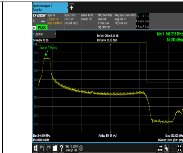
Band26_3MHz_16QAM_27025_1RB#0
