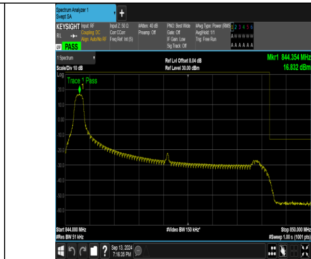
Band26_5MHz_16QAM_27015_1RB#0
