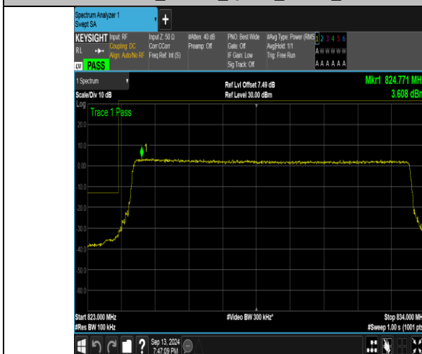
Band26_10MHz_QPSK_26840_50RB#0
