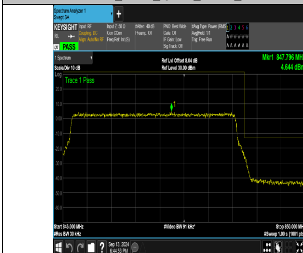
Band26_3MHz_QPSK_27025_15RB#0
