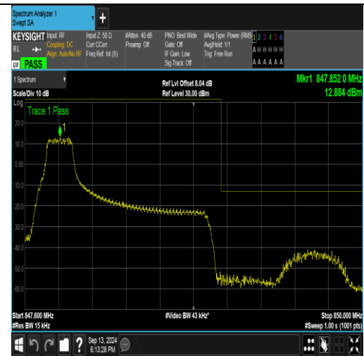
Band26_1.4MHz_16QAM_27033_1RB#0
