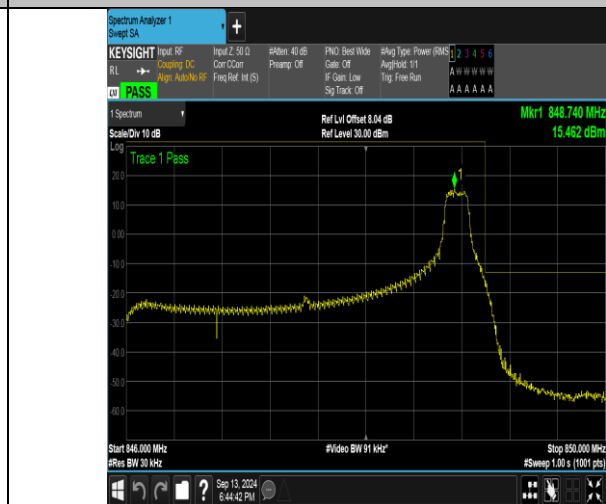
Band26_3MHz_16QAM_27025_1RB#14
