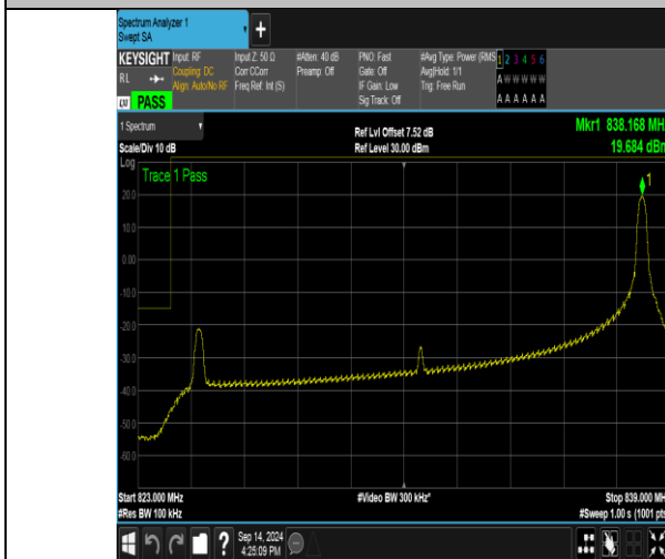
Band26_15MHz_QPSK_26865_1RB#74
