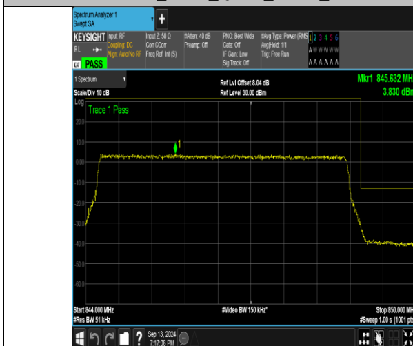
Band26_5MHz_QPSK_27015_25RB#0
