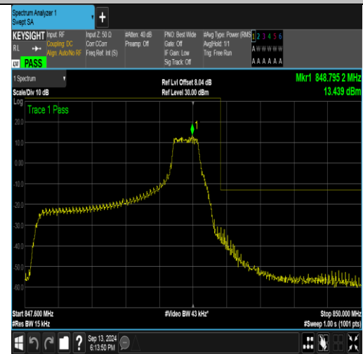
Band26_1.4MHz_16QAM_27033_1RB#5
