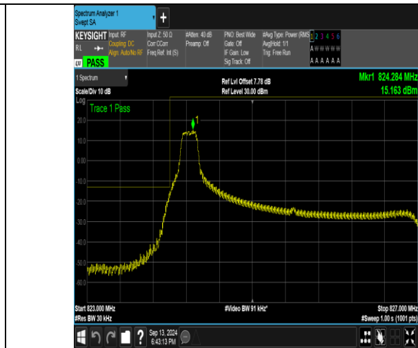
Band26_3MHz_16QAM_26805_1RB#0
