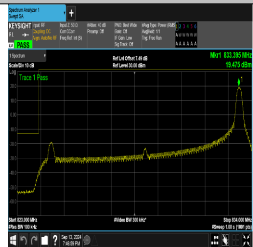
Band26_10MHz_16QAM_26840_1RB#49
