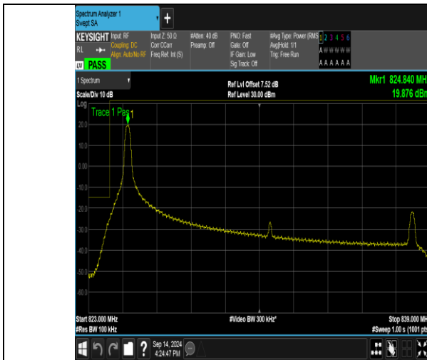
Band26_15MHz_QPSK_26865_1RB#0
