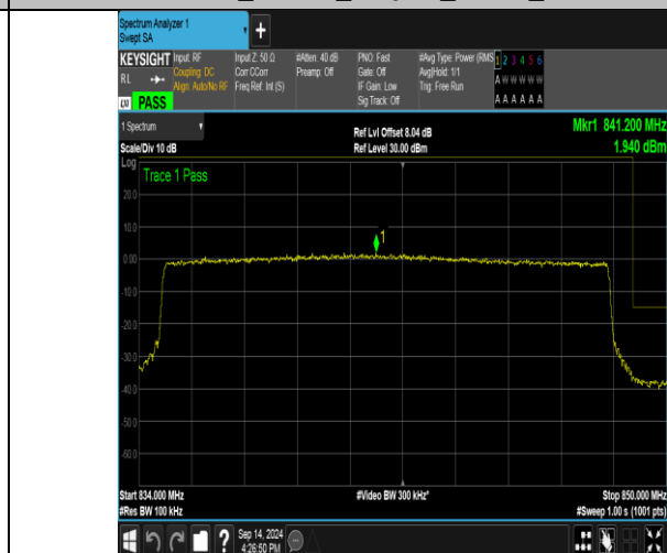
Band26_15MHz_16QAM_26965_75RB#0
