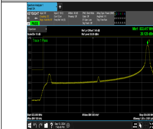
Band26_10MHz_QPSK_26840_1RB#49
