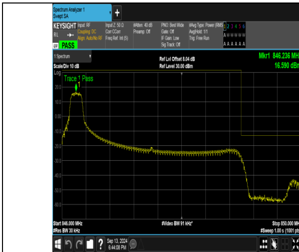
Band26_3MHz_QPSK_27025_1RB#0
