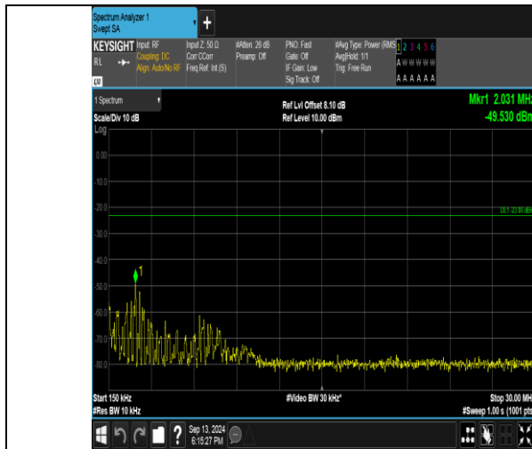
Band26_1.4MHz_16QAM_26797_1RB#0_0.15~30_0.15~30
