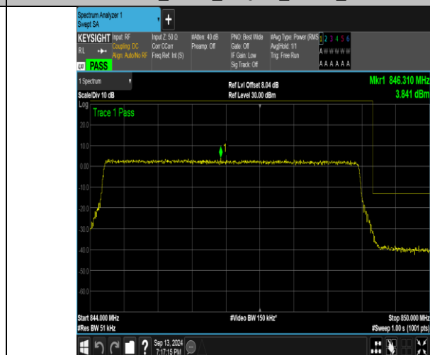
Band26_5MHz_16QAM_27015_25RB#0
