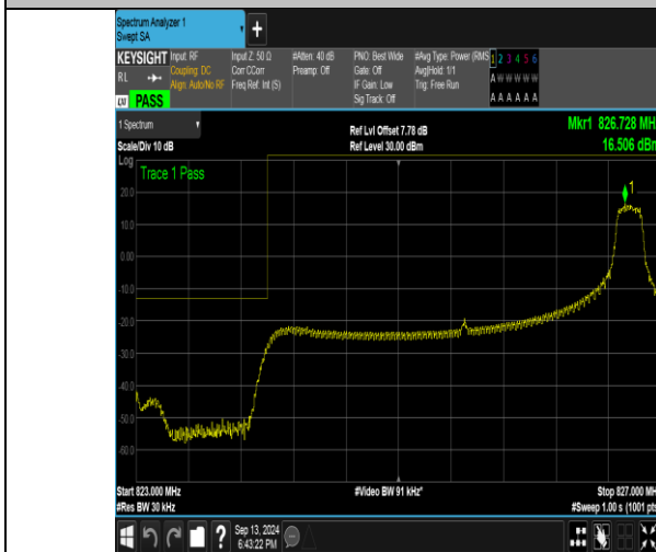
Band26_3MHz_QPSK_26805_1RB#14
