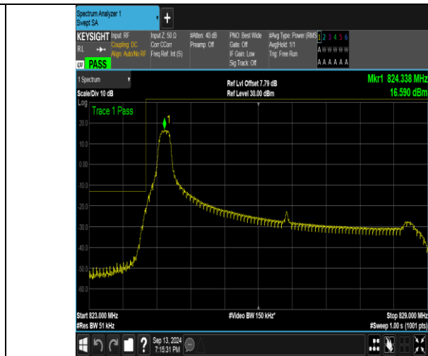
Band26_5MHz_16QAM_26815_1RB#0
