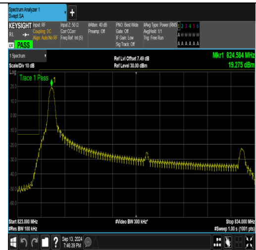
Band26_10MHz_16QAM_26840_1RB#0
