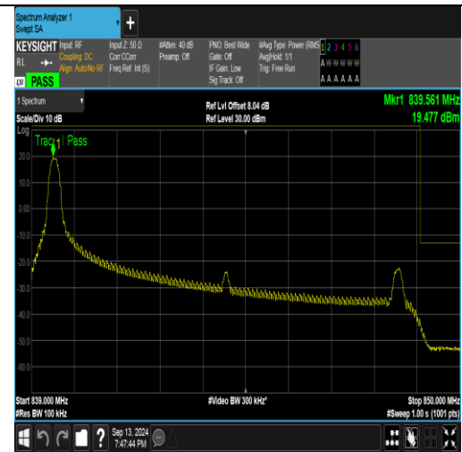
Band26_10MHz_16QAM_26990_1RB#0
