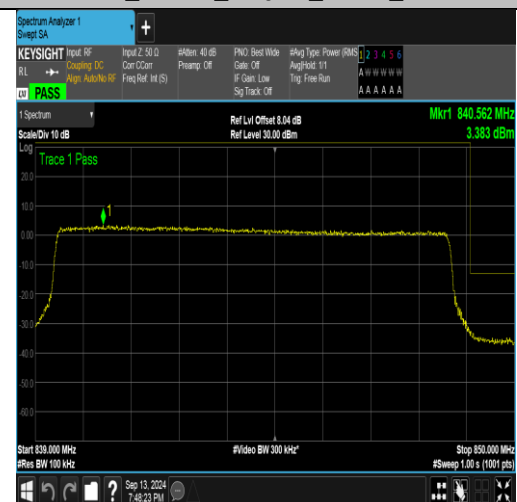
Band26_10MHz_16QAM_26990_50RB#0
