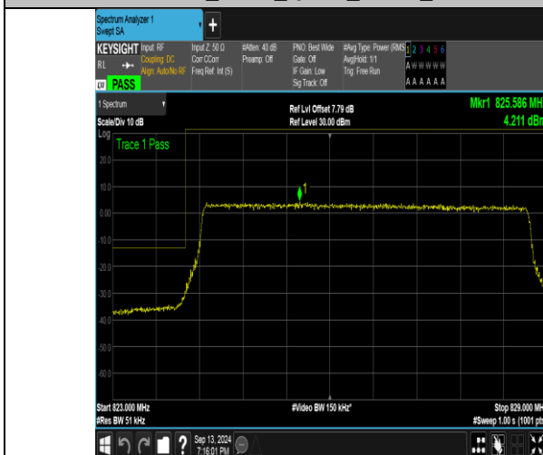
Band26_5MHz_QPSK_26815_25RB#0
