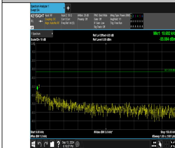
Band26_1.4MHz_QPSK_26797_1RB#5_0.009~0.15_0.009~0.15
