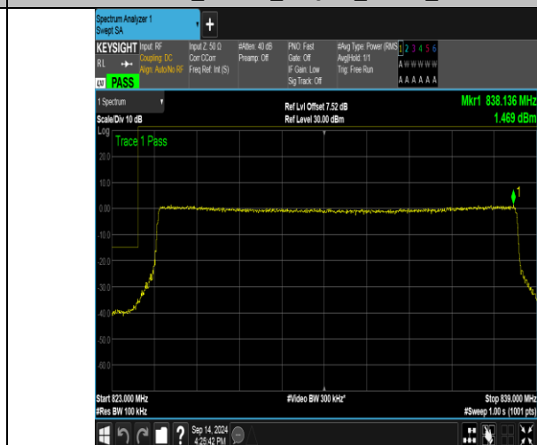
Band26_15MHz_16QAM_26865_75RB#0
