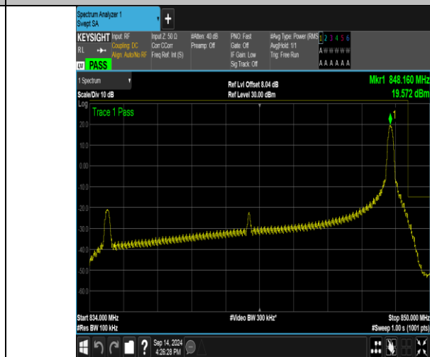
Band26_15MHz_16QAM_26965_1RB#74
