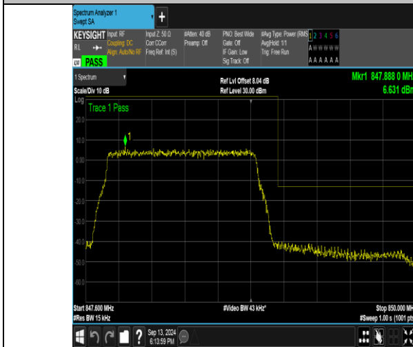
Band26_1.4MHz_QPSK_27033_6RB#0
