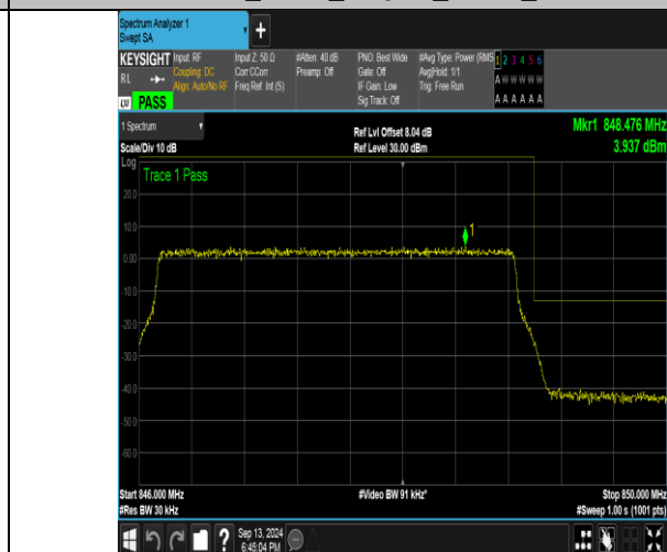
Band26_3MHz_16QAM_27025_15RB#0
