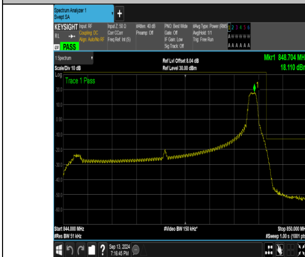
Band26_5MHz_QPSK_27015_1RB#24
