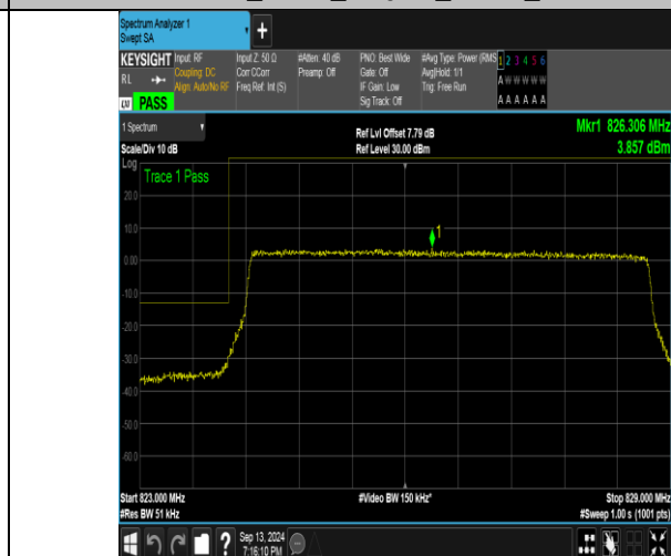
Band26_5MHz_16QAM_26815_25RB#0
