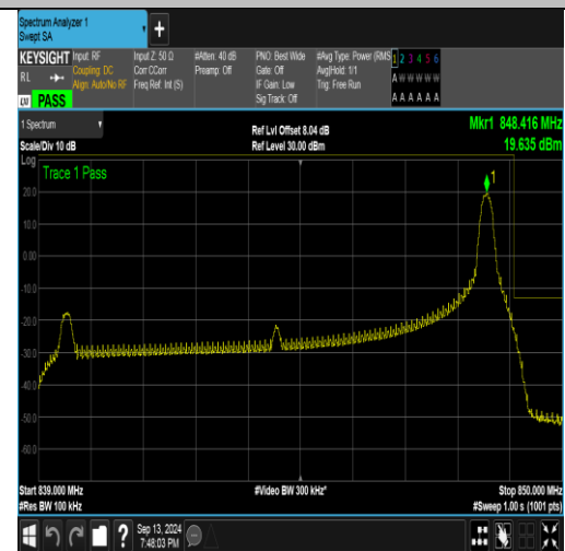
Band26_10MHz_16QAM_26990_1RB#49
