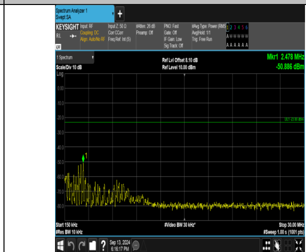
Band26_1.4MHz_QPSK_26797_1RB#5_0.15~30_0.15~30
