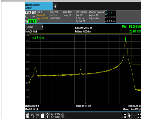
Band26_10MHz_QPSK_26990_1RB#49
