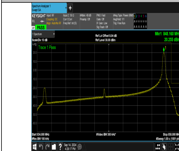
Band26_15MHz_QPSK_26965_1RB#74
