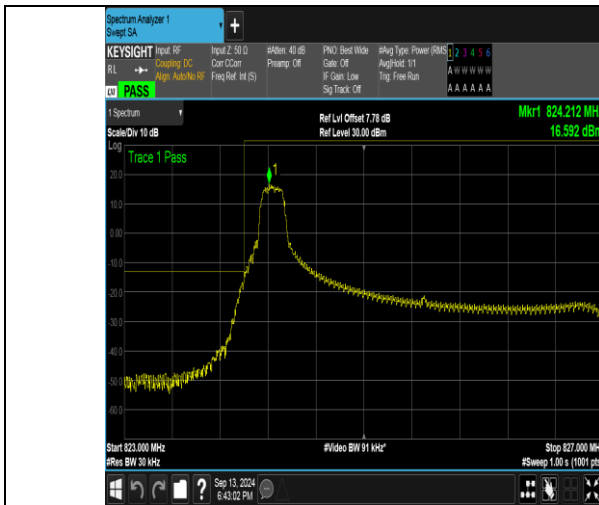
Band26_3MHz_QPSK_26805_1RB#0
