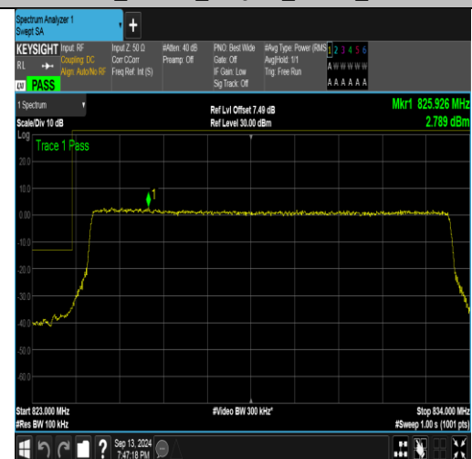
Band26_10MHz_16QAM_26840_50RB#0
