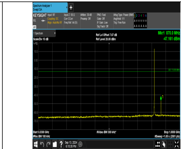
Band26_1.4MHz_16QAM_26797_1RB#0_30~1000_30~1000
