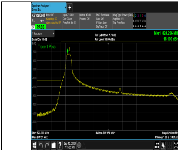
Band26_5MHz_QPSK_26815_1RB#0
