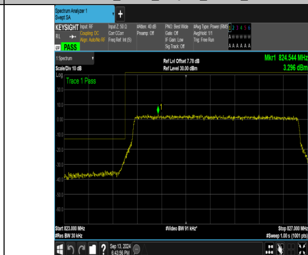
Band26_3MHz_16QAM_26805_15RB#0
