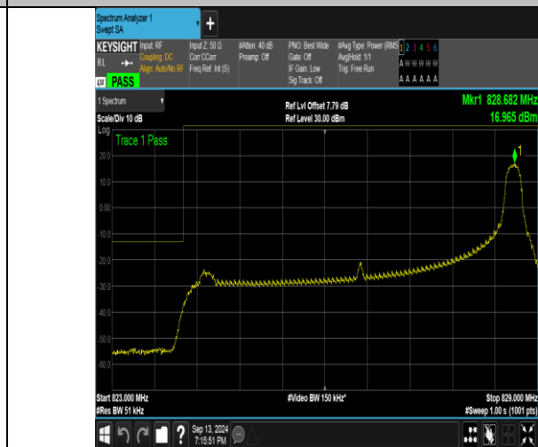
Band26_5MHz_16QAM_26815_1RB#24
