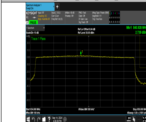
Band26_15MHz_QPSK_26965_75RB#0
