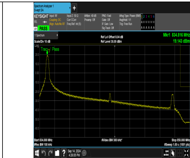
Band26_15MHz_16QAM_26965_1RB#0
