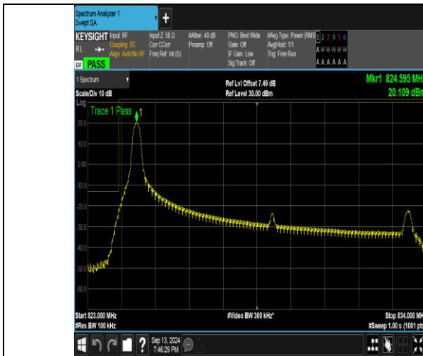
Band26_10MHz_QPSK_26840_1RB#0
