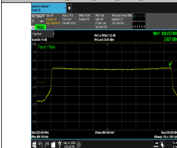
Band26_15MHz_QPSK_26865_75RB#0
