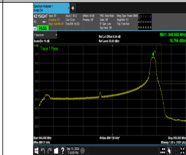
Band26_5MHz_16QAM_27015_1RB#24
