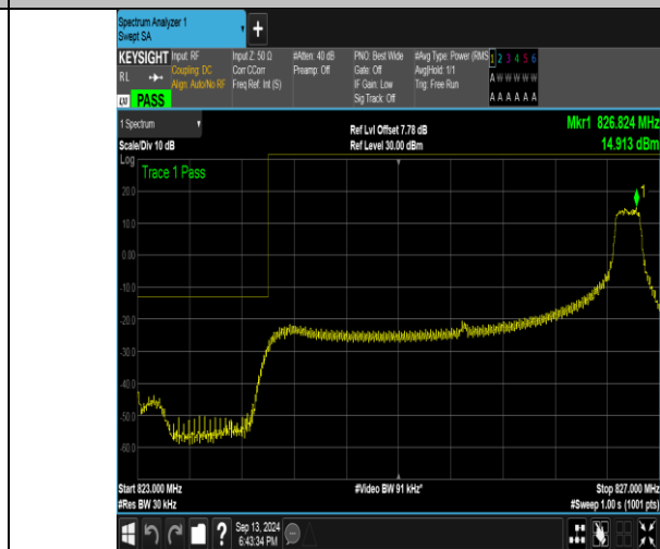
Band26_3MHz_16QAM_26805_1RB#14
