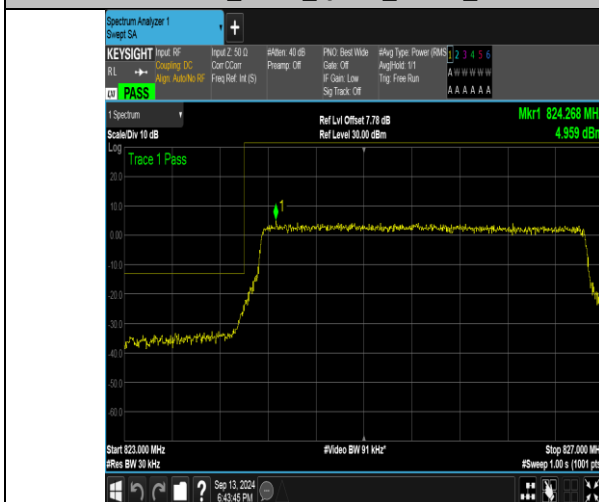
Band26_3MHz_QPSK_26805_15RB#0
