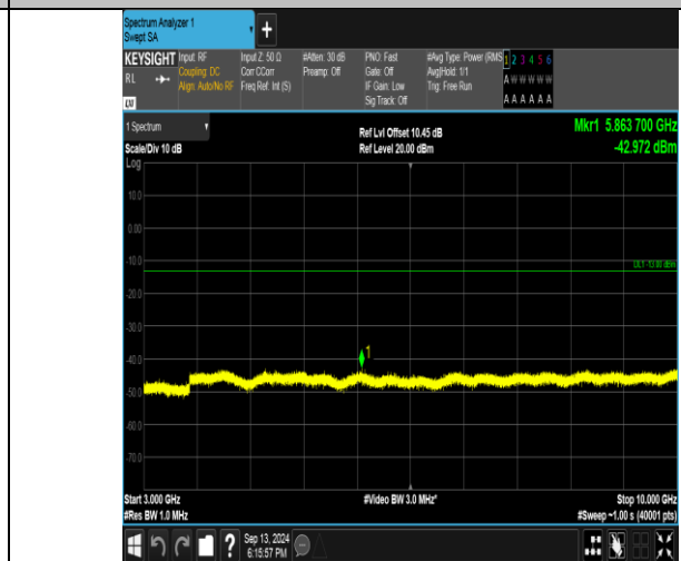
Band26_1.4MHz_16QAM_26797_1RB#0_3000~10000_3000~10000
