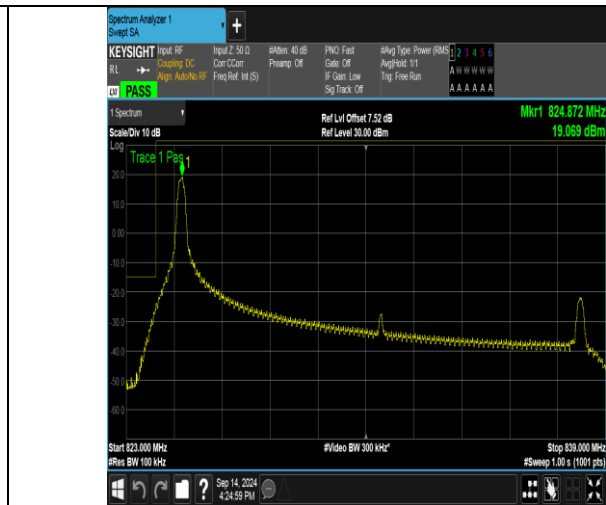
Band26_15MHz_16QAM_26865_1RB#0
