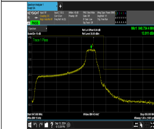
Band26_1.4MHz_QPSK_27033_1RB#5
