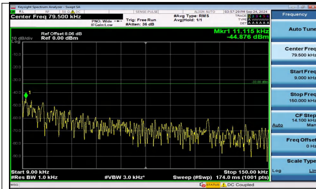
Band5_5MHz_QPSK_20425_1RB#0_0.009~0.15_0.009~0.15
