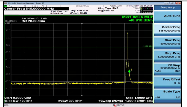
Band5_5MHz_16QAM_20425_25RB#0_30~1000_30~100 0
