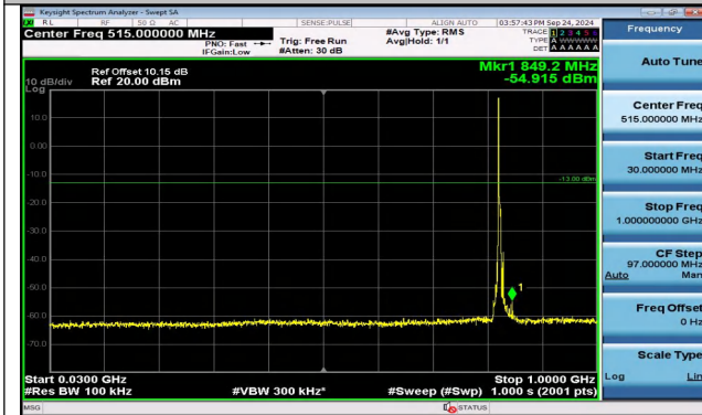
Band5_5MHz_QPSK_20425_1RB#0_30~1000_30~1000
