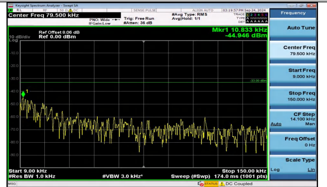
Band5_3MHz_16QAM_20635_15RB#0_0.009~0.15_0.009~0.15
