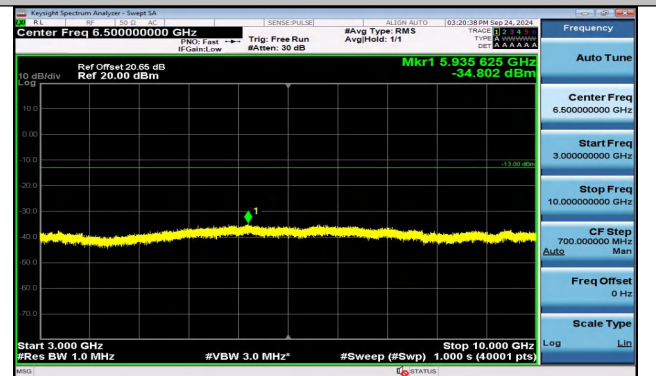
Band5_3MHz_16QAM_20635_15RB#0_3000~10000_3000~10000
