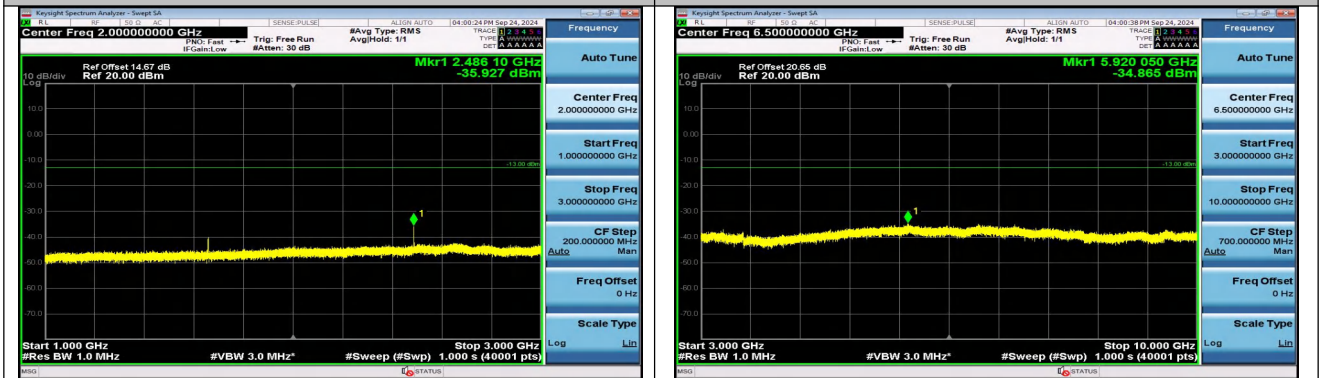
Band5_5MHz_16QAM_20425_1RB#24_1000~3000_1000 ~3000
