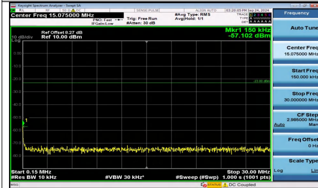
Band5_3MHz_16QAM_20635_15RB#0_0.15~30_0.15~30
