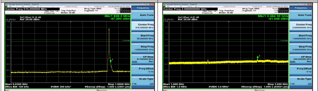
Band5_5MHz_QPSK_20425_25RB#0_1000~3000_1000~3 000
