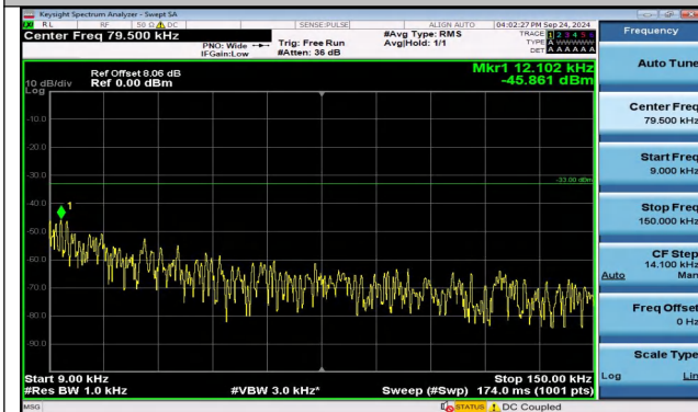
Band5_5MHz_QPSK_20525_1RB#0_0.009~0.15_0.009~0.15
