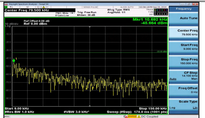
Band5_5MHz_16QAM_20425_1RB#0_0.009~0.15_0.009~0.15
