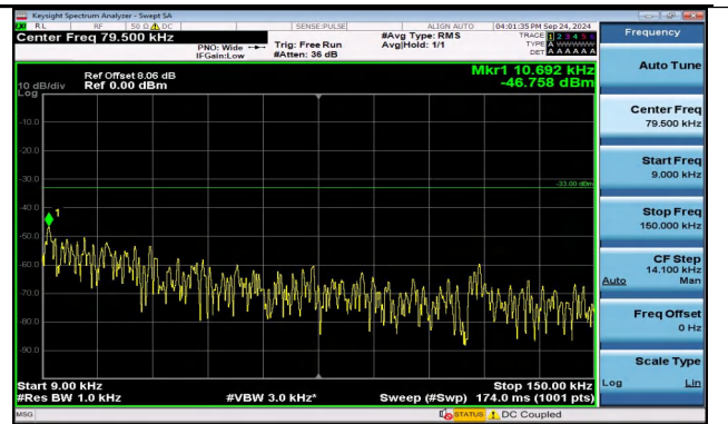
Band5_5MHz_16QAM_20425_25RB#0_0.009~0.15_0.009 ~0.15
