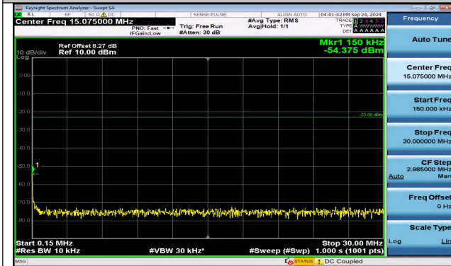
Band5_5MHz_16QAM_20425_25RB#0_0.15~30_0.15~3 0
