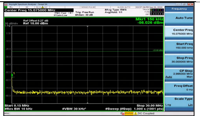
Band5_5MHz_QPSK_20425_1RB#0_0.15~30_0.15~30
