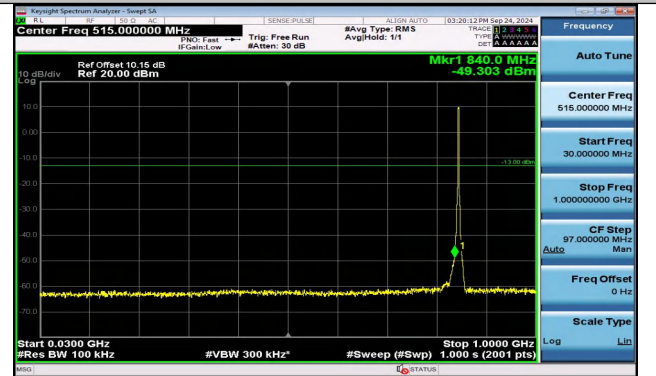
Band5_3MHz_16QAM_20635_15RB#0_30~1000_30~1000
