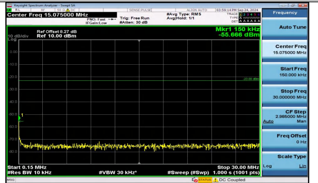
Band5_5MHz_QPSK_20425_1RB#24_0.15~30_0.15~30
