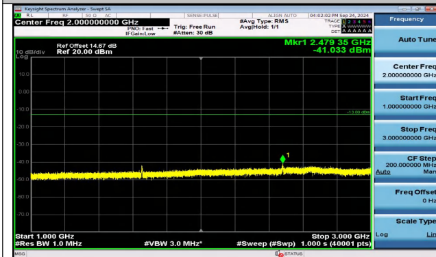
Band5_5MHz_16QAM_20425_25RB#0_1000~3000_1000 ~3000
