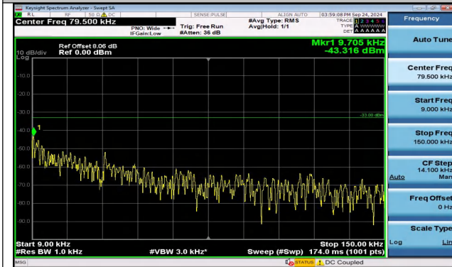
Band5_5MHz_QPSK_20425_1RB#24_0.009~0.15_0.009 ~0.15
