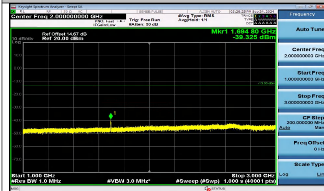
Band5_3MHz_16QAM_20635_15RB#0_1000~3000_1000~3000
