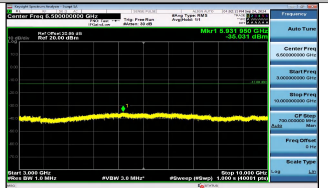
Band5_5MHz_16QAM_20425_25RB#0_3000~10000_3000 ~10000
