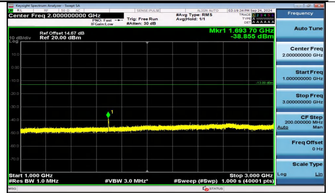
Band5_3MHz_QPSK_20635_15RB#0_1000~3000_1000~3000
