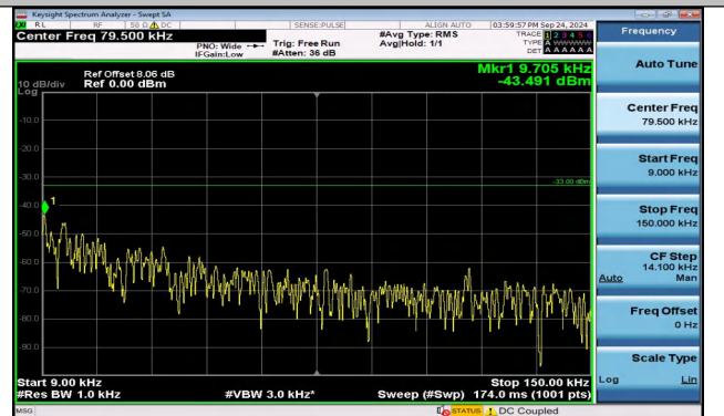
Band5_5MHz_16QAM_20425_1RB#24_0.009~0.15_0.009 ~0.15
