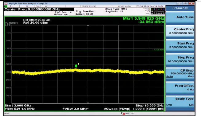
Band5_5MHz_16QAM_20425_1RB#0_3000~10000_3000 ~10000
