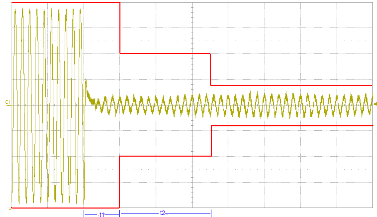
473MHz On to Off
