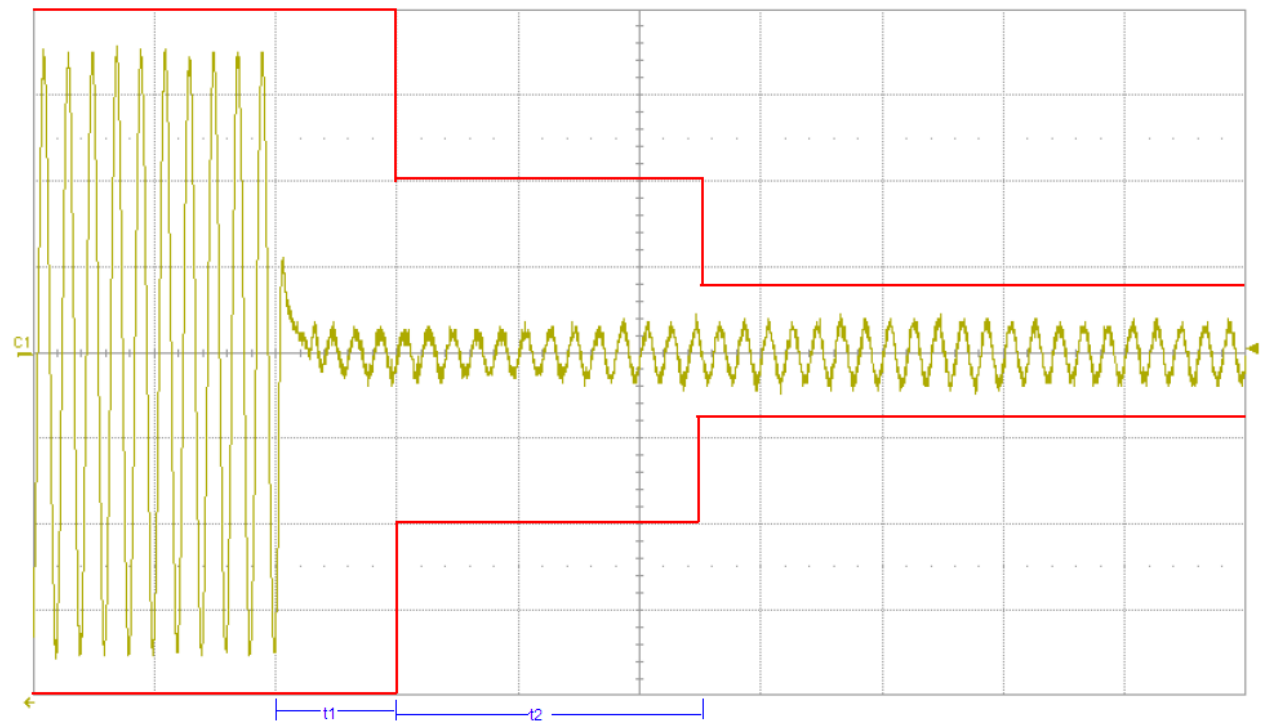
450MHz On to Off
