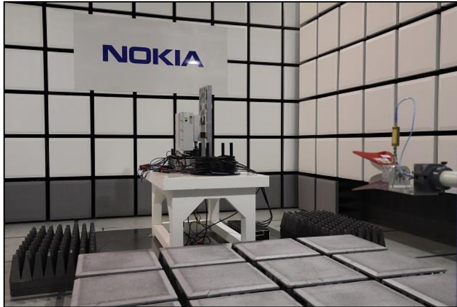
Figure 3 - Radiated Emissions (6 GHz to 18 GHz)
