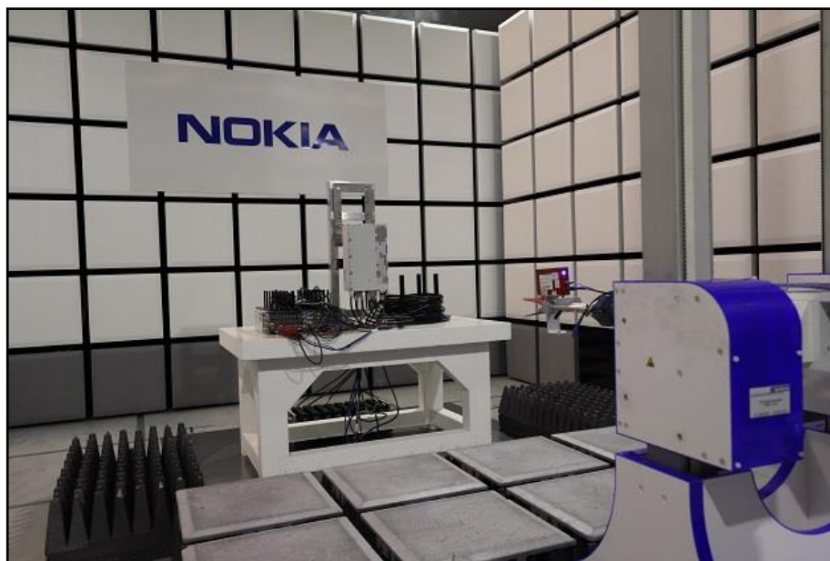
Figure 4 - Radiated Emissions (18 GHz to 40 GHz)
