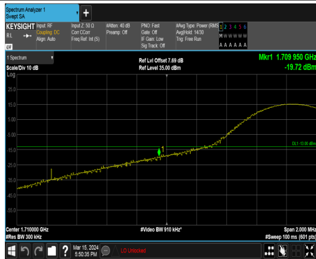
Band66-15MHz-QPSK-132047-1RB#74
