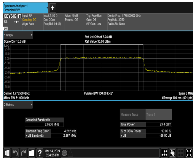
Band66-3MHz-16QAM-131987-15RB#0
