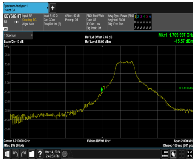
Band66-1.4MHz-16QAM-131979-1RB#5
