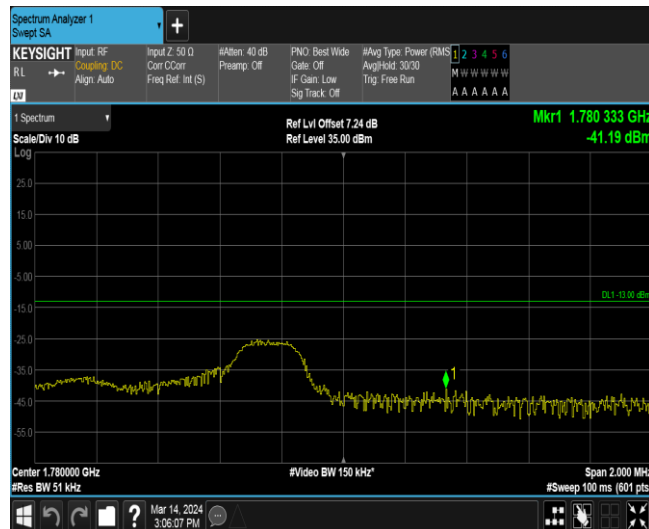
Band66-3MHz-16QAM-132657-1RB#14
