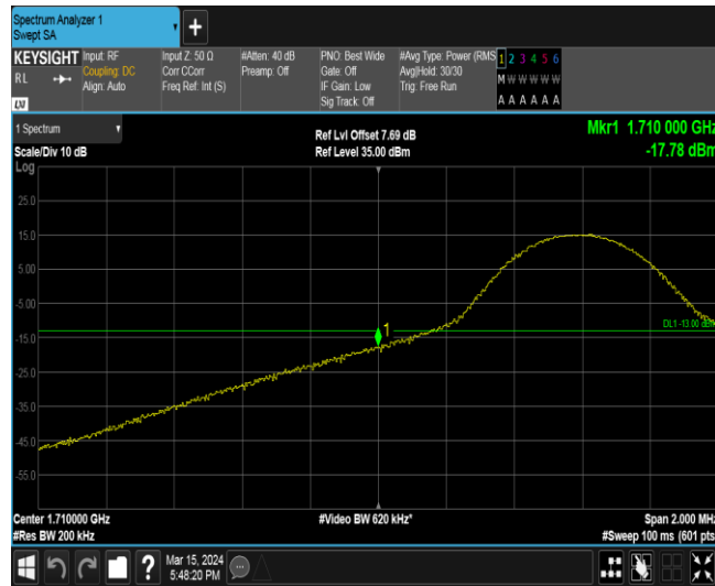
Band66-10MHz-QPSK-132022-1RB#49
