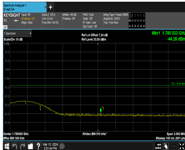
Band66-15MHz-QPSK-132597-1RB#74
