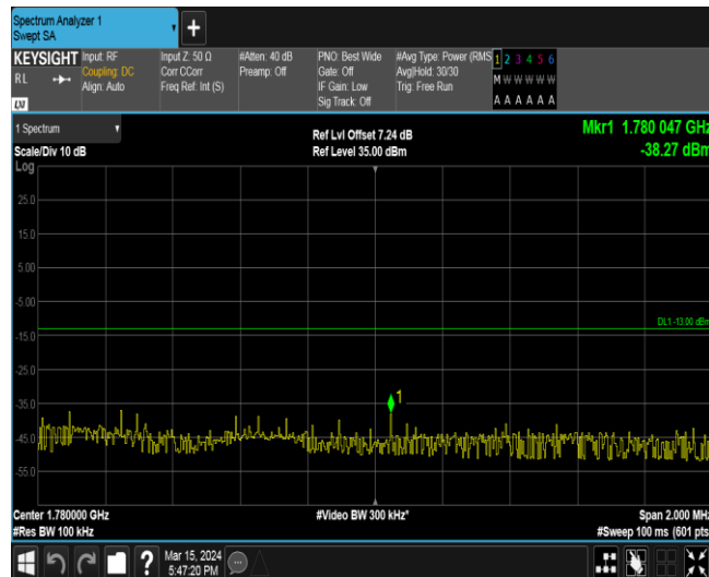
Band66-5MHz-16QAM-132647-1RB#24
