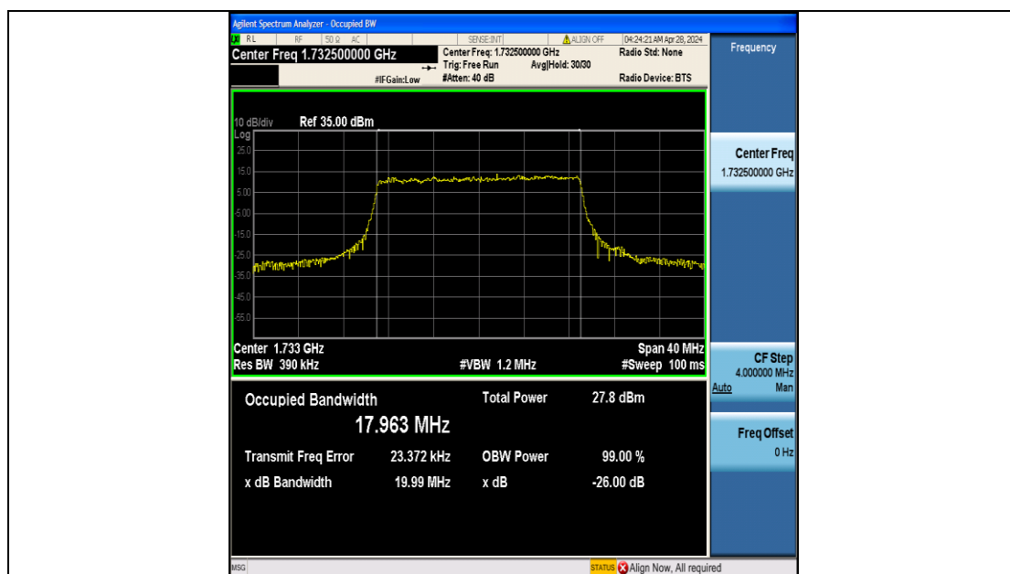
Band4-20MHz-QPSK-20175-100RB#0-PASS
