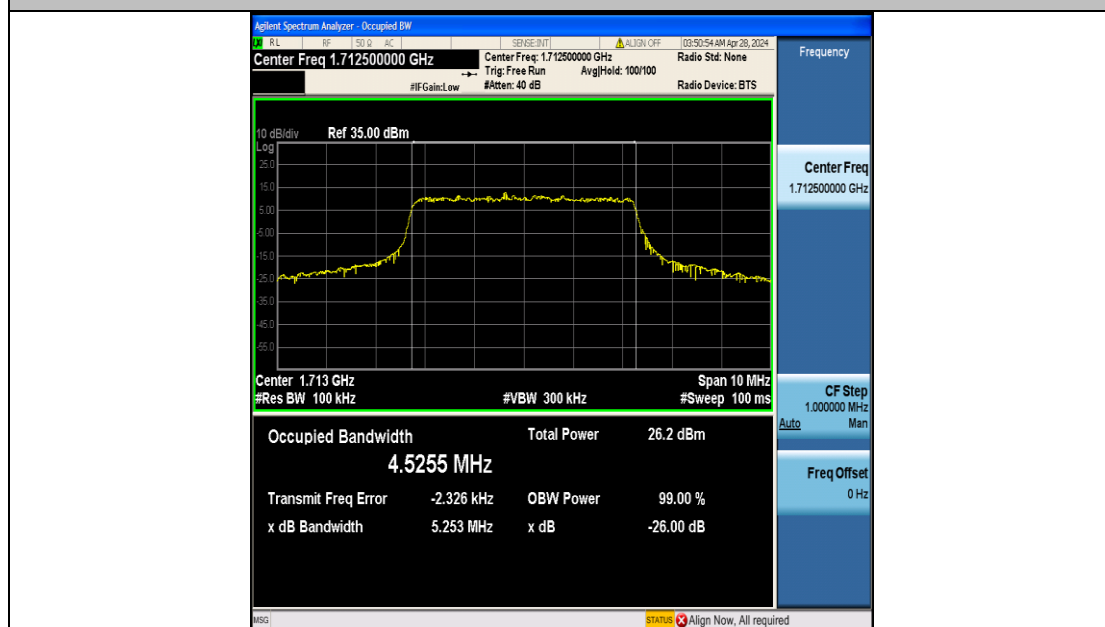
Band4-5MHz-16QAM-19975-25RB#0-PASS
