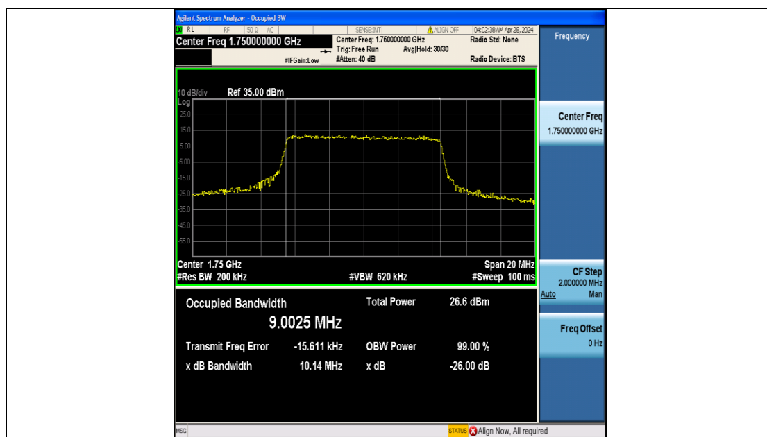
Band4-10MHz-QPSK-20350-50RB#0-PASS
