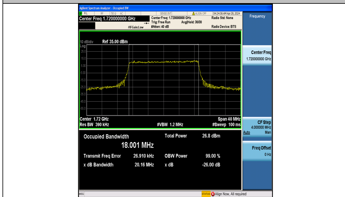
Band4-20MHz-16QAM-20050-100RB#0-PASS
