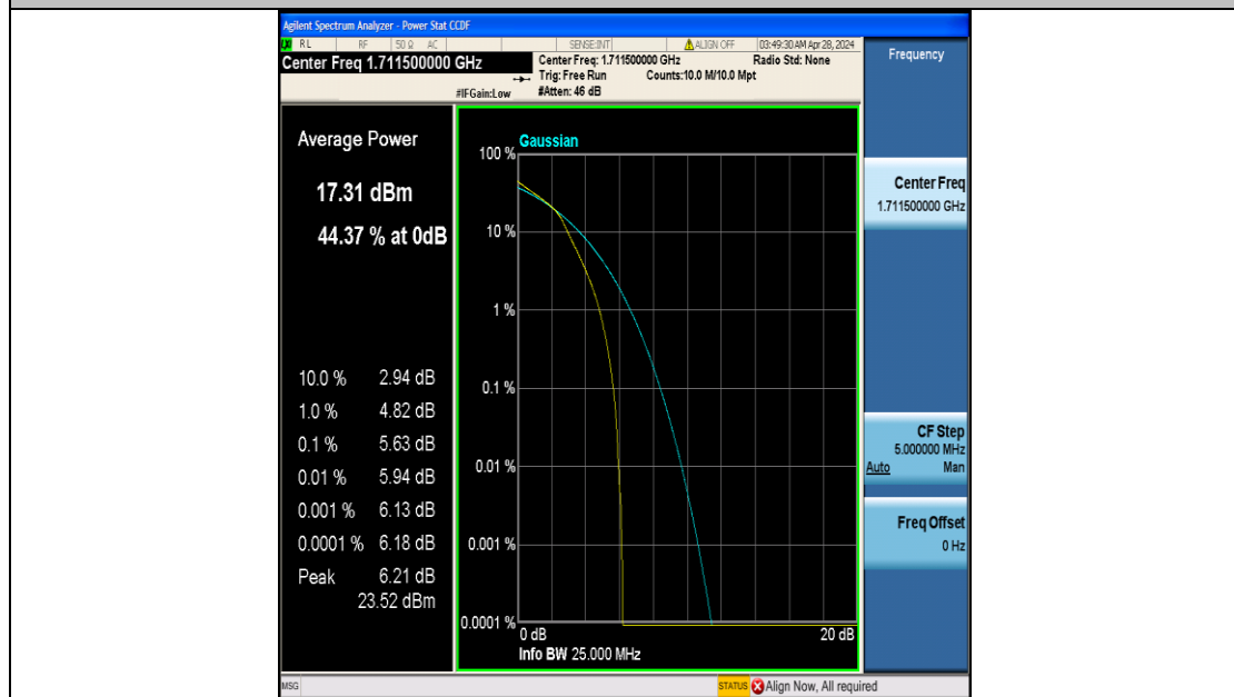
Band4-3MHz-16QAM-19965-15RB#0-PASS
