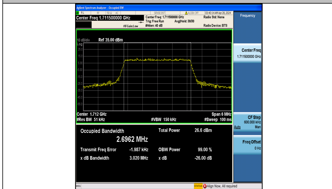
Band4-3MHz-16QAM-19965-15RB#0-PASS
