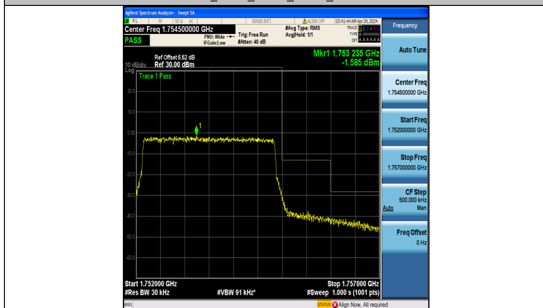
Band4_3MHz_16QAM_20385_15RB#0
