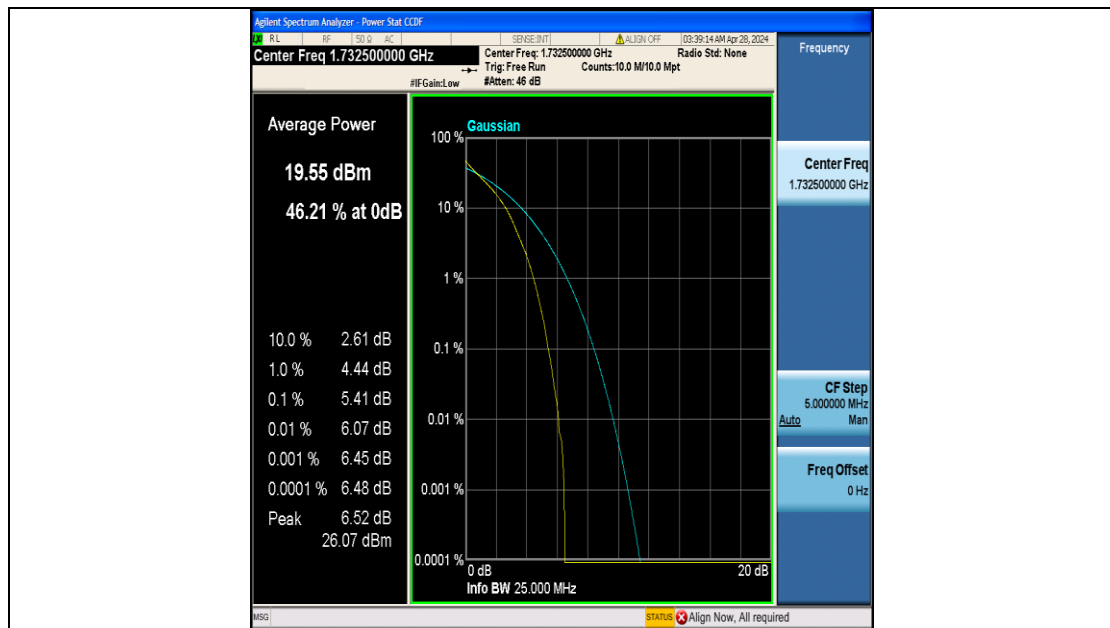
Band4-1.4MHz-QPSK-20175-6RB#0-PASS
