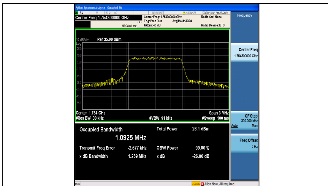
Band4-1.4MHz-QPSK-20393-6RB#0-PASS
