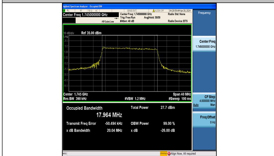
Band4-20MHz-16QAM-20300-100RB#0-PASS
