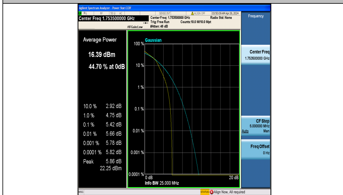
Band4-3MHz-16QAM-20385-15RB#0-PASS
