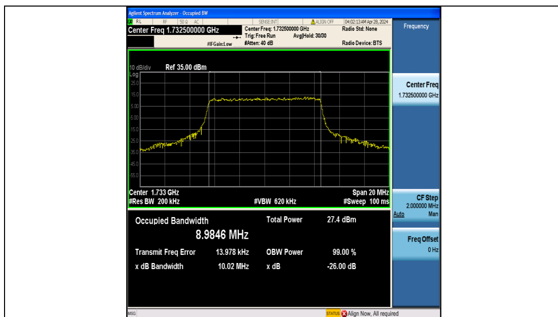
Band4-10MHz-QPSK-20175-50RB#0-PASS
