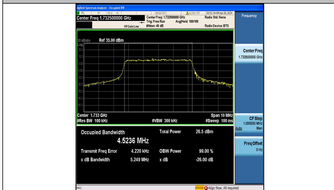
Band4-5MHz-16QAM-20175-25RB#0-PASS
