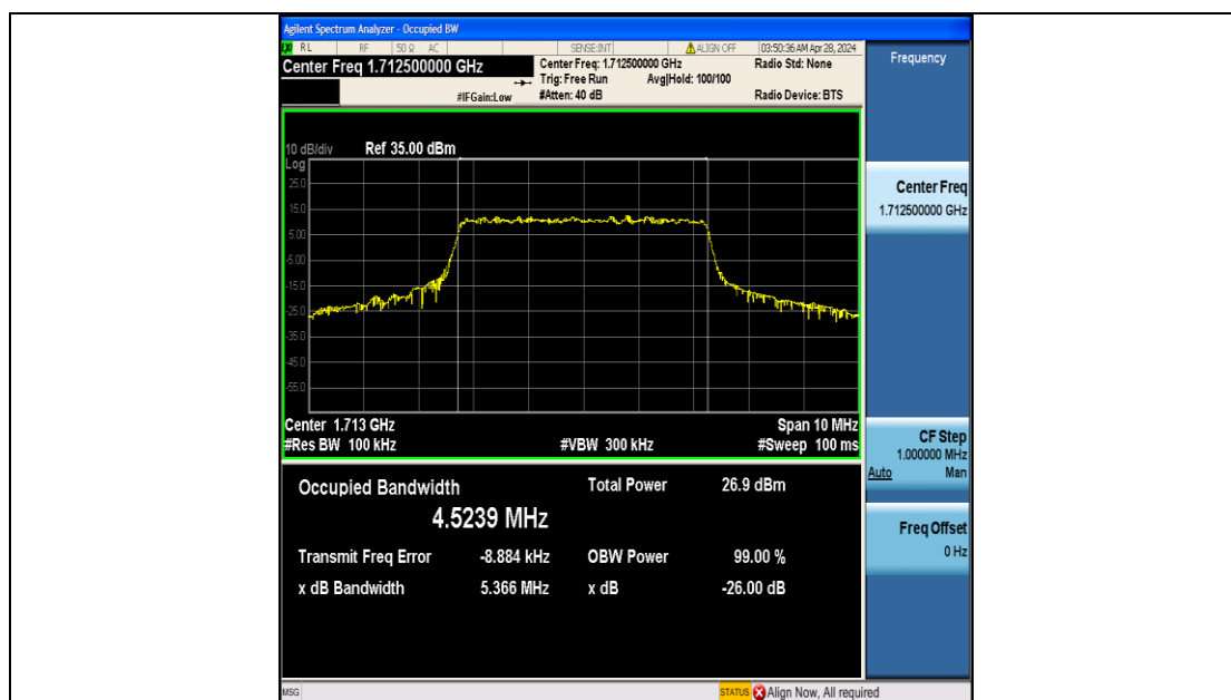
Band4-5MHz-QPSK-19975-25RB#0-PASS
