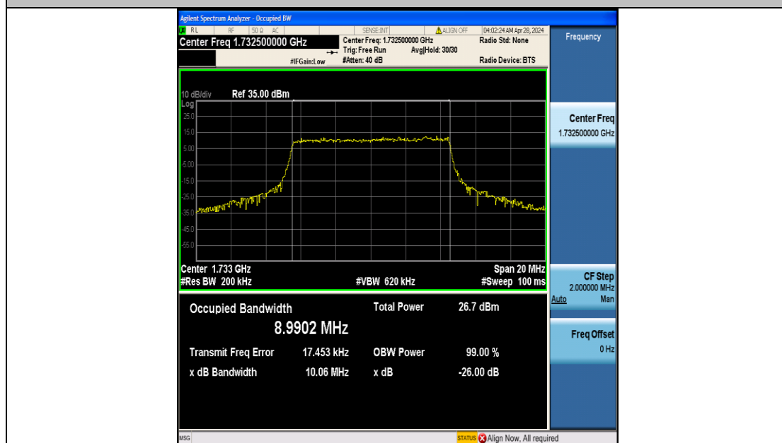
Band4-10MHz-16QAM-20175-50RB#0-PASS
