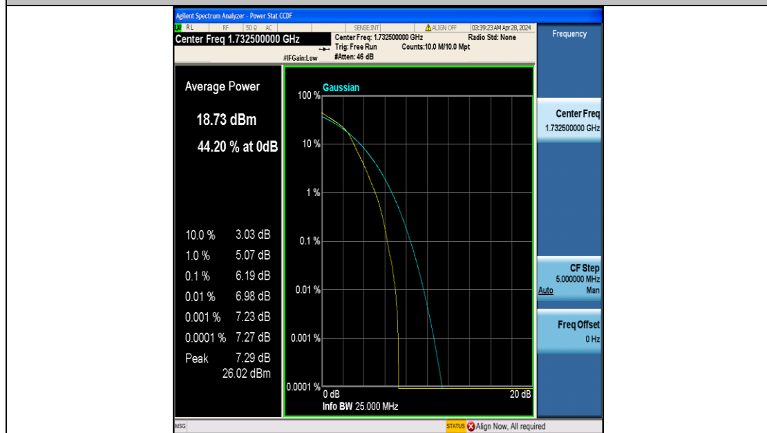
Band4-1.4MHz-16QAM-20175-6RB#0-PASS
