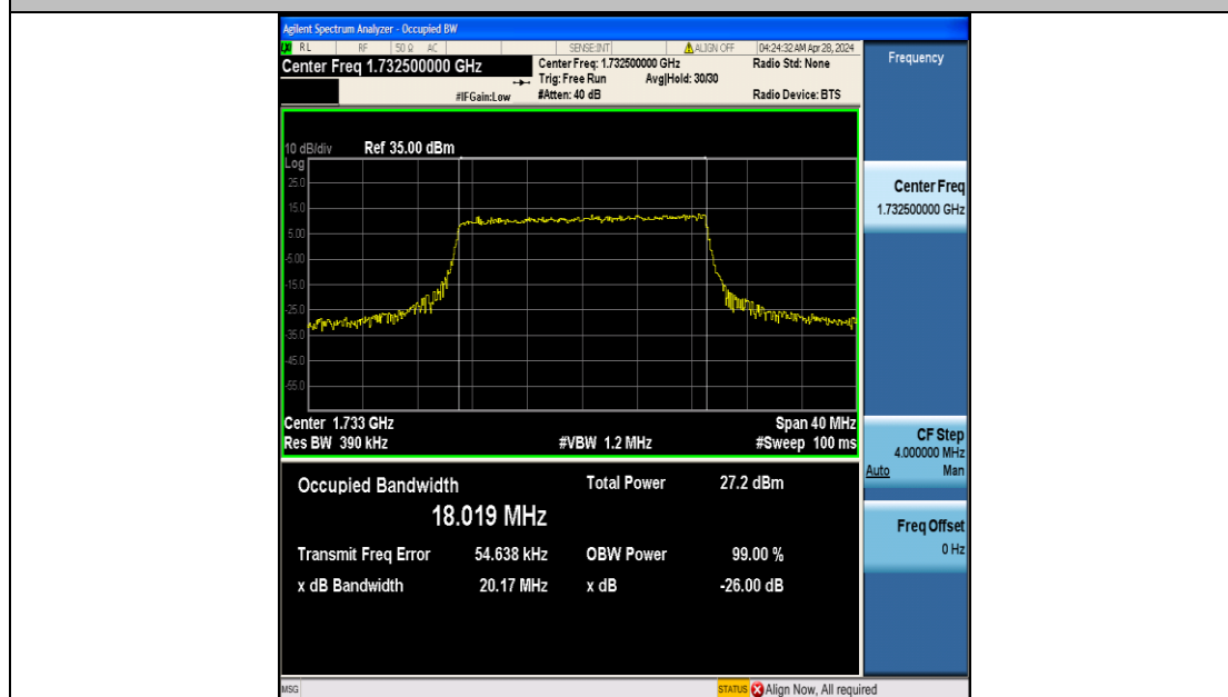
Band4-20MHz-16QAM-20175-100RB#0-PASS
