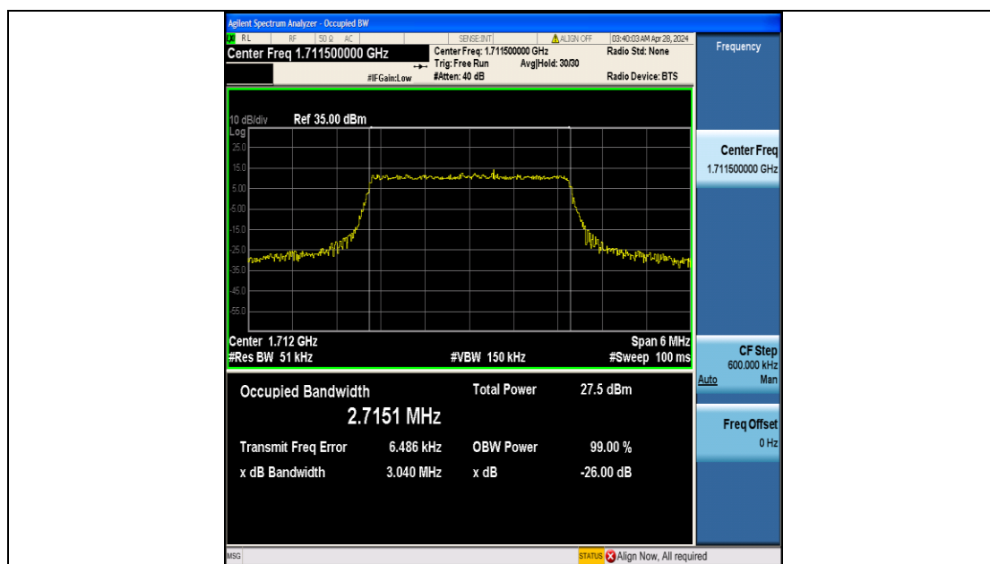
Band4-3MHz-QPSK-19965-15RB#0-PASS
