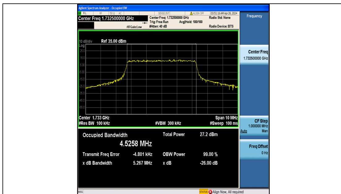
Band4-5MHz-QPSK-20175-25RB#0-PASS
