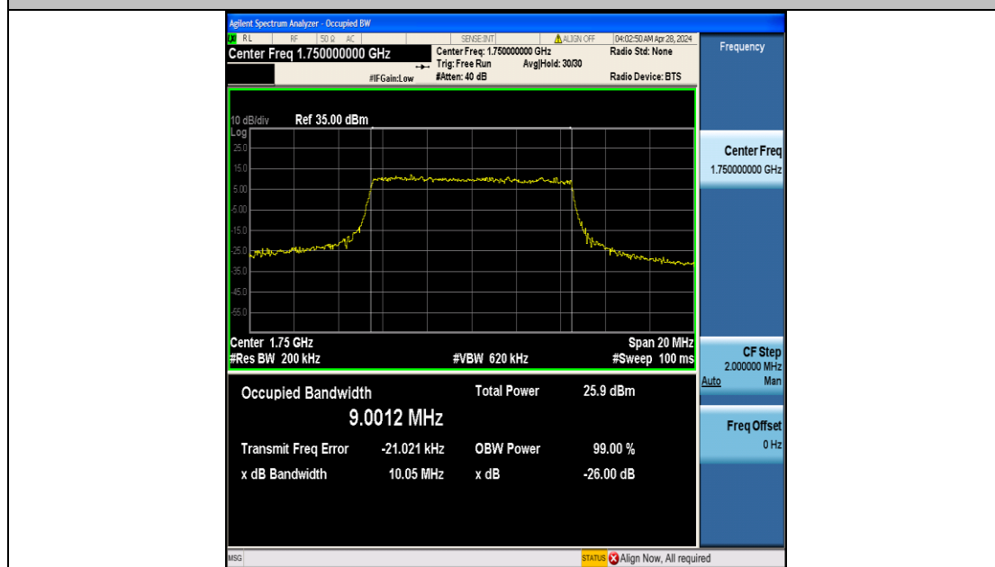
Band4-10MHz-16QAM-20350-50RB#0-PASS
