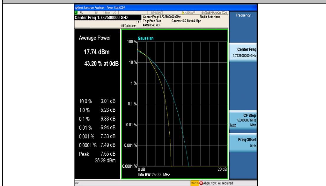
Band4-15MHz-16QAM-20175-75RB#0-PASS
