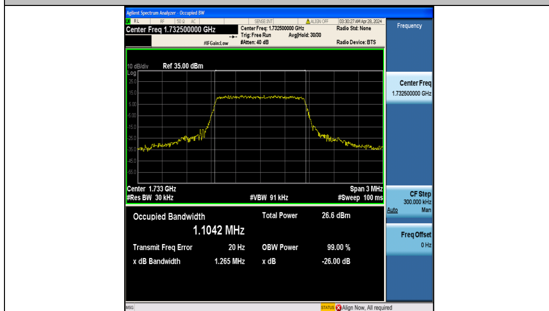
Band4-1.4MHz-16QAM-20175-6RB#0-PASS
