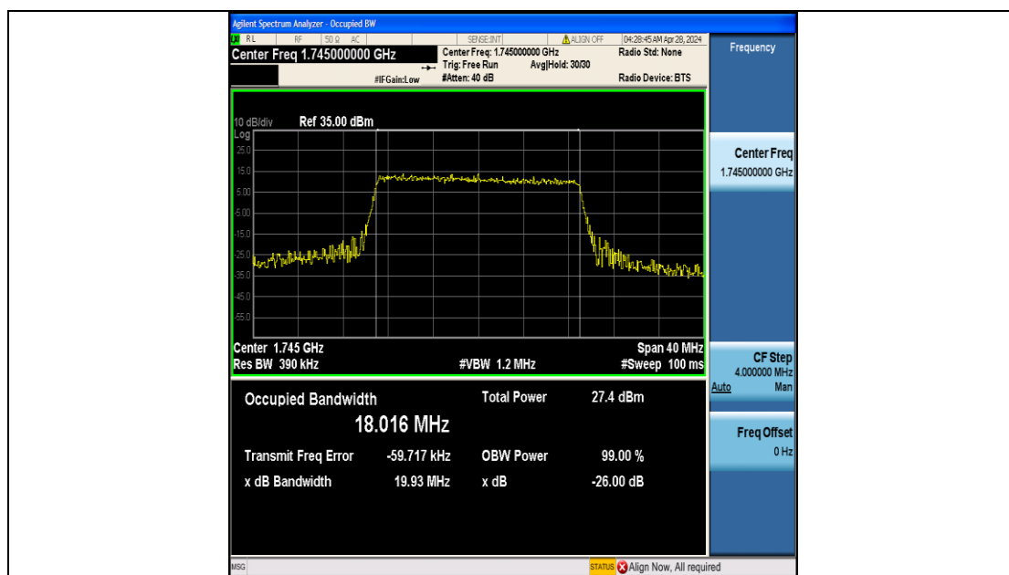
Band4-20MHz-QPSK-20300-100RB#0-PASS
