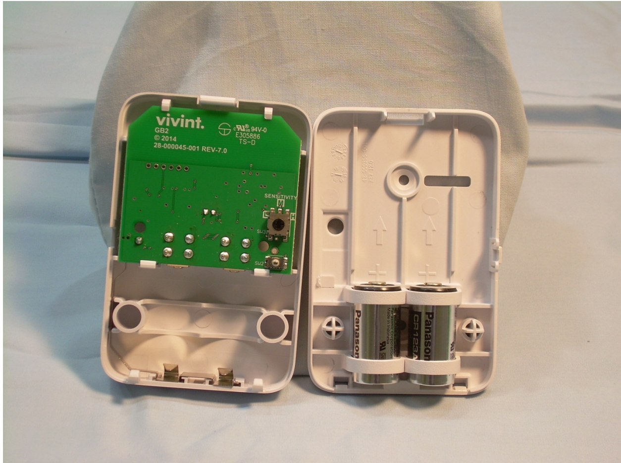
View of the EUT – Housing Opened
