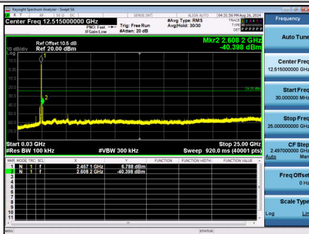
11G-Ant1-2462-30~25000-PASS
