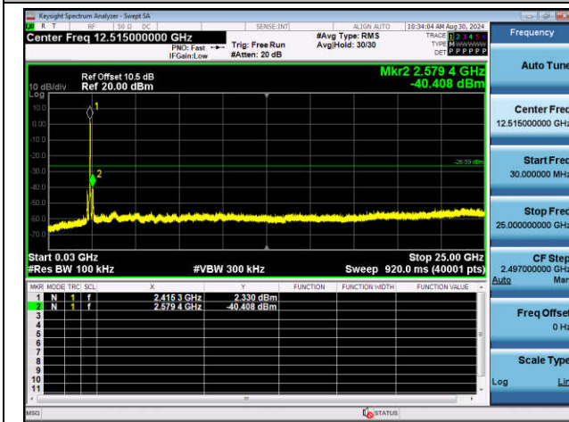
11AX40SISO-Ant2-2437-0~Reference-PASS
