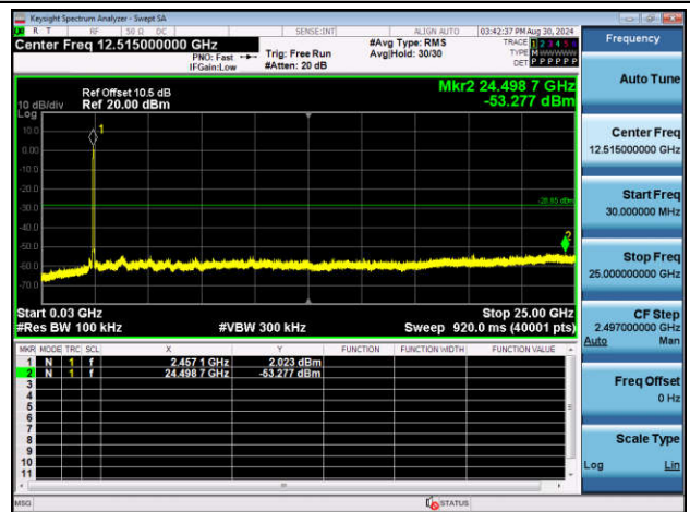
11AX40SISO-Ant1-2452-30~25000-PASS
