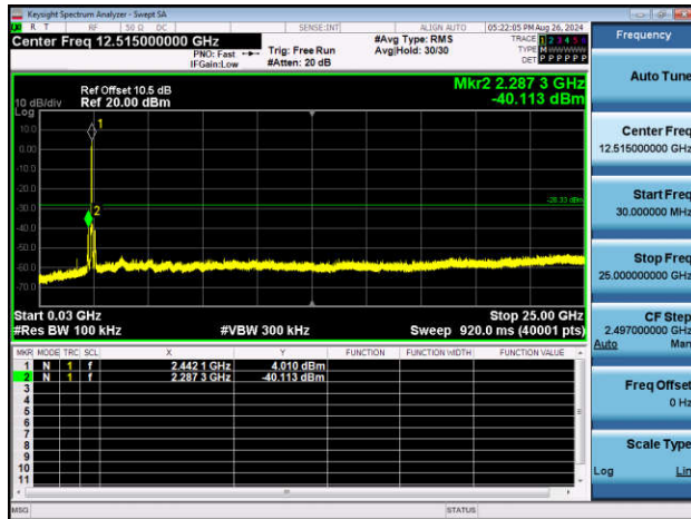
11N40SISO-Ant1-2452-0~Reference-PASS
