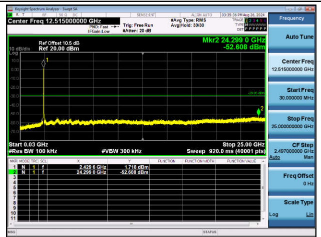
11N40SISO-Ant2-2437-0~Reference-PASS
