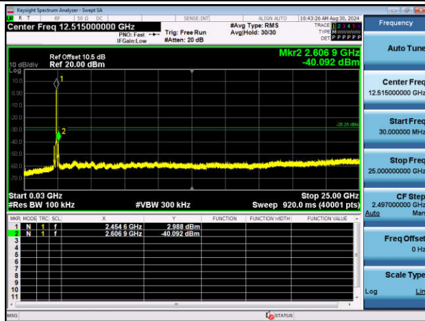
11AX40SISO-Ant2-2452-0~Reference-PASS
