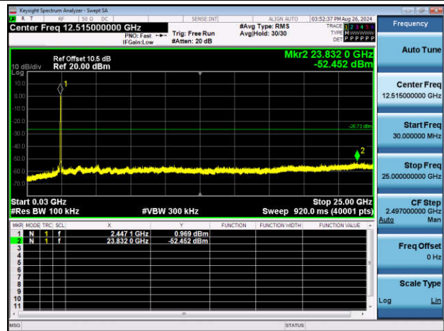
11N40SISO-Ant2-2452-30~25000-PASS
