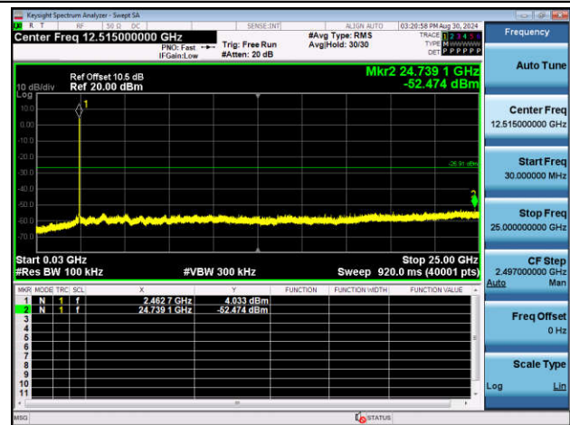
11AX20SISO-Ant1-2462-30~25000-PASS
