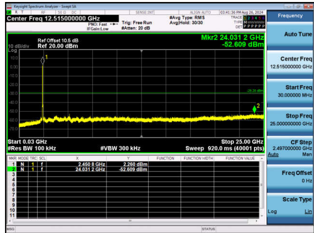
11N40SISO-Ant2-2452-0~Reference-PASS
