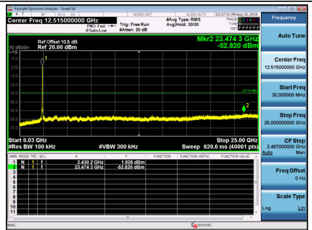
11AX40SISO-Ant1-2437-0~Reference-PASS
