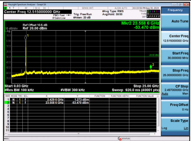
11AX40SISO-Ant1-2452-0~Reference-PASS
