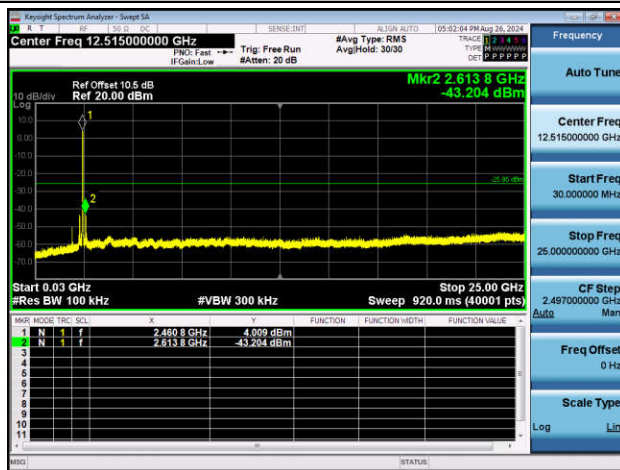
11N20SISO-Ant1-2462-30~25000-PASS
