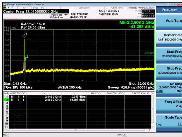
11N40SISO-Ant1-2452-30~25000-PASS
