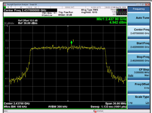
11AX20SISO-Ant2-2437-0~Reference-PASS
