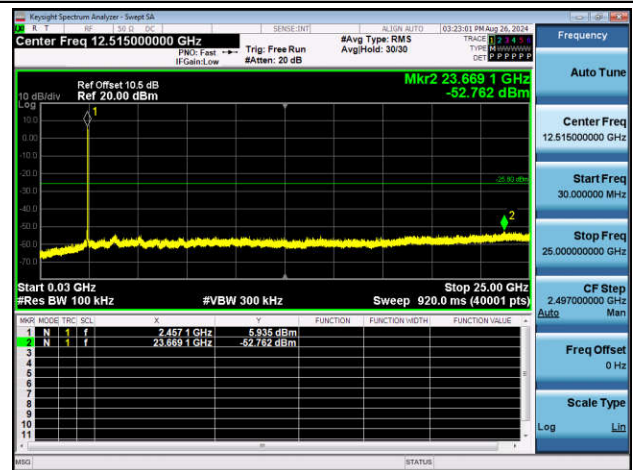
11N20SISO-Ant2-2462-30~25000-PASS
