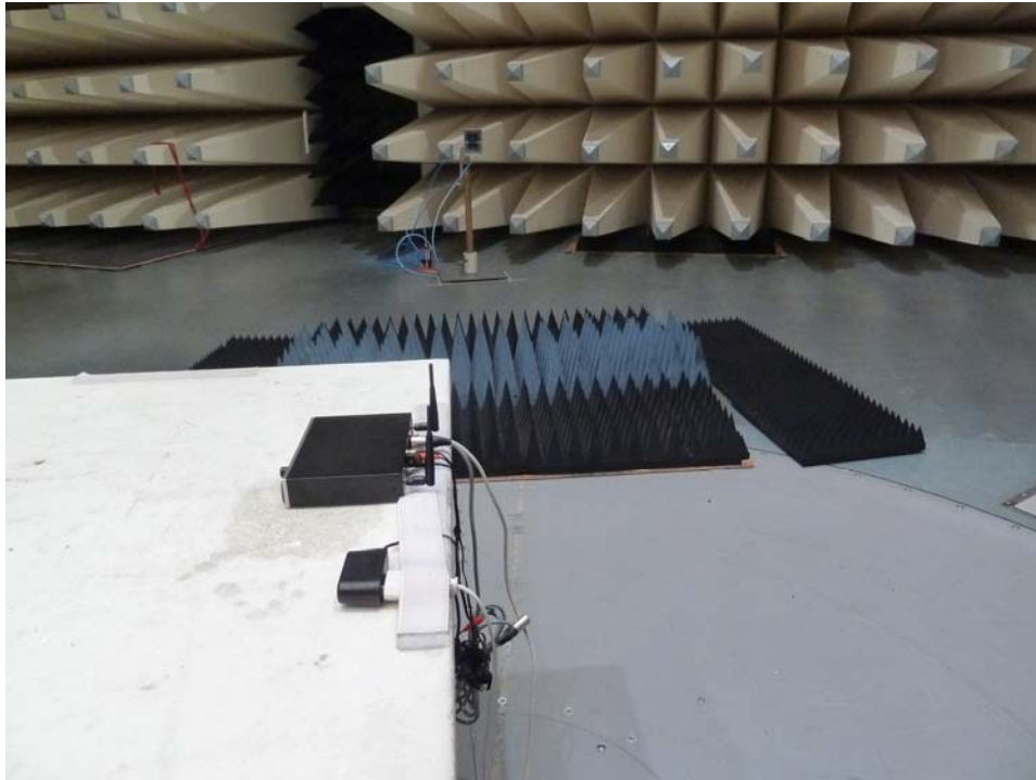
Photo 3: Radiated Emission
