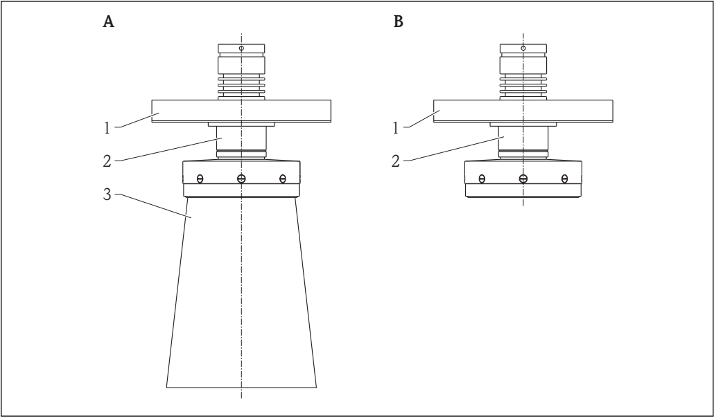
A Version with antenna extension (≥ DN200/8") B Version without antenna extension (DN100/4", DN150/6")
