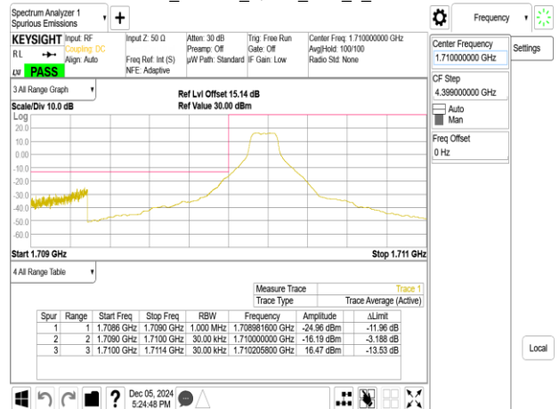
Band66_1.4MHz_QPSK_RB6_0_CH131979
