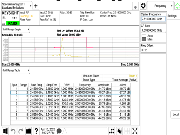
Band41_20MHz_QPSK_RB1_99_CH39790
