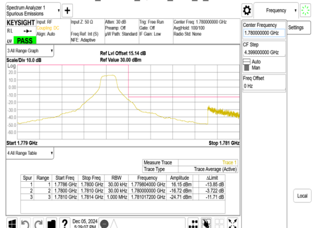
Band66_1.4MHz_QPSK_RB1_5_CH132665
