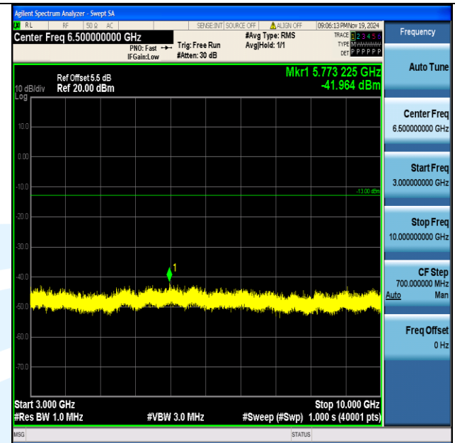
Band5_10MHz_16QAM_20450_1RB#0_3000~10000_3000~10000
