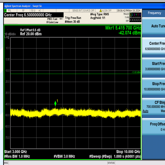
Band5_10MHz_QPSK_20525_1RB#0_3000~10000_3000~10000
