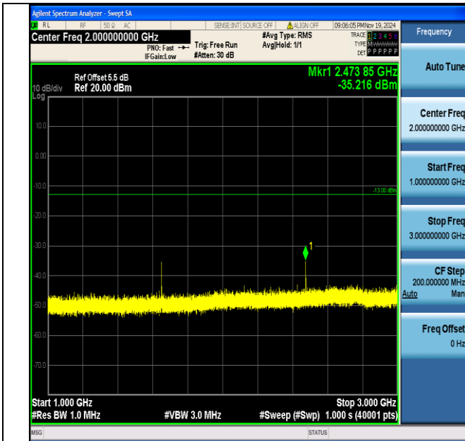
Band5_10MHz_16QAM_20450_1RB#0_1000~3000_1000~3000
