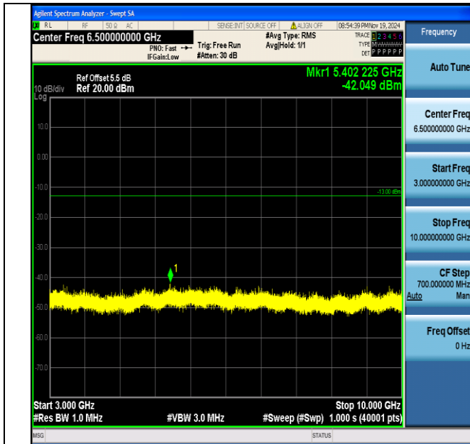
Band5_5MHz_QPSK_20625_1RB#0_3000~10000_3000~10000
