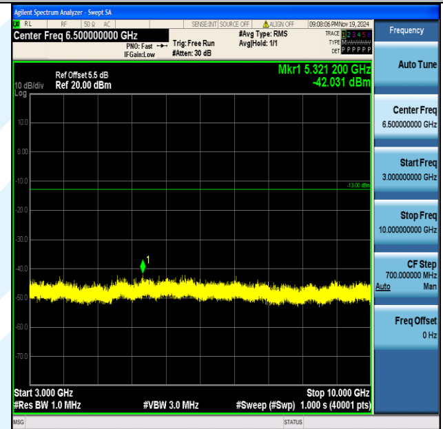
Band5_10MHz_16QAM_20600_1RB#0_3000~10000_3000~10000
