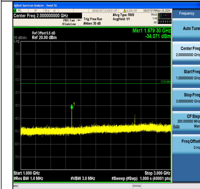
Band5_10MHz_16QAM_20600_1RB#0_1000~3000_1000~3000
