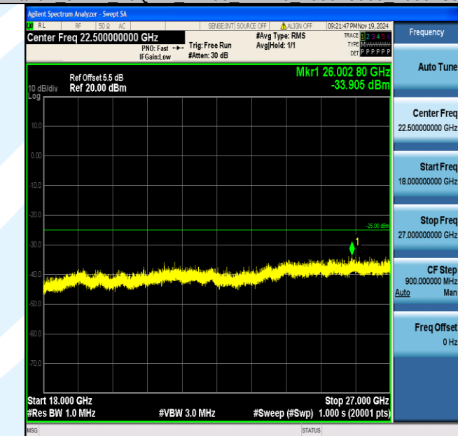
Band7_5MHz_16QAM_21100_1RB#0_18000~27000_18000~27000
