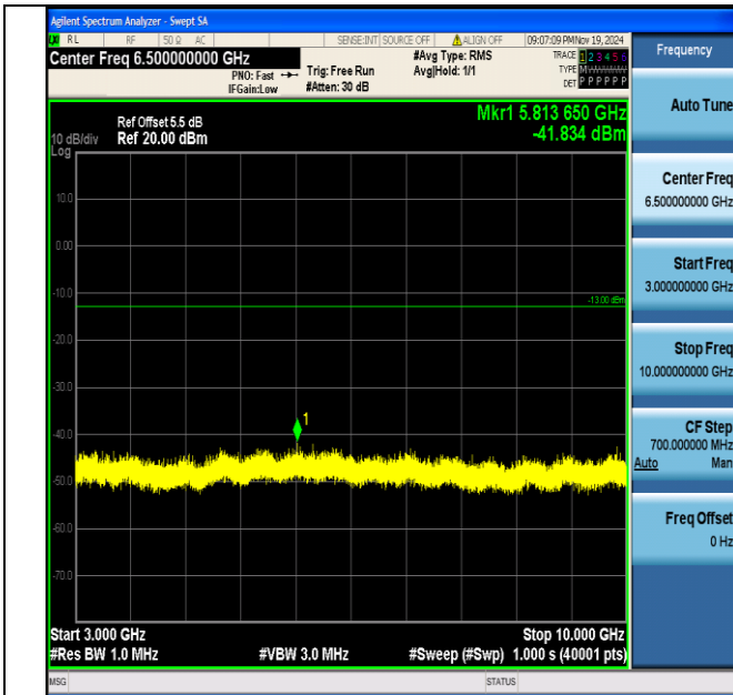
Band5_10MHz_16QAM_20525_1RB#0_3000~10000_3000~10000
