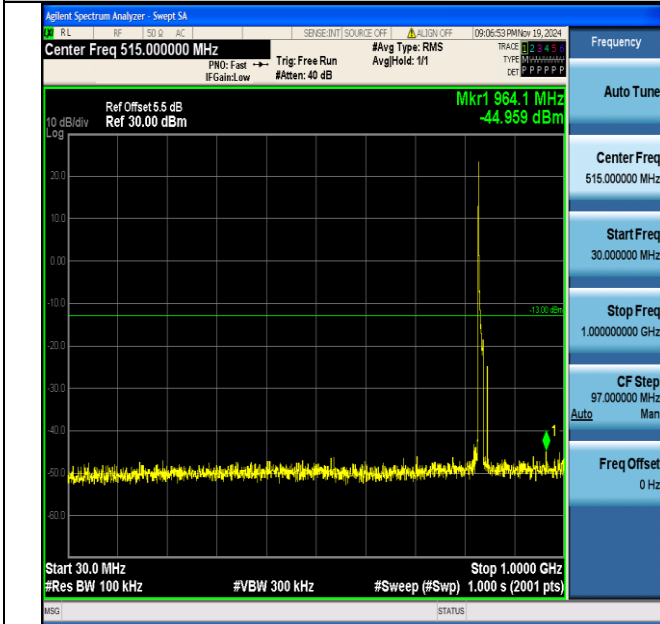
Band5_10MHz_16QAM_20525_1RB#0_30~1000_30~1000
