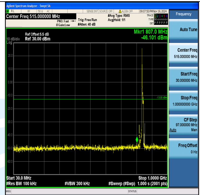
Band5_10MHz_16QAM_20600_1RB#0_30~1000_30~1000
