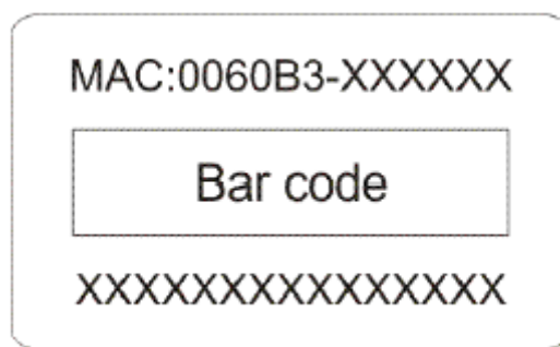
Figure 39 MAC Address
