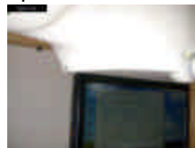
Figure A.12.1 Body SAR Test Setup -- Tablet Position, LCD Flip -- (Top Side)
