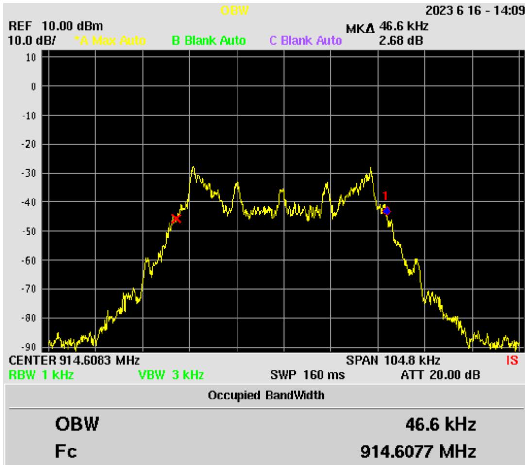
Figure 15. 99% Occupied Bandwidth – Mid Channel
