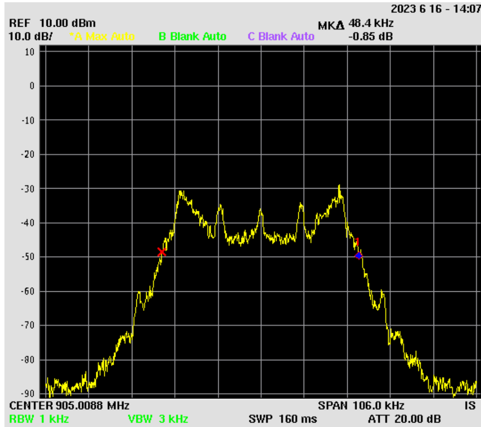
Figure 12. Twenty dB Bandwidth – Low Channel
