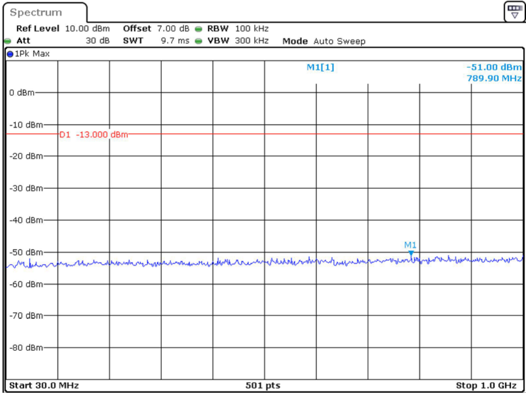
Band 4_10 MHz_Low_QPSK_RB50#0_1(30MHz-1GHz)
