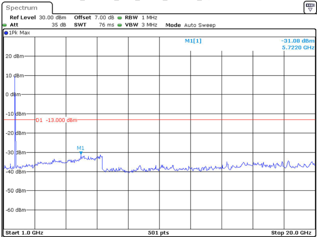
Band 4_10 MHz_Low_QPSK_RB50#0_2(1GHz-20GHz)
