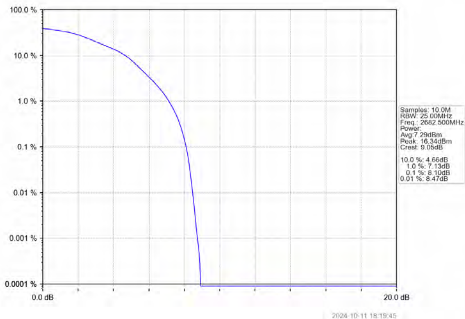
Band41 15MHz 16QAM HCH 2682.5MHz RB 75 0 NTN
