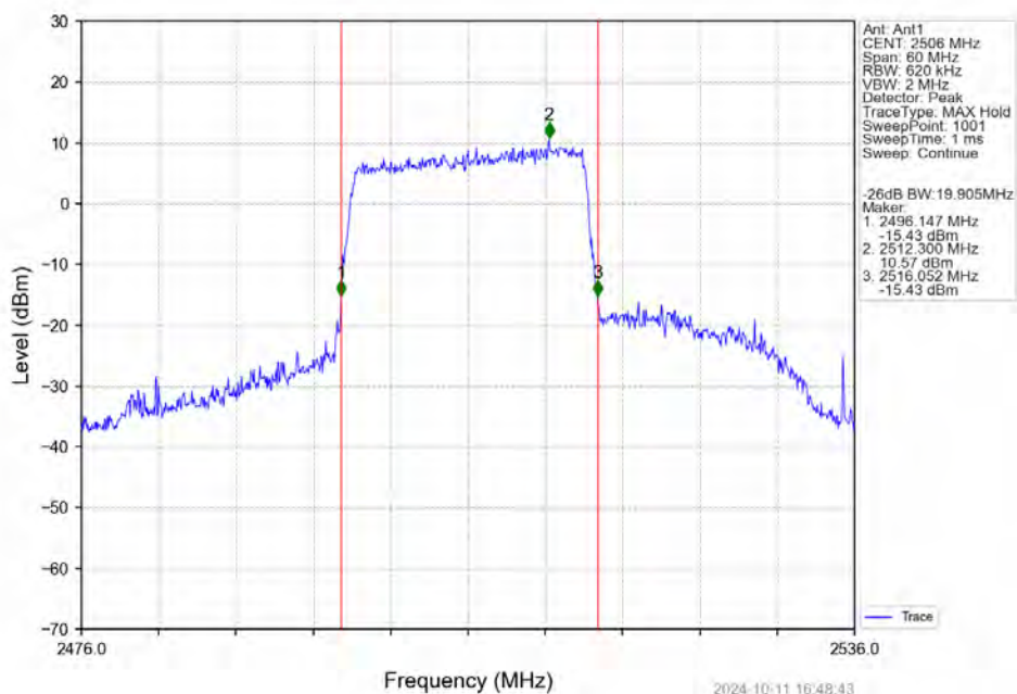
Band41_20MHz_16QAM_LCH_2506MHz_RB_100_0 NTN
