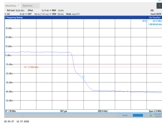
Band66-3MHz-QPSK-132657-15RB#0
