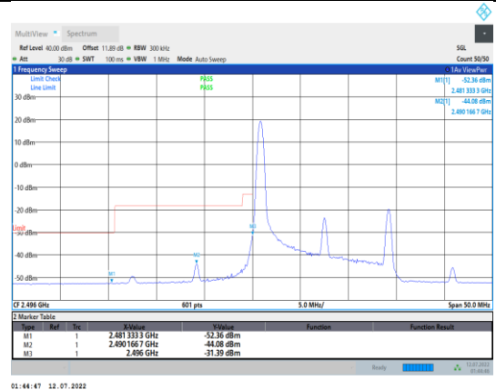
Band41-15MHz-16QAM-39725-1RB#0
