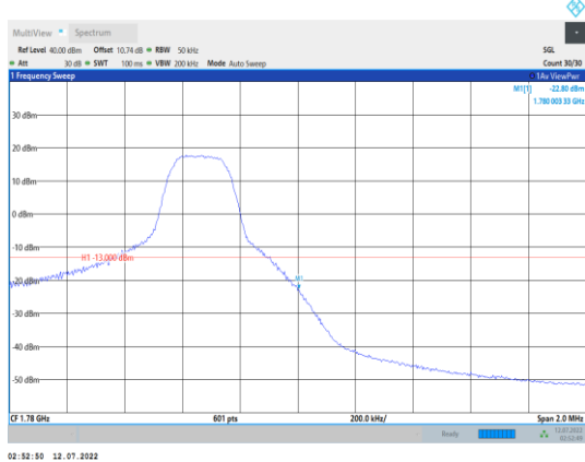
Band66-5MHz-16QAM-132647-1RB#24
