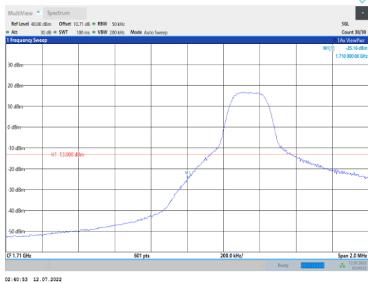
Band66-5MHz-16QAM-131997-1RB#0
