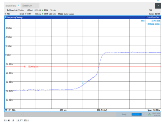
Band66-5MHz-QPSK-131997-25RB#0
