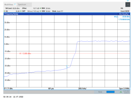
Band66-1.4MHz-16QAM-131979-6RB#0
