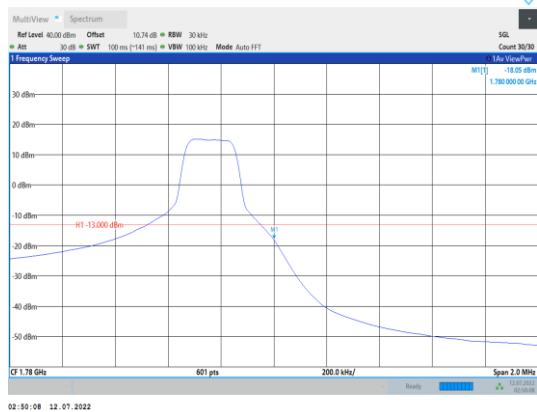
Band66-3MHz-16QAM-132657-1RB#14
