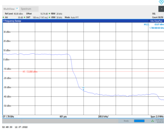
Band66-1.4MHz-QPSK-132665-6RB#0
