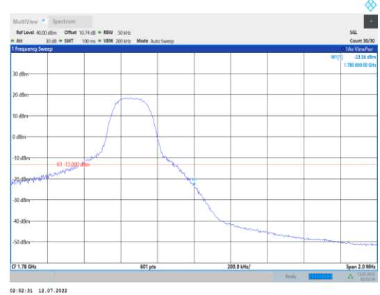
Band66-5MHz-QPSK-132647-1RB#24
