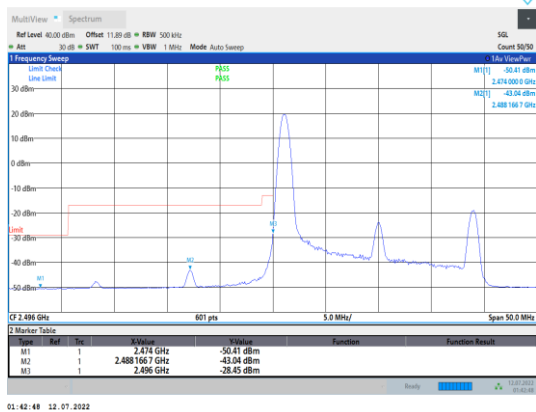
Band41-20MHz-16QAM-39750-1RB#0
