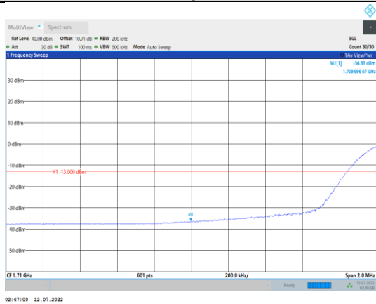
Band66-20MHz-16QAM-132072-100RB#0
