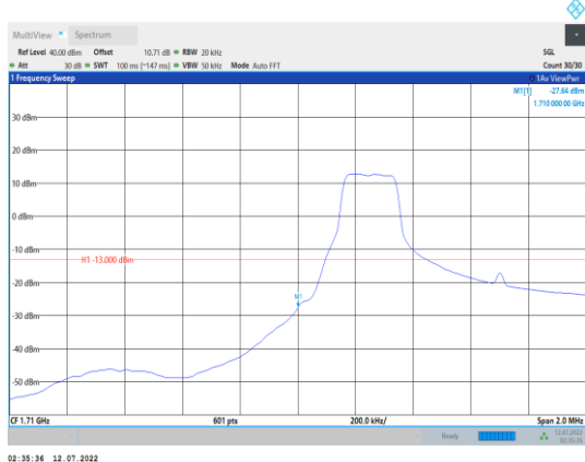
Band66-1.4MHz-16QAM-131979-1RB#0
