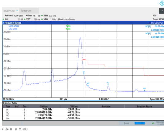
Band41-15MHz-QPSK-41515-1RB#74
