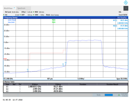
Band41-15MHz-16QAM-39725-75RB#0
