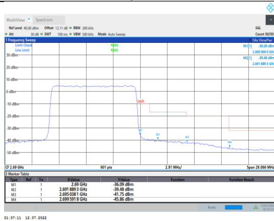
Band41-10MHz-QPSK-41540-50RB#0
