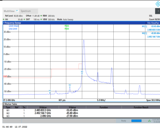
Band41-10MHz-16QAM-39700-1RB#0
