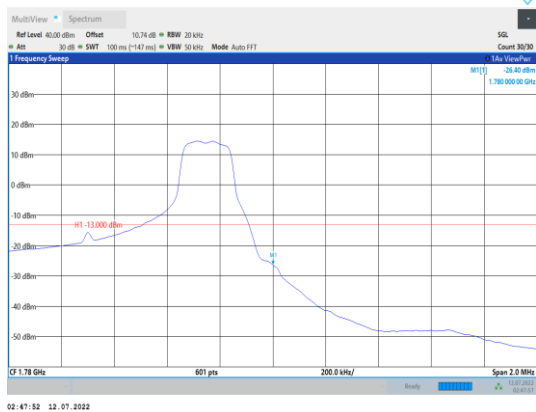
Band66-1.4MHz-QPSK-132665-1RB#5
