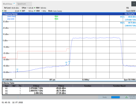
Band41-20MHz-16QAM-39750-100RB#0
