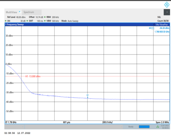
Band66-20MHz-16QAM-132572-100RB#0
