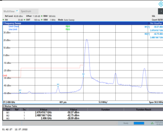
Band41-20MHz-QPSK-39750-1RB#0
