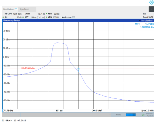
Band66-3MHz-QPSK-132657-1RB#14
