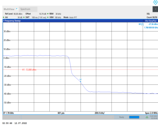
Band66-3MHz-16QAM-132657-15RB#0
