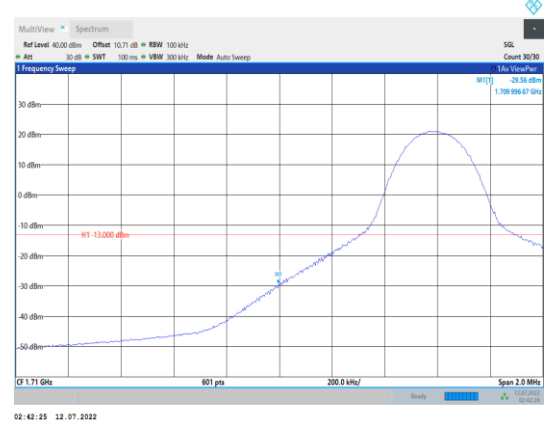
Band66-10MHz-QPSK-132022-1RB#0
