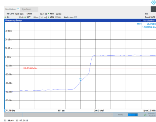
Band66-3MHz-16QAM-131987-15RB#0
