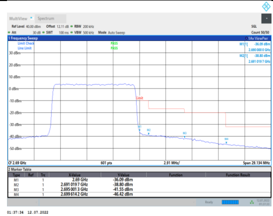
Band41-10MHz-16QAM-41540-50RB#0
