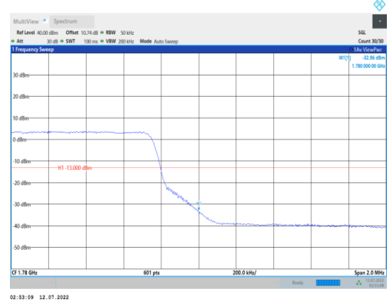
Band66-5MHz-QPSK-132647-25RB#0
