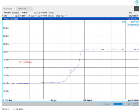
Band66-3MHz-QPSK-131987-15RB#0
