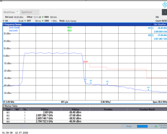
Band41-15MHz-16QAM-41515-75RB#0
