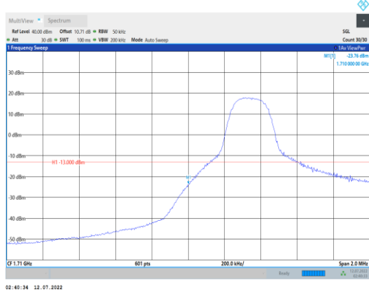
Band66-5MHz-QPSK-131997-1RB#0
