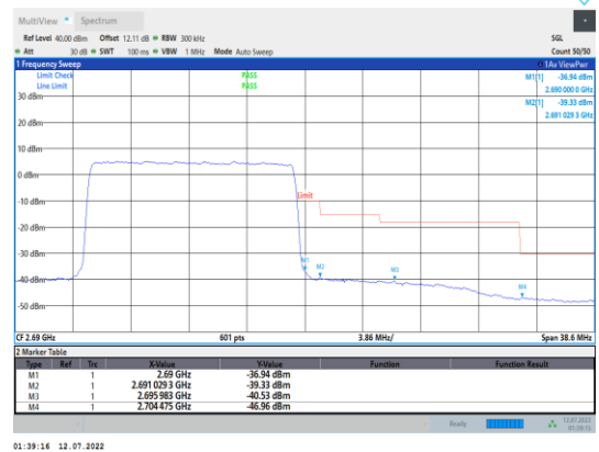
Band41-15MHz-QPSK-41515-75RB#0
