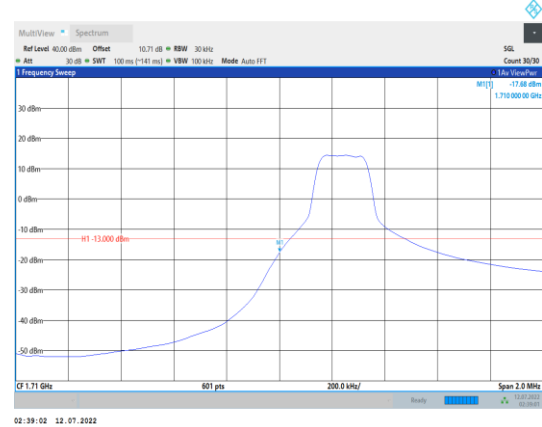
Band66-3MHz-16QAM-131987-1RB#0
