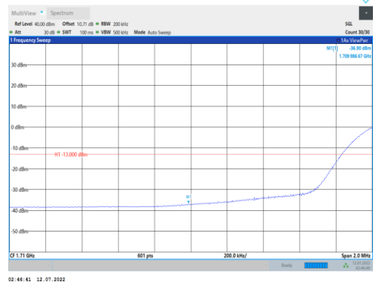
Band66-20MHz-QPSK-132072-100RB#0
