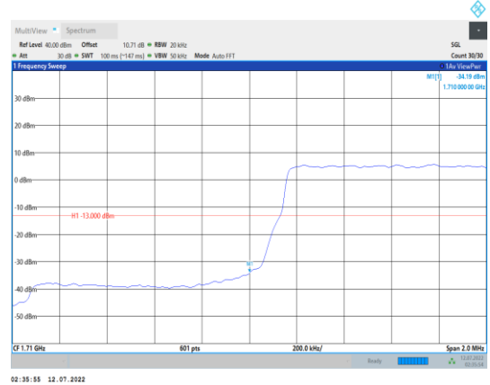
Band66-1.4MHz-QPSK-131979-6RB#0
