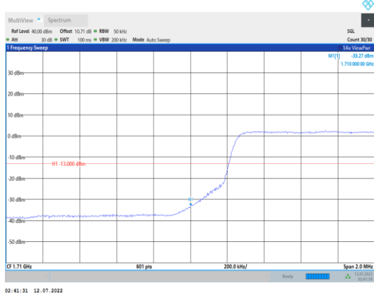
Band66-5MHz-16QAM-131997-25RB#0
