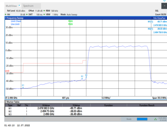
Band41-20MHz-QPSK-39750-100RB#0
