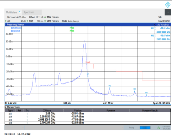
Band41-10MHz-16QAM-41540-1RB#49
