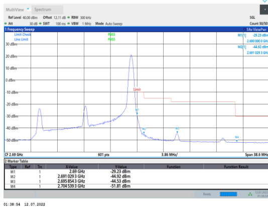
Band41-15MHz-16QAM-41515-1RB#74
