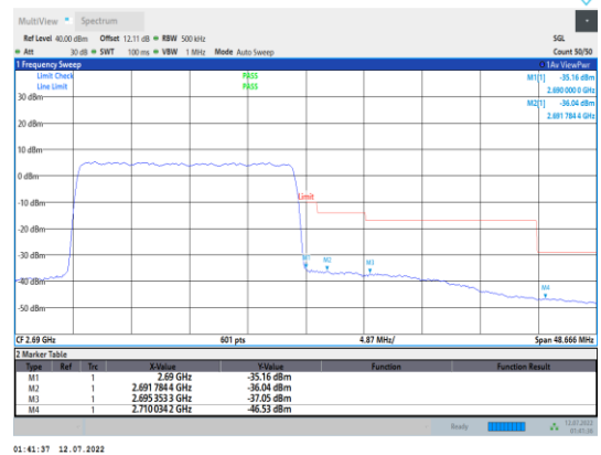
Band41-20MHz-16QAM-41490-100RB#0
