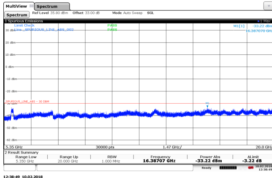
Figure 104 Spurious Emissions (5.35 GHz – 20 GHz) – QPSK (5220.0 MHz) (20MHz Channel BW)
