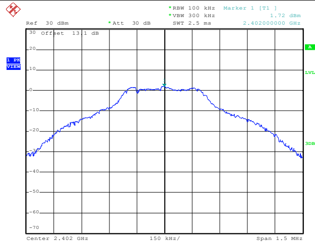
DH5_Ant1_2402_0~Reference
