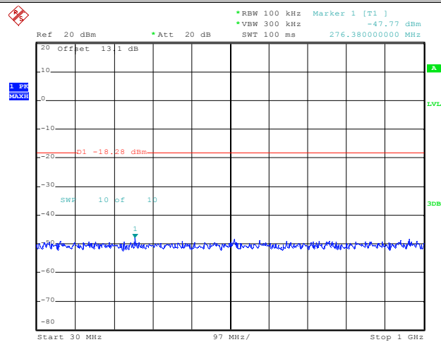
DH5_Ant1_2402_30~1000
