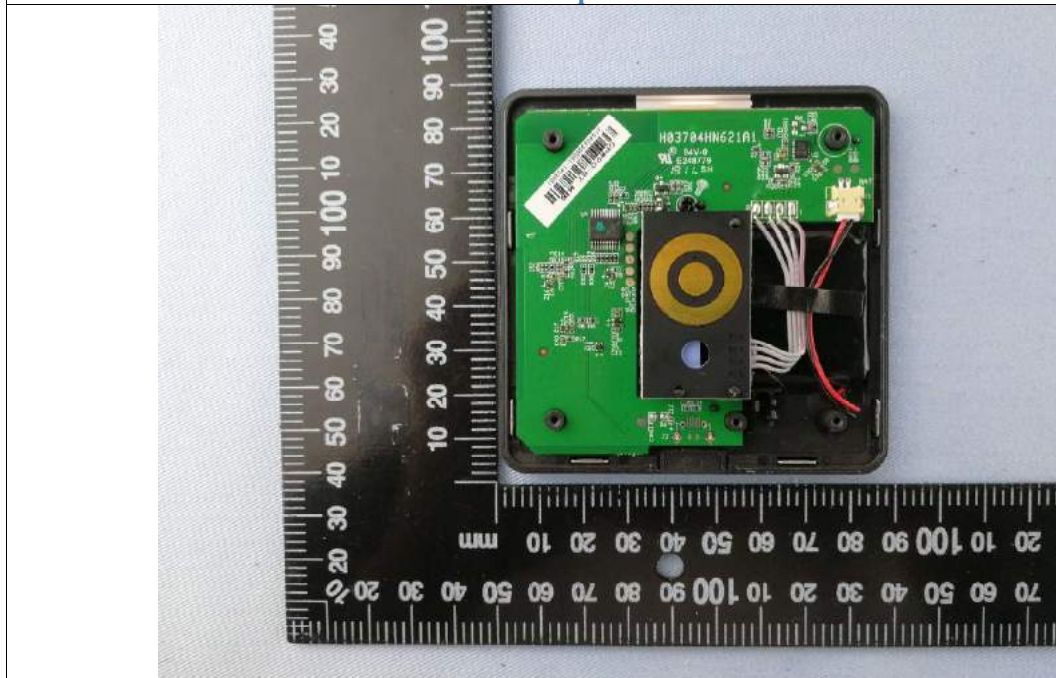
Board layout side view
