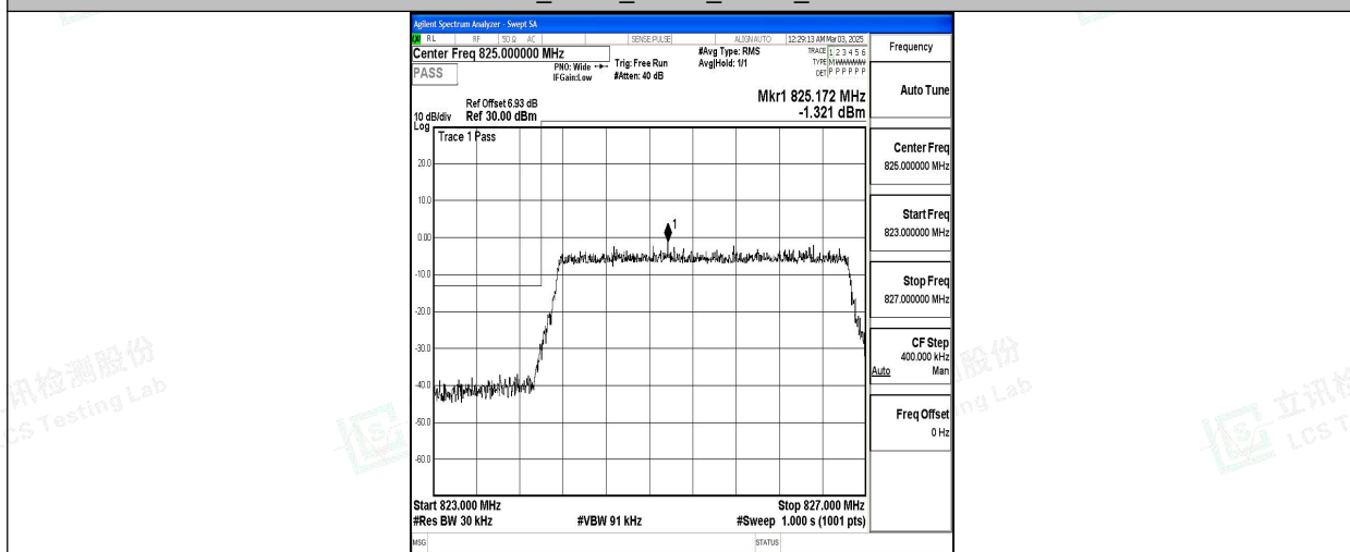
Band5_3MHz_16QAM_20415_15RB#0
