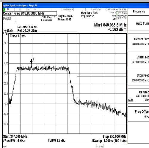
Band5_1.4MHz_16QAM_20643_6RB#0
