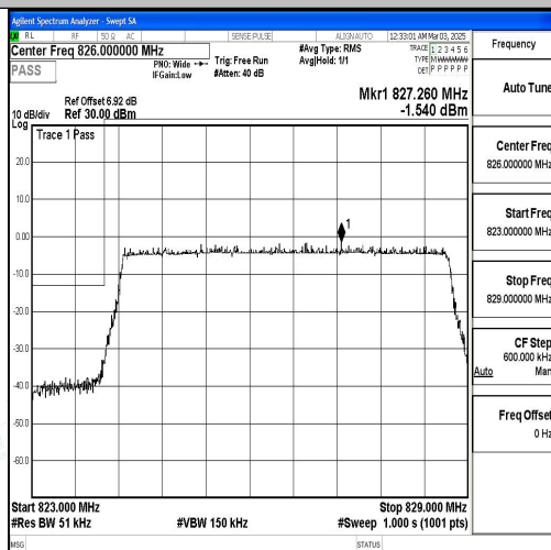
Band5_5MHz_QPSK_20425_25RB#0
