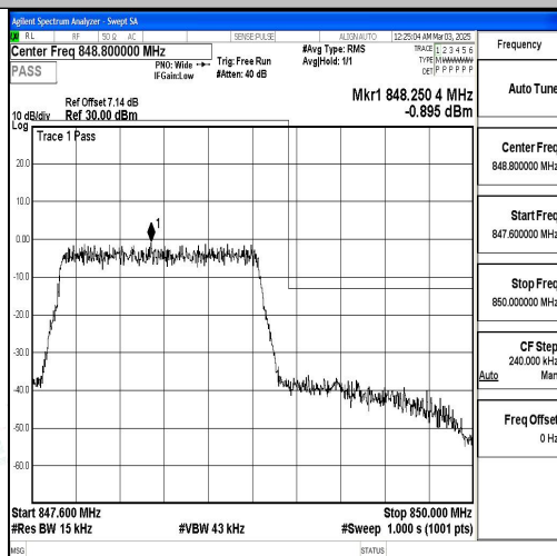
Band5_1.4MHz_QPSK_20643_6RB#0
