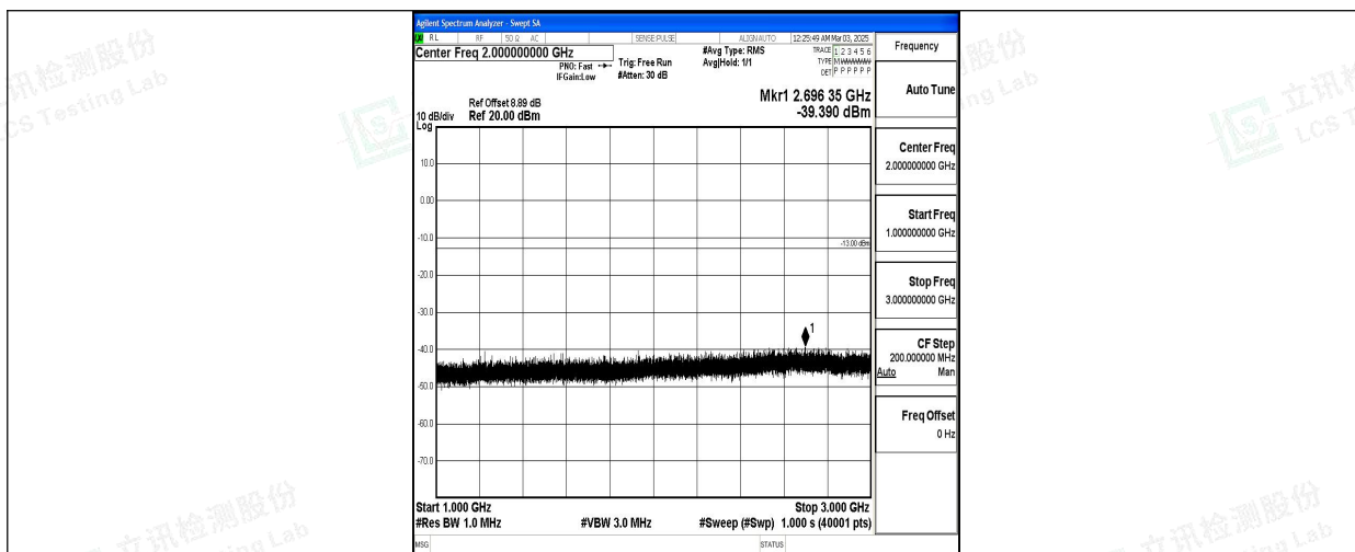
Band5_1.4MHz_QPSK_20407_1RB#0_1000~3000_1000~3000
