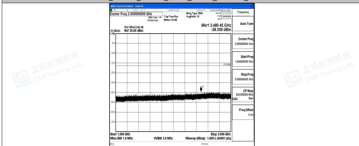
Band5_1.4MHz_16QAM_20407_1RB#0_1000~3000_1000~3000
