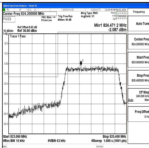
Band5_1.4MHz_16QAM_20407_6RB#0
