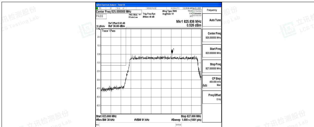
Band5_3MHz_QPSK_20415_15RB#0
