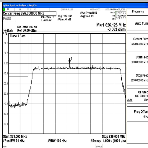
Band5_5MHz_16QAM_20425_25RB#0
