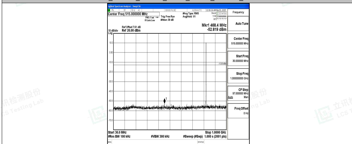
Band5_1.4MHz_16QAM_20407_1RB#0_30~1000_30~1000
