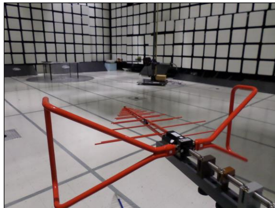
Photograph 4. Radiated Spurious Emissions, Test Setup – Below 1 GHz (Antenna)
