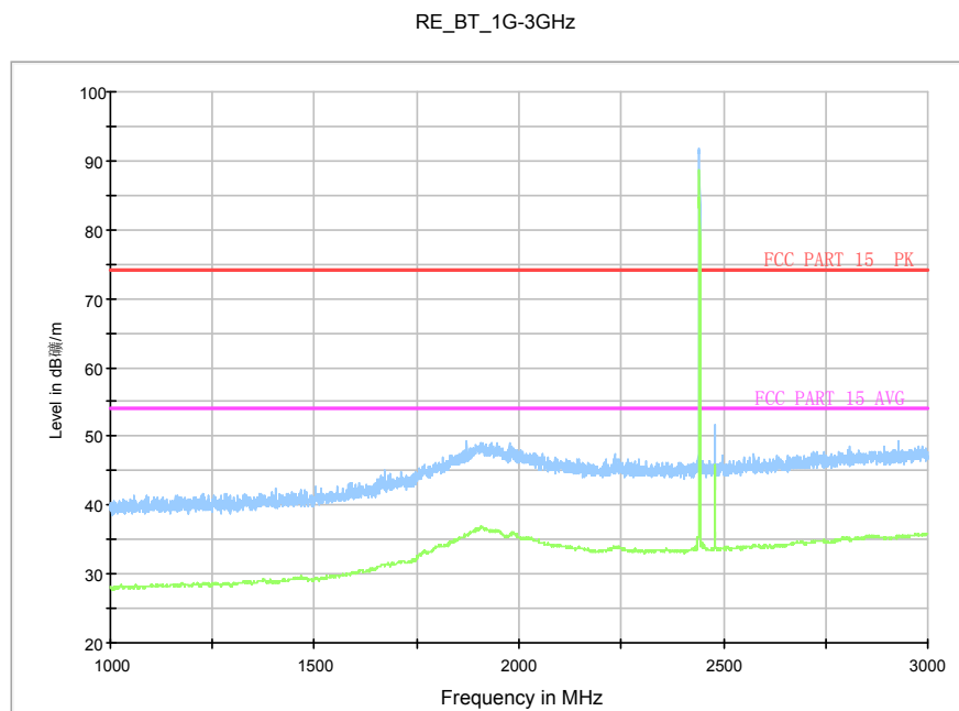
Fig.81. Radiated emission: 8DPSK, Channel 39, 1 GHz - 3 GHz
