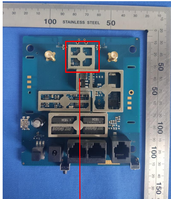
Internal 4-- Main board face
