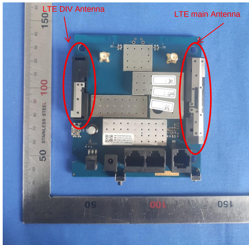
Internal 3 -- Main board face
