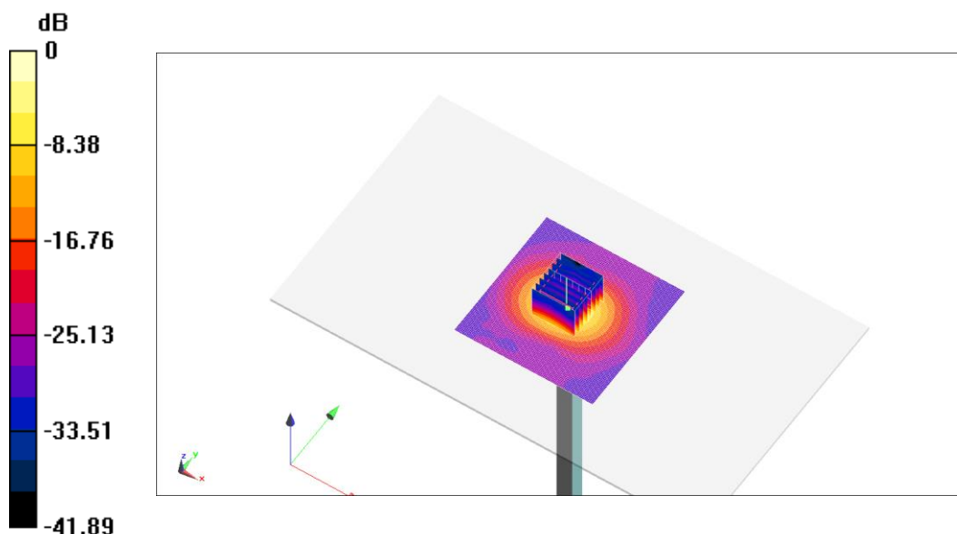
Fig.B.3 validation 5600 MHz 250mW
