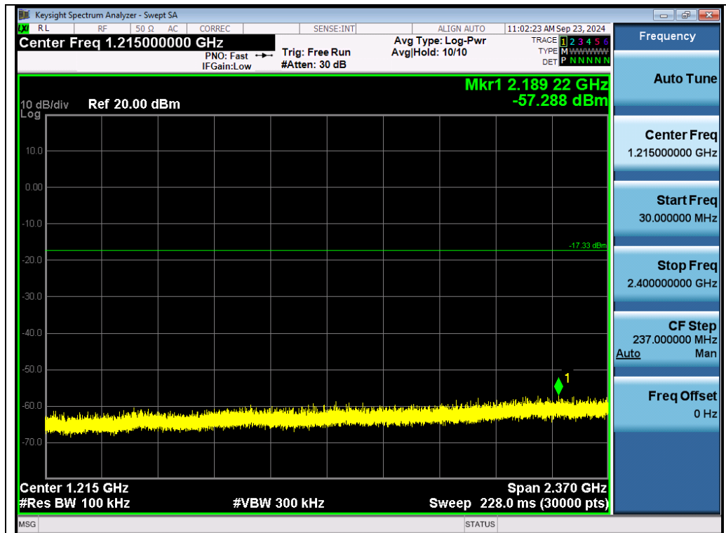
Test_Graph_2.4G_ANT1_2441.85_Lower Band Emissions
