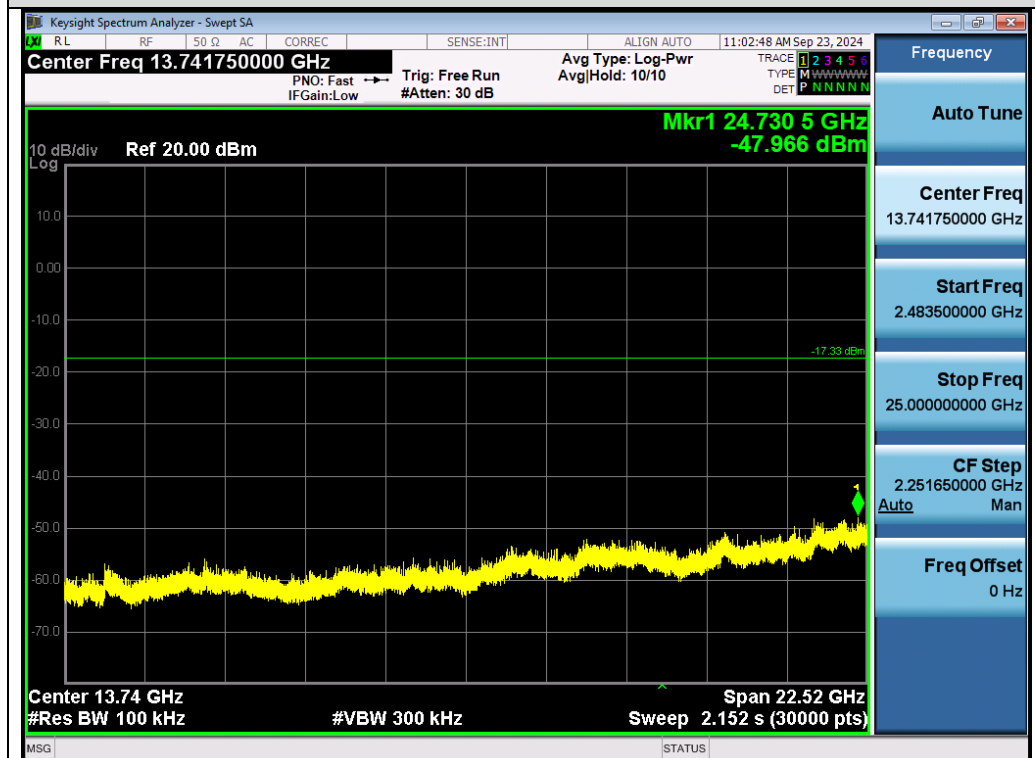
Test_Graph_2.4G_ANT1_2441.85_Higher Band Emissions
