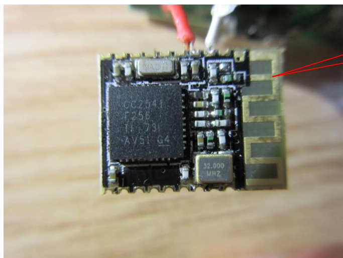
Bluetooth antenna
