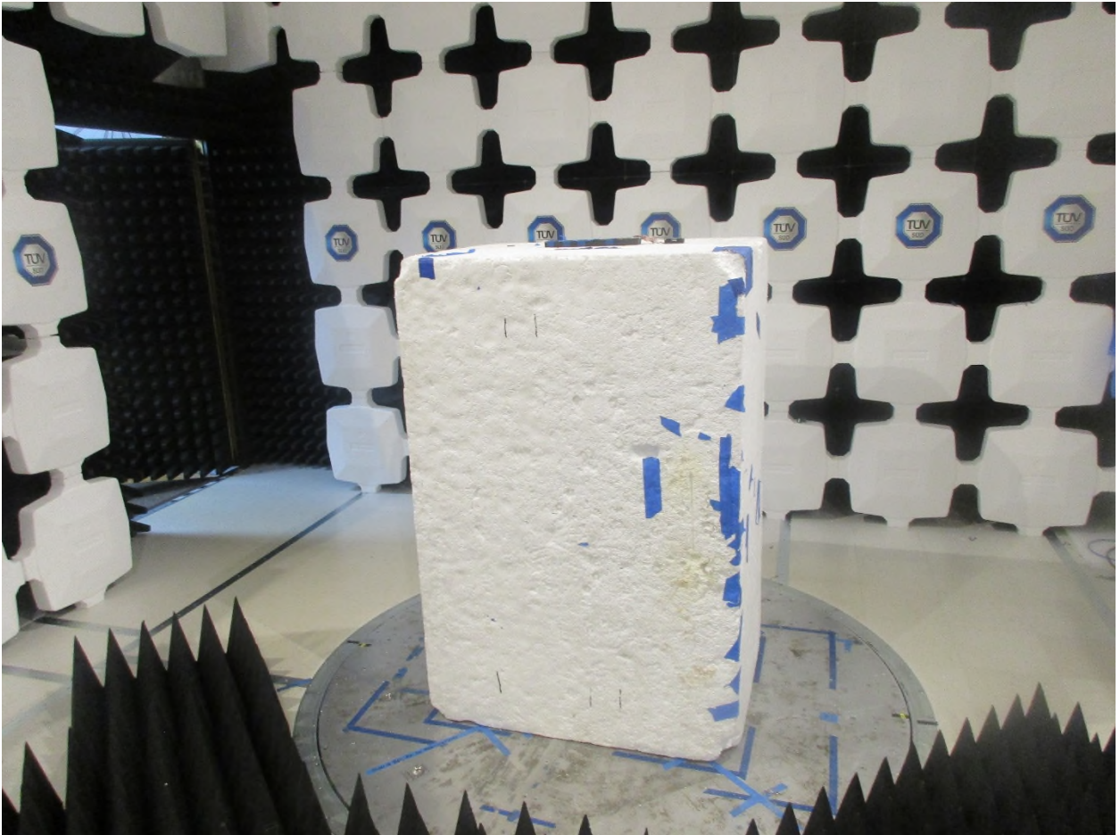
Figure 17: Radiated Emissions – Front View – External Flag Antenna
