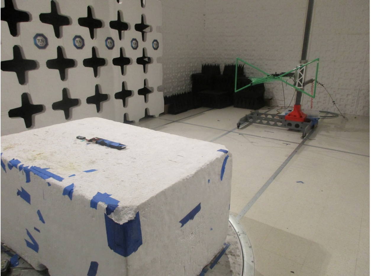
Figure 16: Radiated Emissions – Back V View – External Flag Antenna
