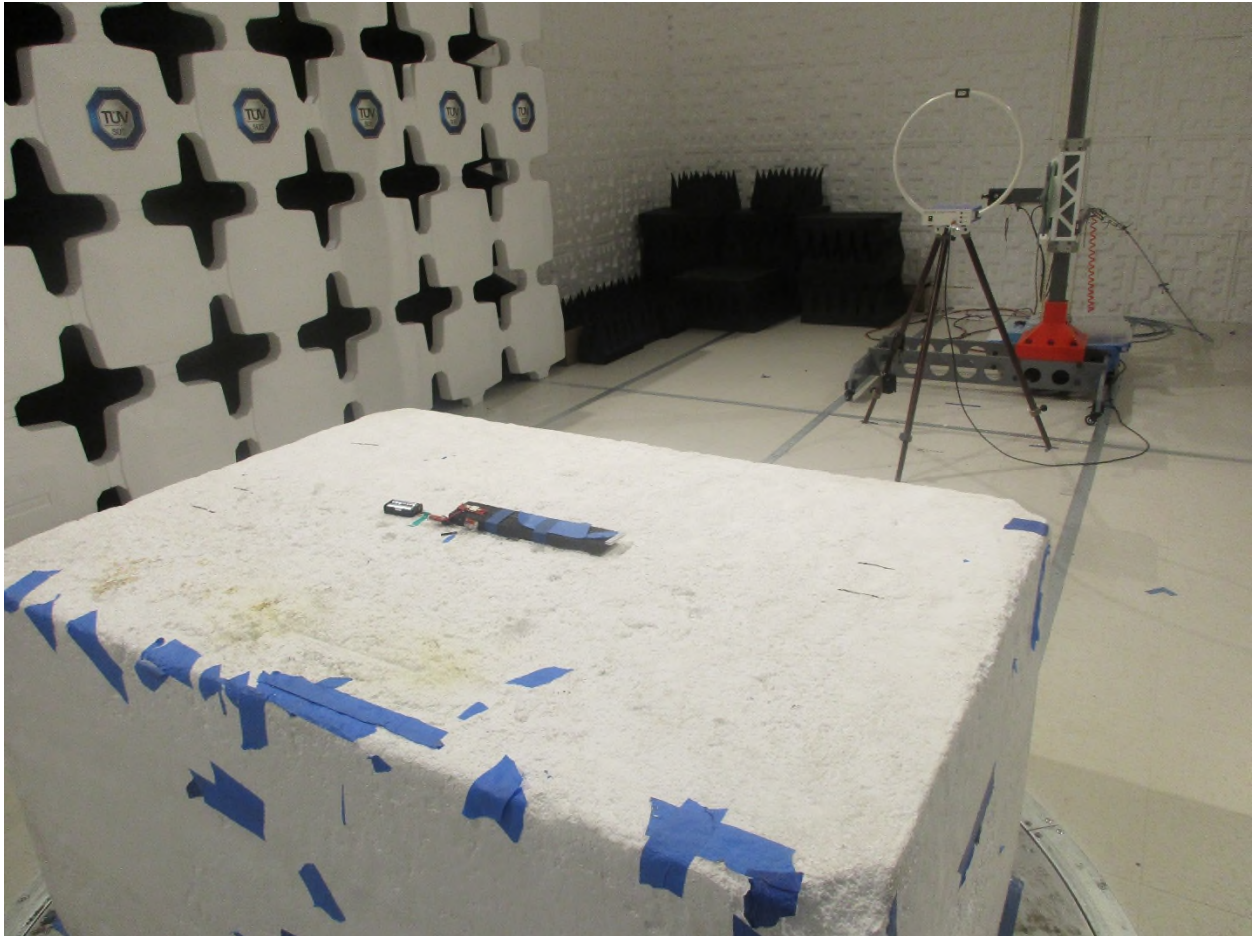
Figure 15: Radiated Emissions – Back View – External Flag Antenna
