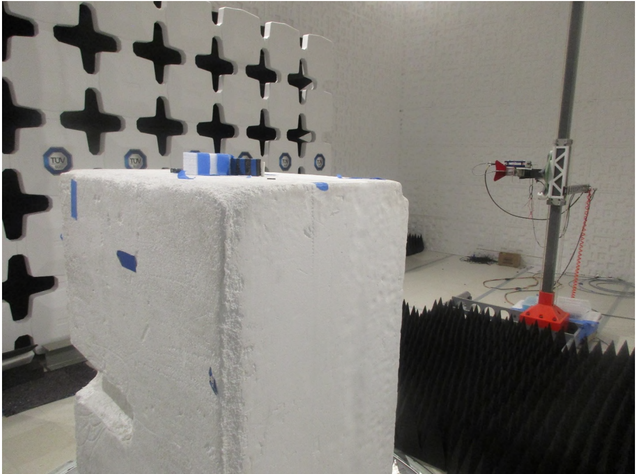
Figure 12: Radiated Emissions – Back View – External Flag Antenna
