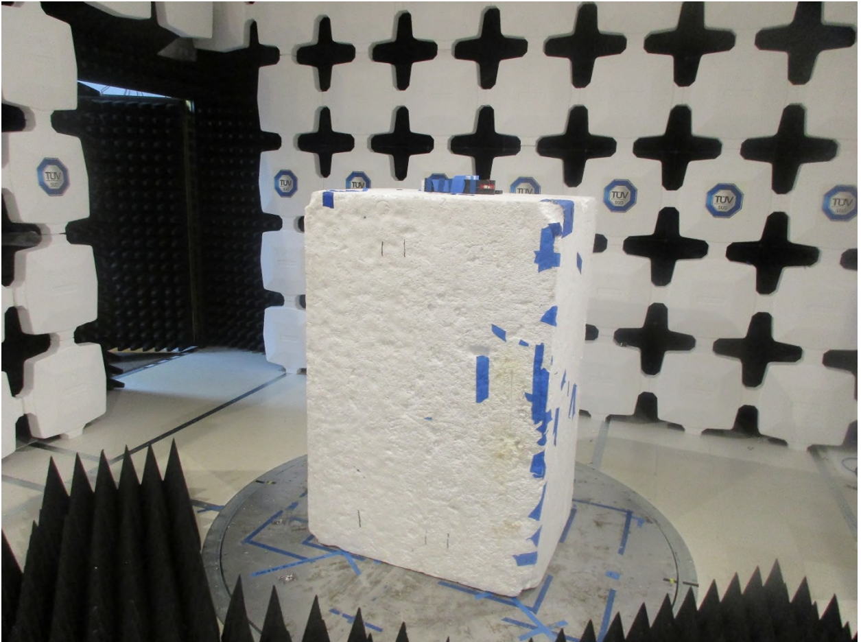
Figure 11: Radiated Emissions – Front View – External Flag Antenna
