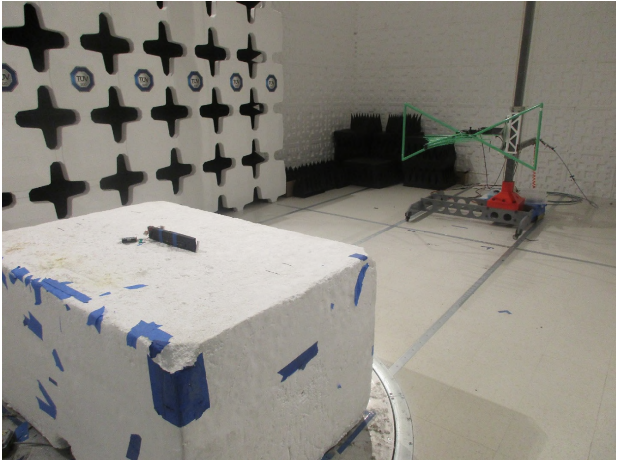
Figure 10: Radiated Emissions – Back View – External Flag Antenna
