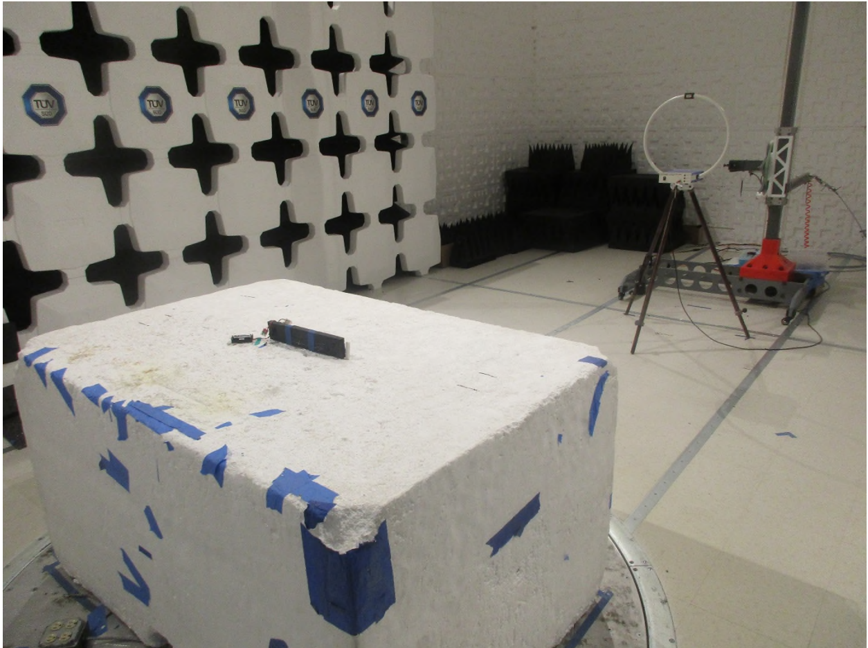
Figure 9: Radiated Emissions – Back View – External Flag Antenna
