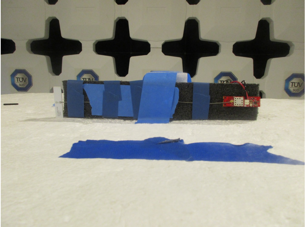
Figure 7: Radiated Emissions – Front View – External Flag Antenna
