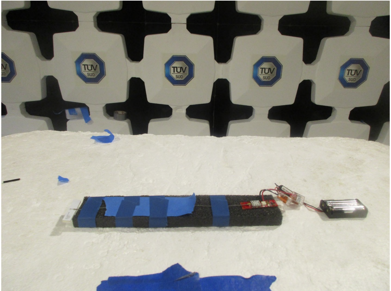
Figure 13: Radiated Emissions – Front View – External Flag Antenna
