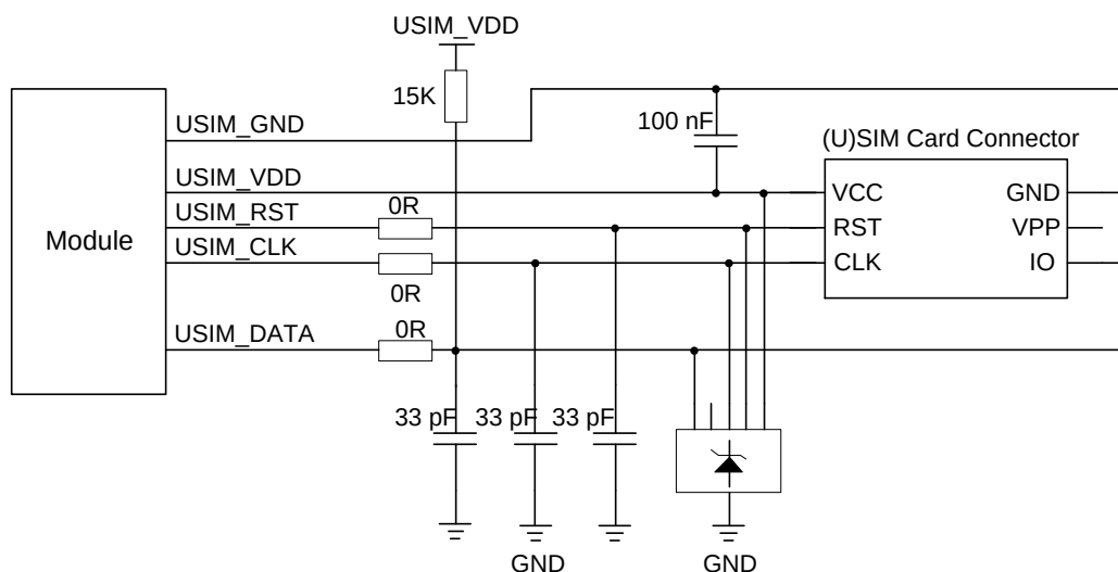
If (U)SIM card detection function is not needed, please keep USIM_PRESENCE unconnected. A reference circuit of (U)SIM interface with a 6-pin (U)SIM card connector is illustrated in the following figure.
