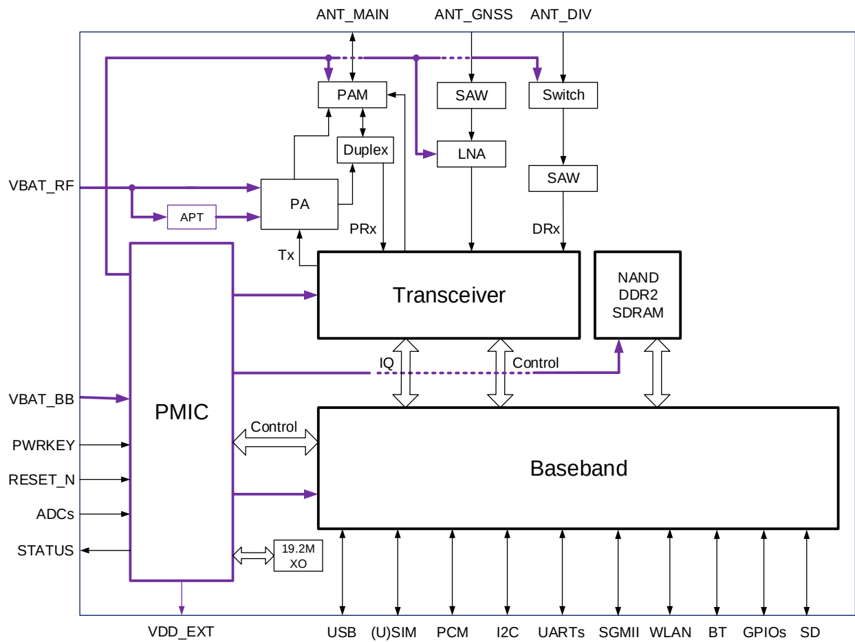
Figure 1: Functional Diagram
