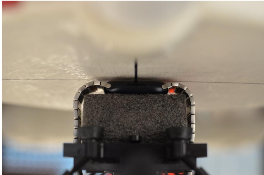
SAR Test Setup Photo 11: Aluminum with Metal Links Wristband, Extremity, Back Side at 0.0 cm
