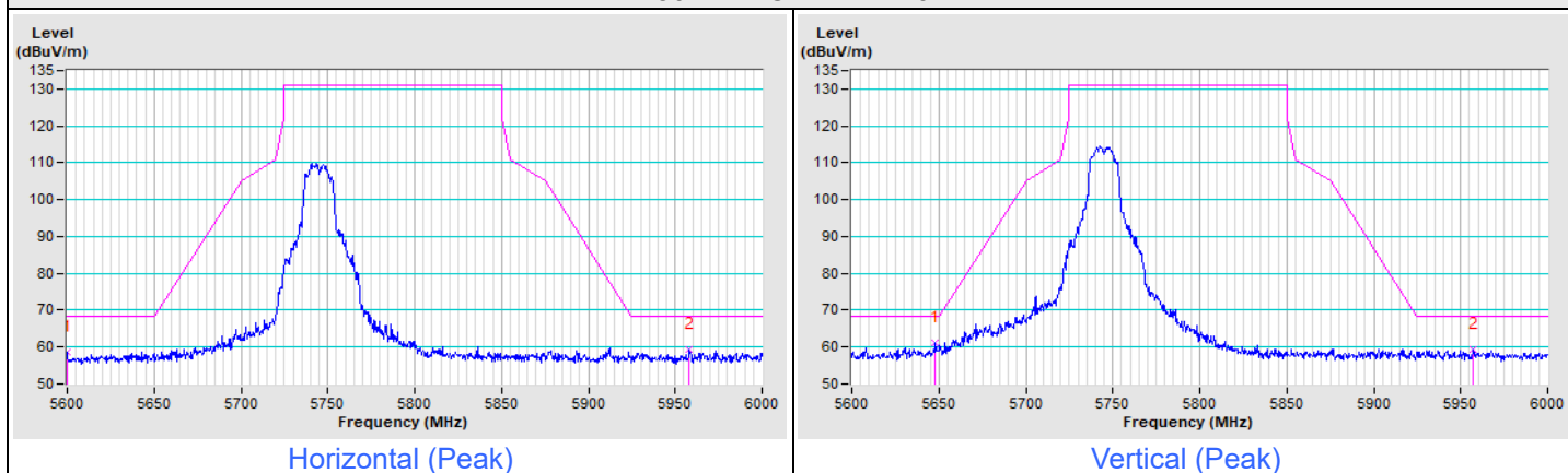
802.11a Channel 149
