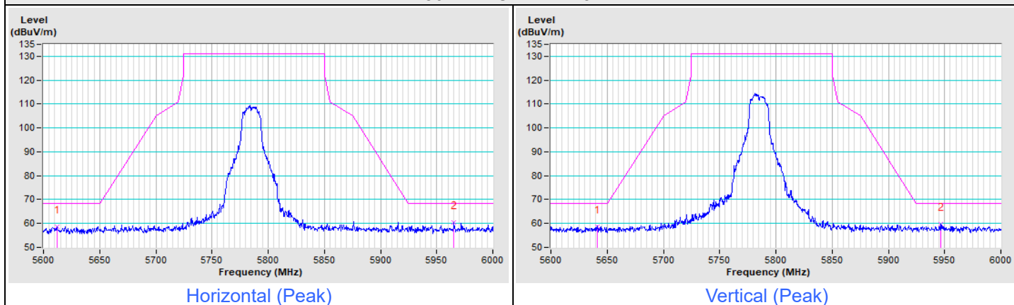
802.11a Channel 157
