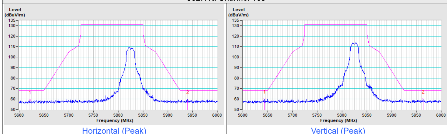
802.11a Channel 165
