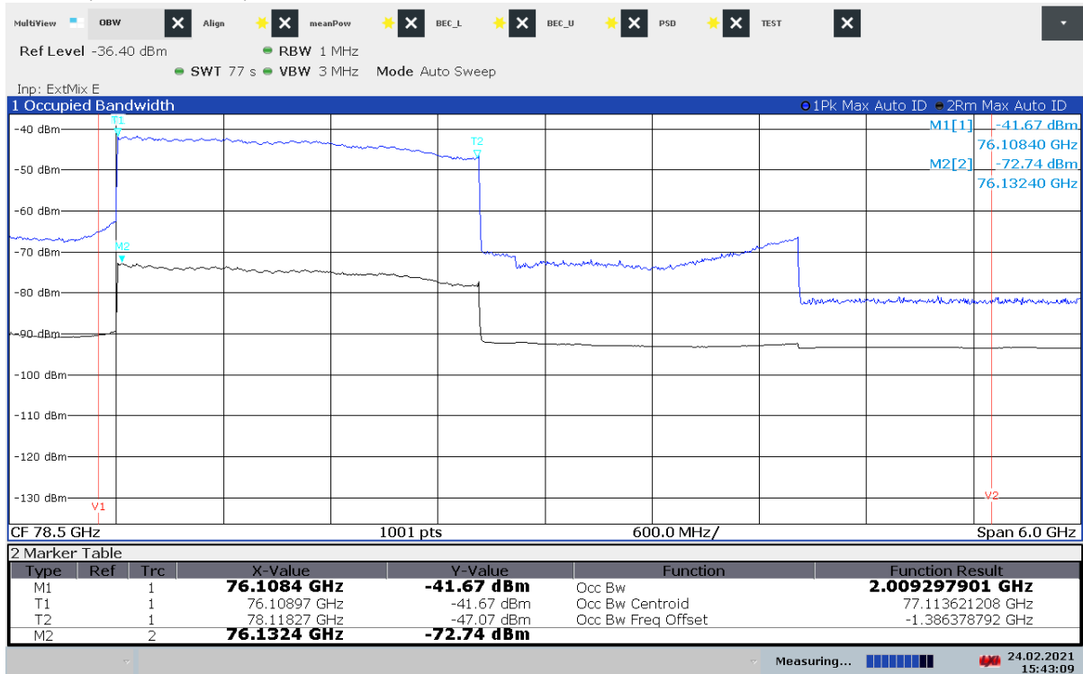
Plot 10: OBW, +10 °C / V_{nom} , Mode 5
