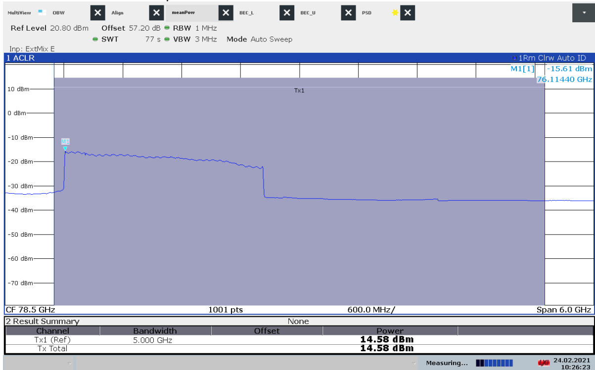
Plot 1: Mode 5 – Radiated mean power
