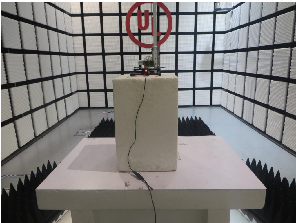
Radiated Disturbance Setup (Above 1 GHz) For 5.8 GHz
