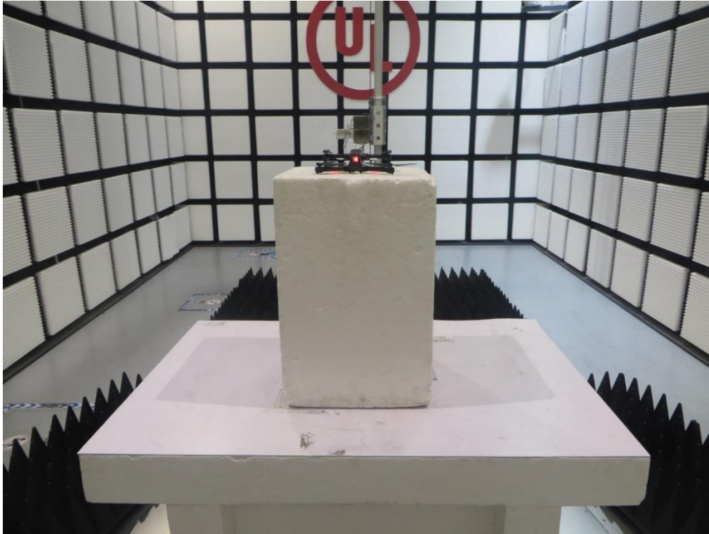
Radiated Disturbance below 1 GHz and above 30 MHz For 5.8 GHz
