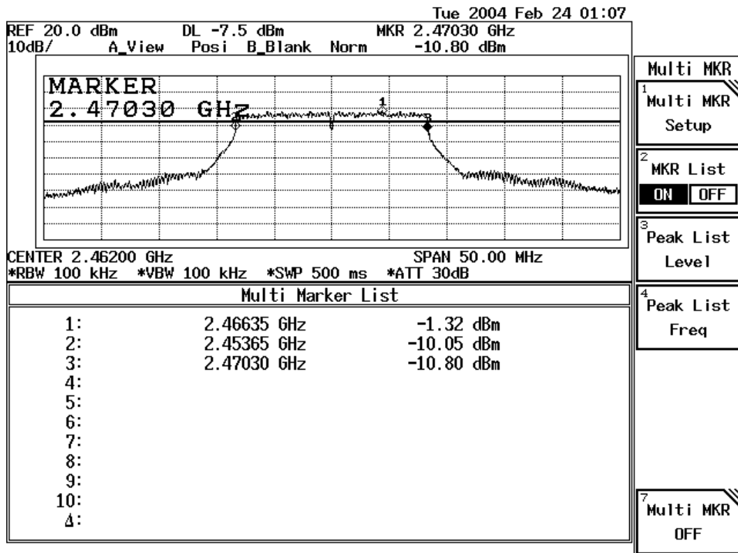
Figure Channel 11: 54Mbps
