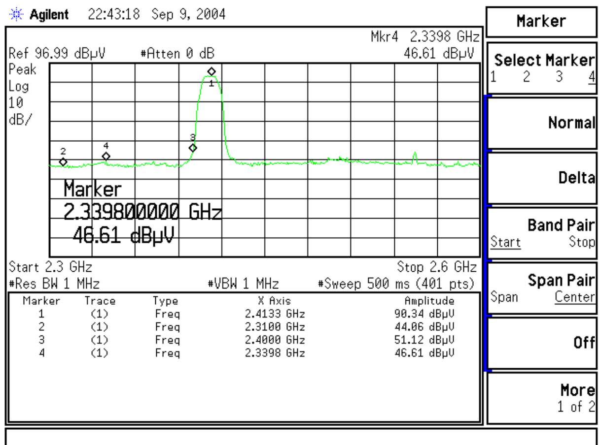
Figure Channel 1: (Horizontal)
