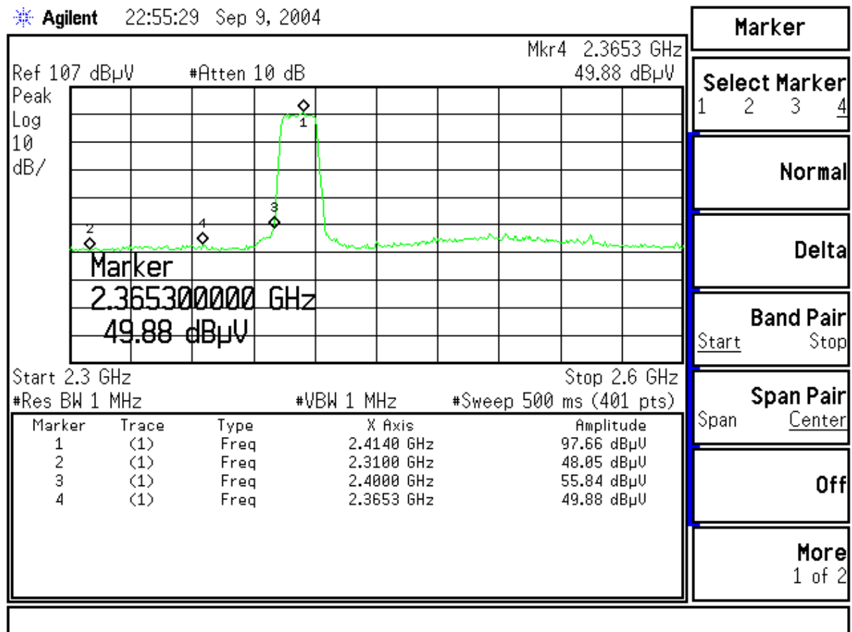
Figure Channel 1: (Vertical)
