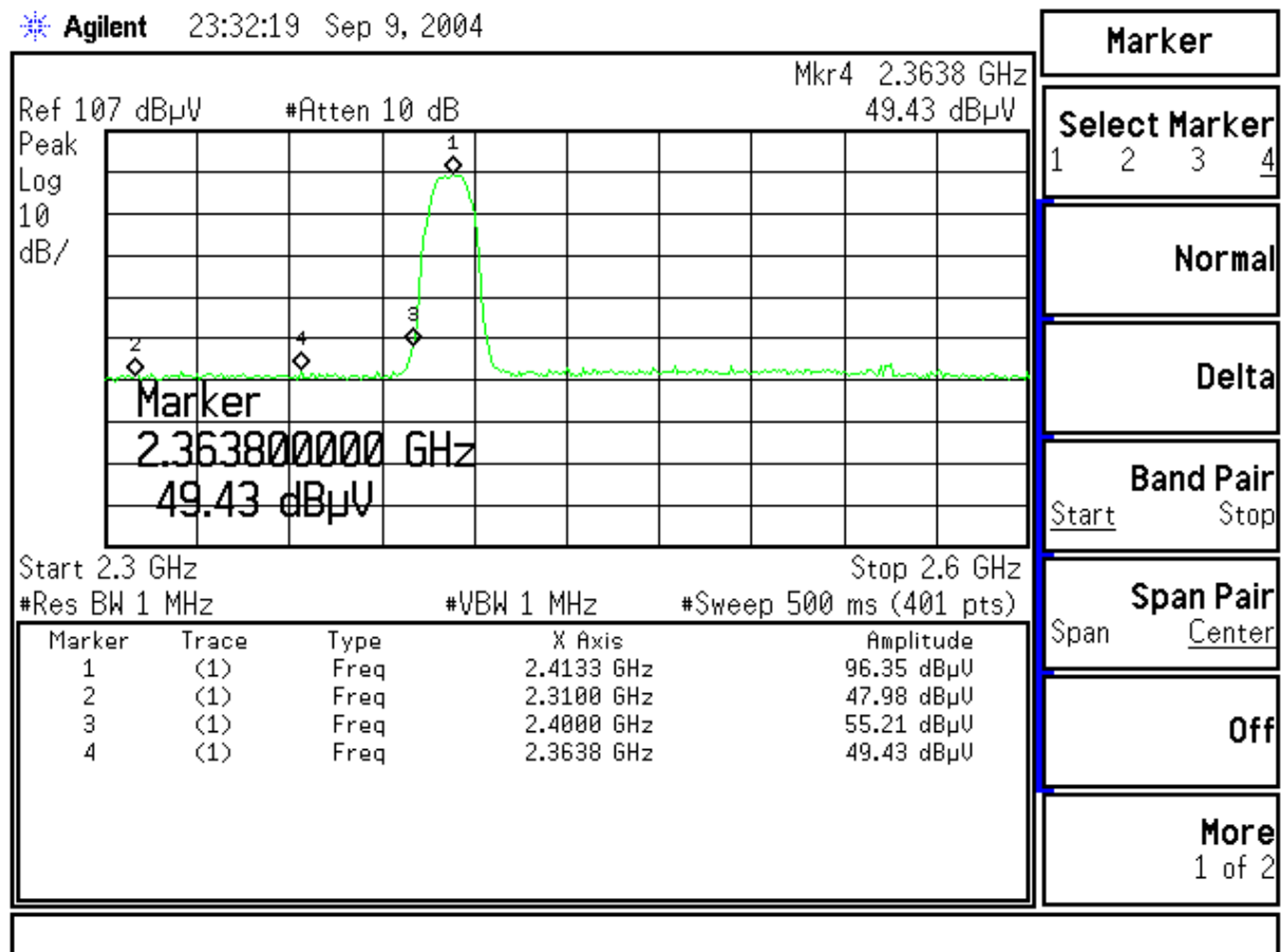
Figure Channel 1: (Horizontal)
