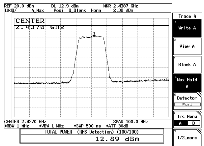
54Mbps-Ch06
