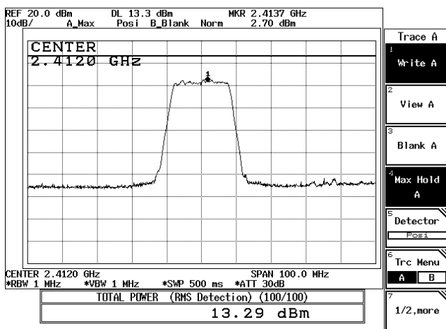
54Mbps-Ch01
