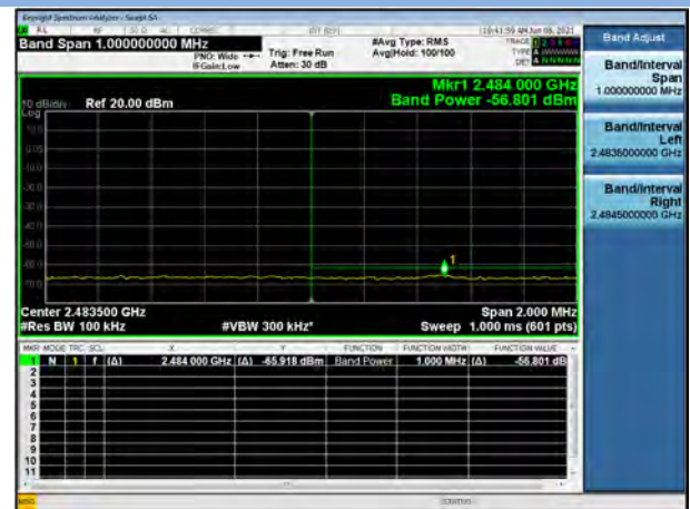
802.11b HIGH CHANNEL, Reference level
