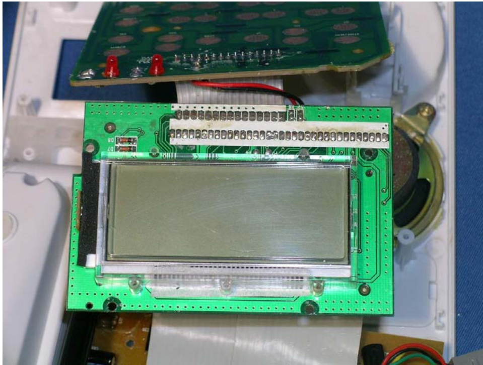
Base LCD display front side
