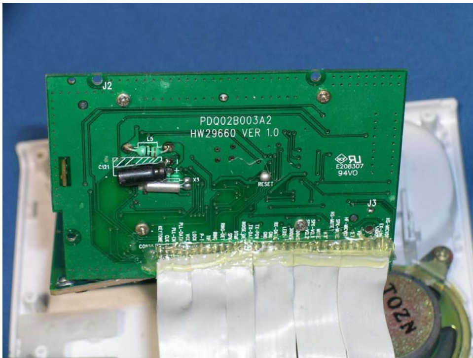
Base LCD display rear side
