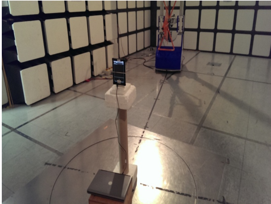
FCC Radiated Emissions 30 MHz to 1 GHz
