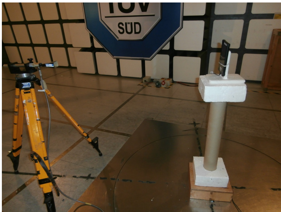
FCC Radiated Emissions 18 GHz to 40 GHz
