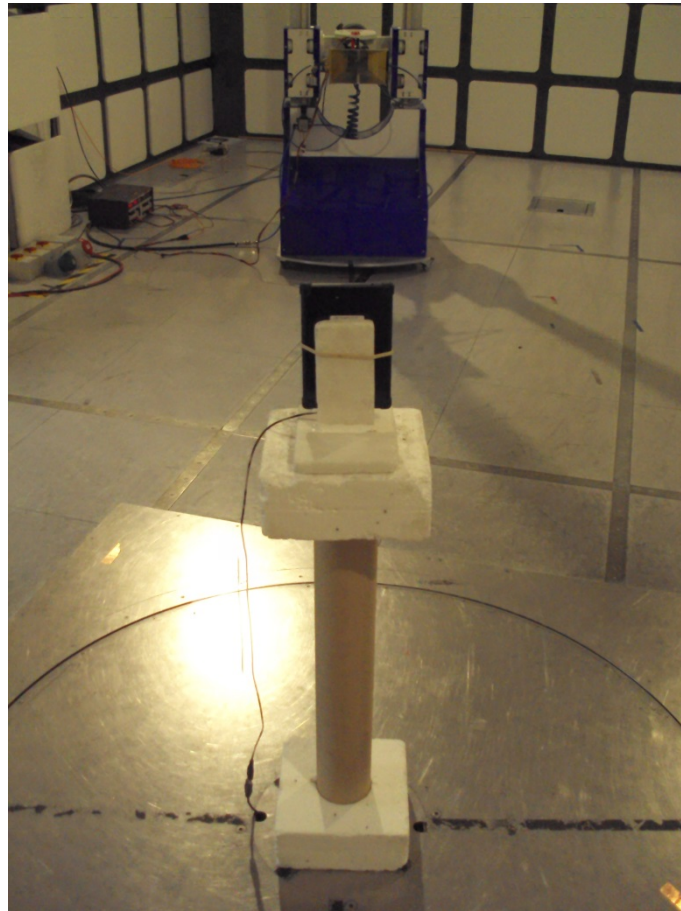
FCC Radiated Emissions 1 GHz to 18 GHz
