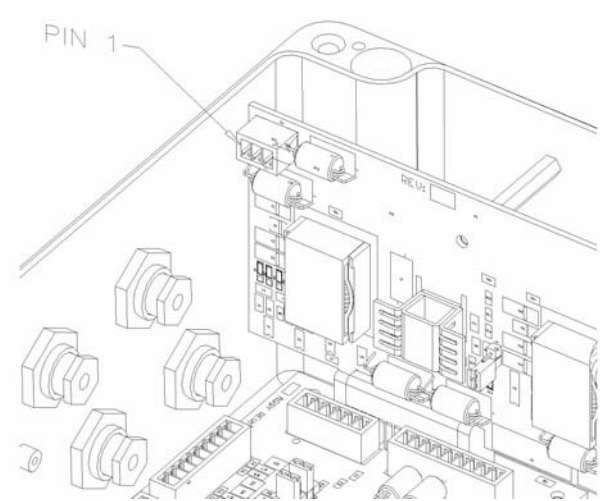
Figure 3-7. Input Power Terminals
