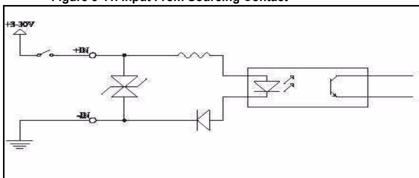
Figure 3-11. Input From Sourcing Contact
