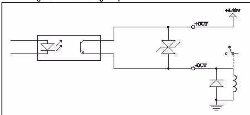
Figure 3-15. Sourcing Output 'Contact'
