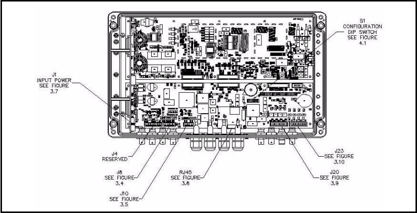
Figure 3-2. Internal Connectors
