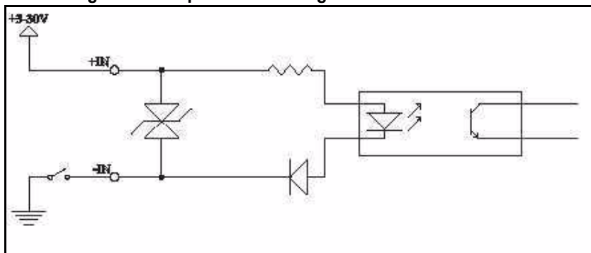
Figure 3-12. Input From Sinking Contact
