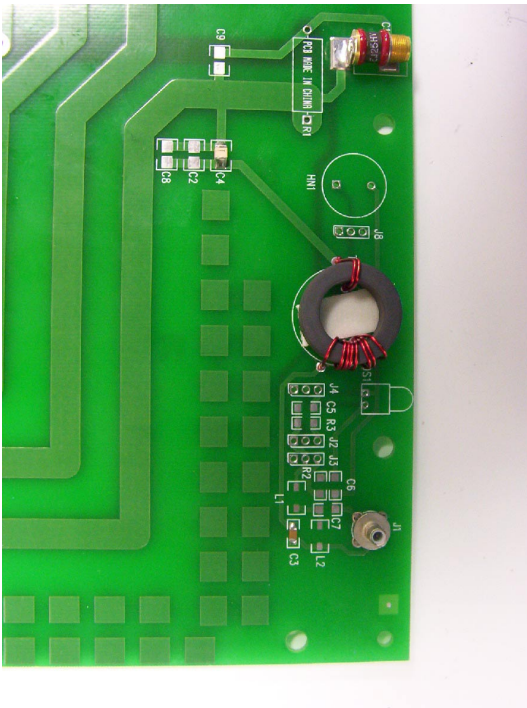
Antenna Component Close-up
