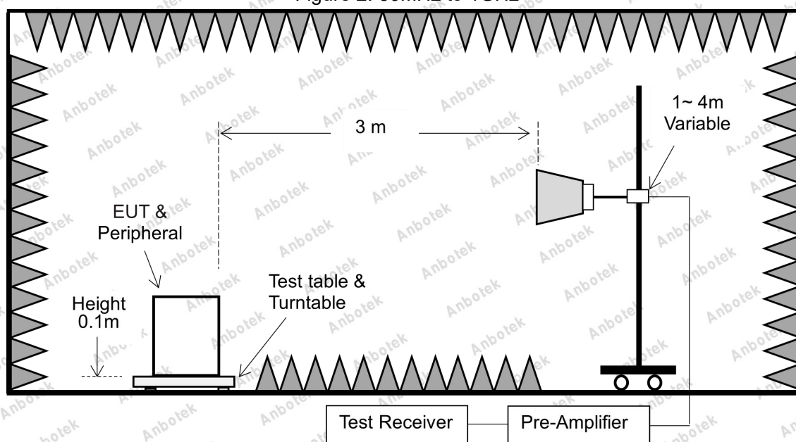
Figure 3. Above 1 GHz
