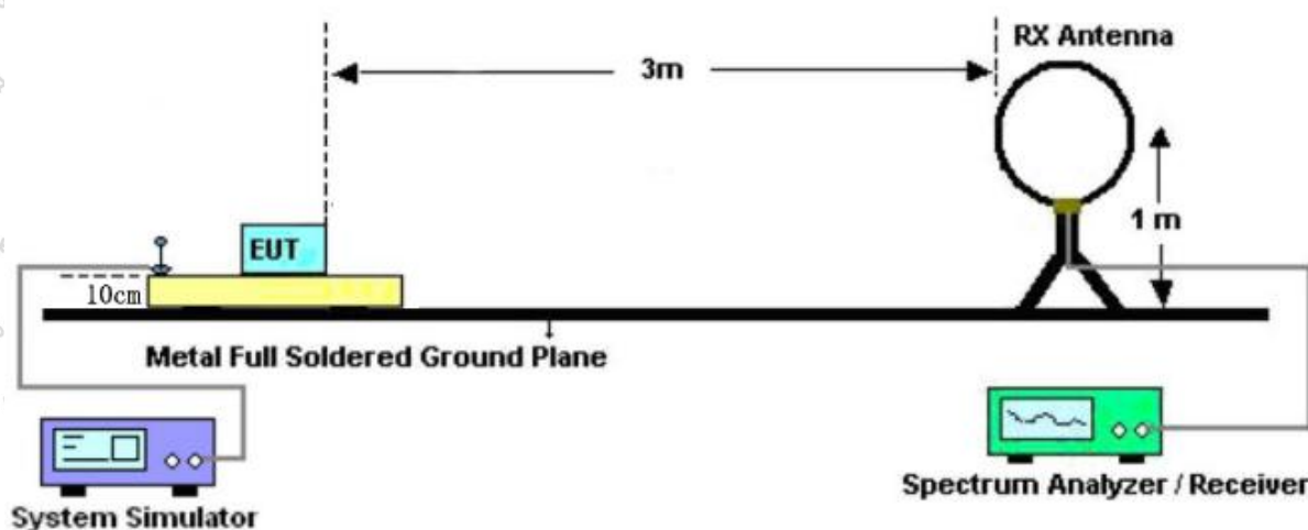
Figure 1. Below 30MHz
